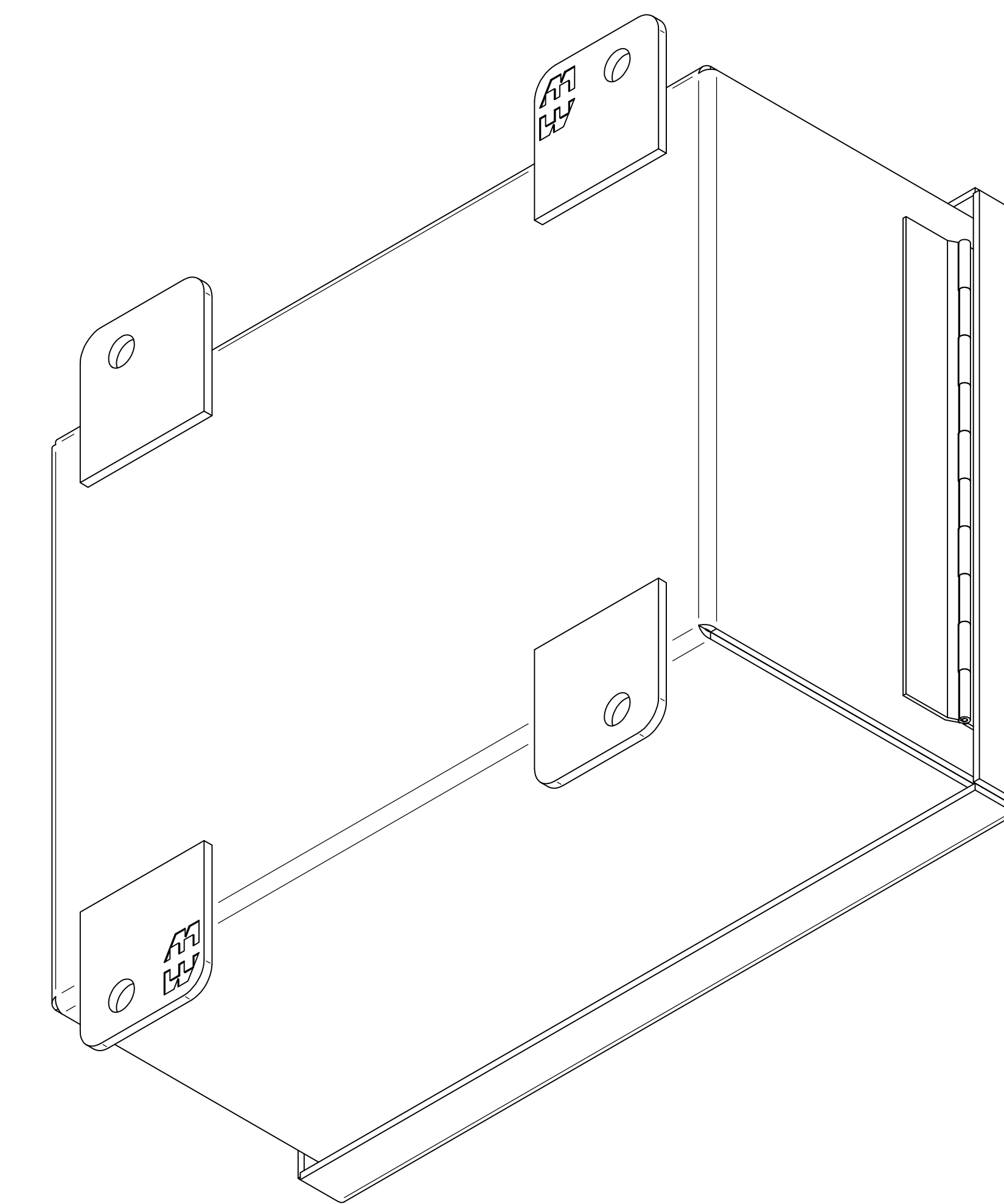
ISOMETRIC VIEWS
