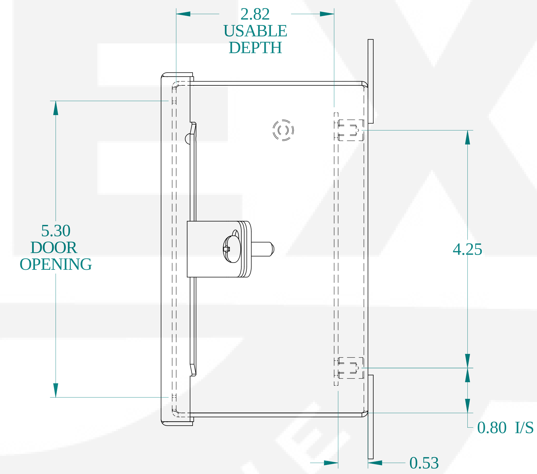
SIDE VIEW
