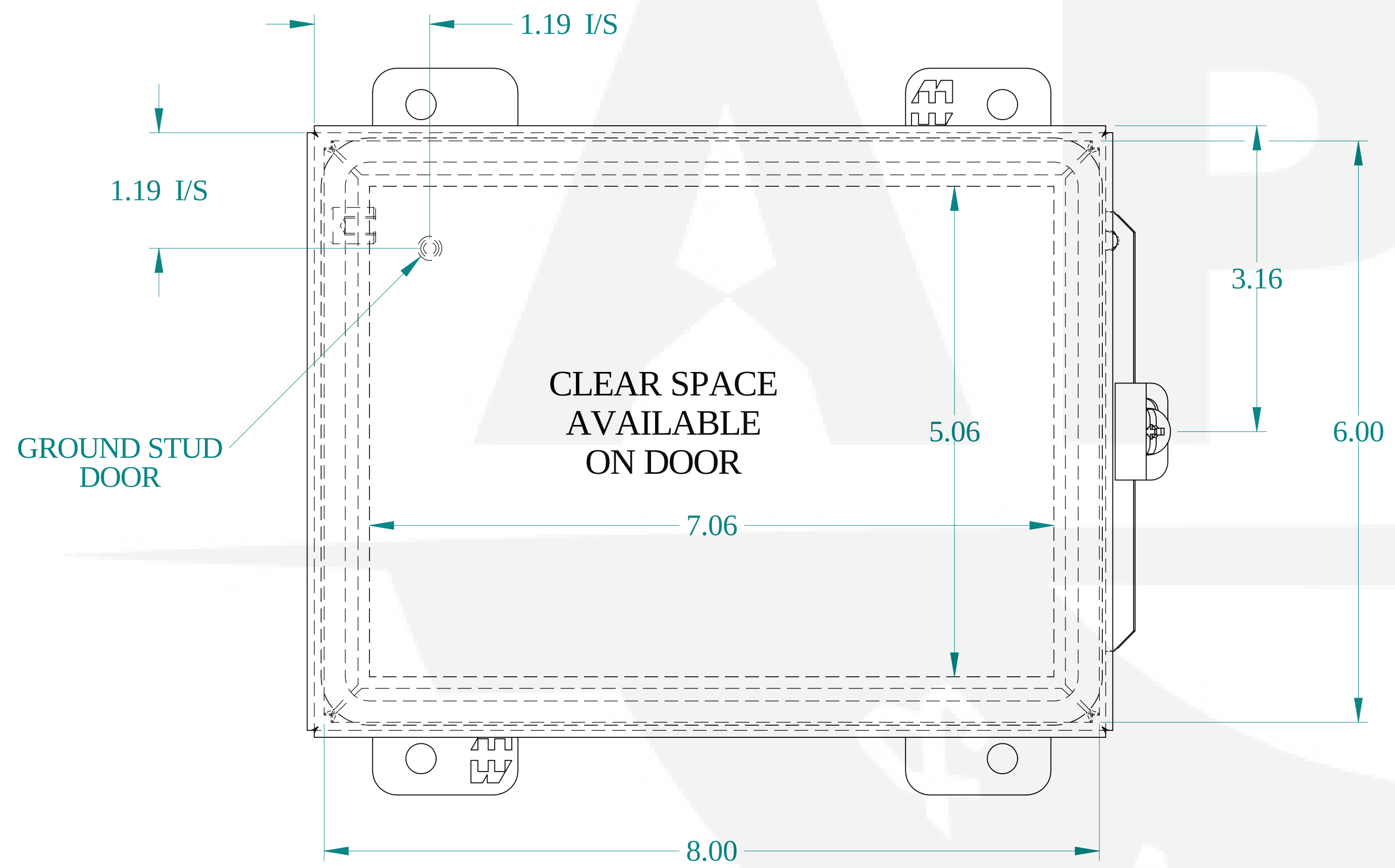
FRONT VIEW
