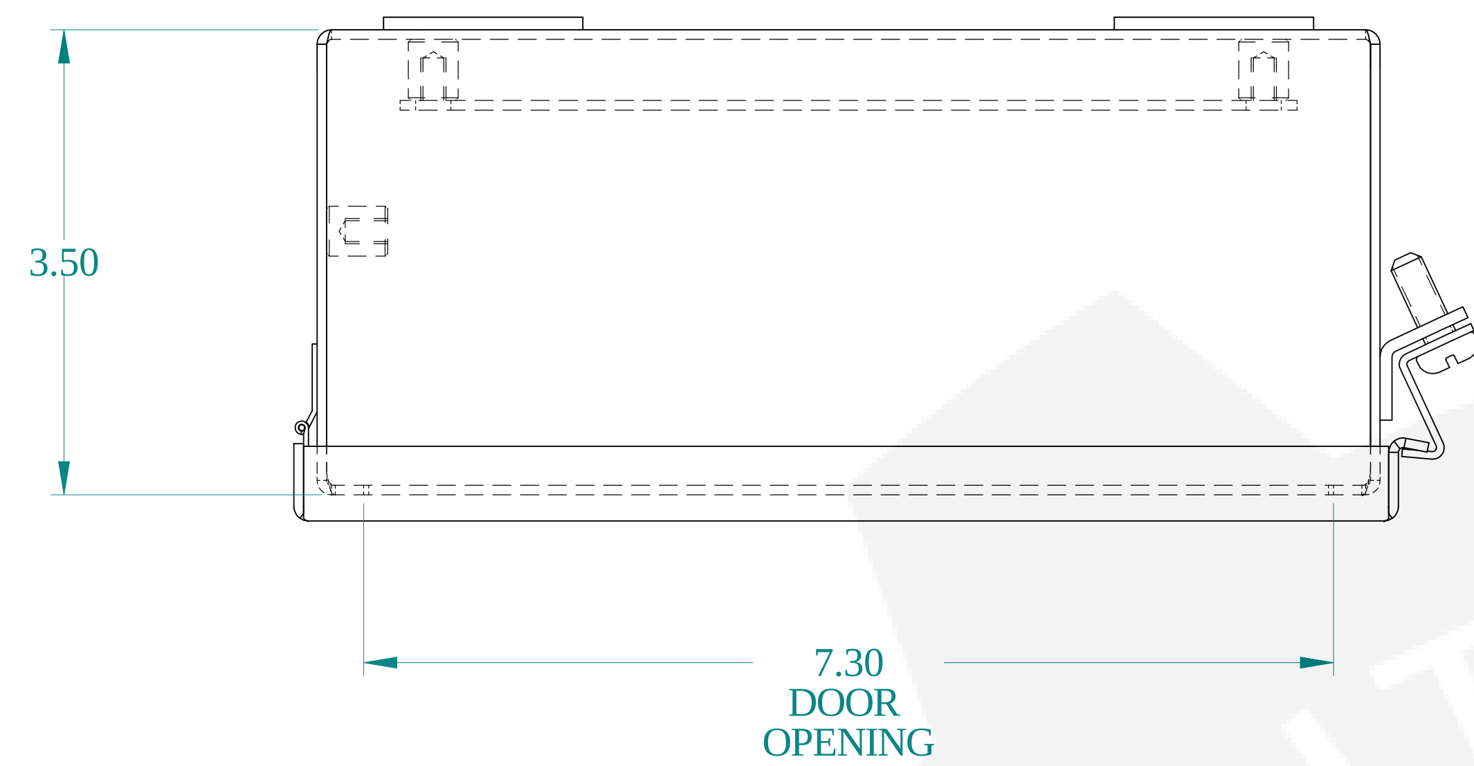
TOP VIEW
