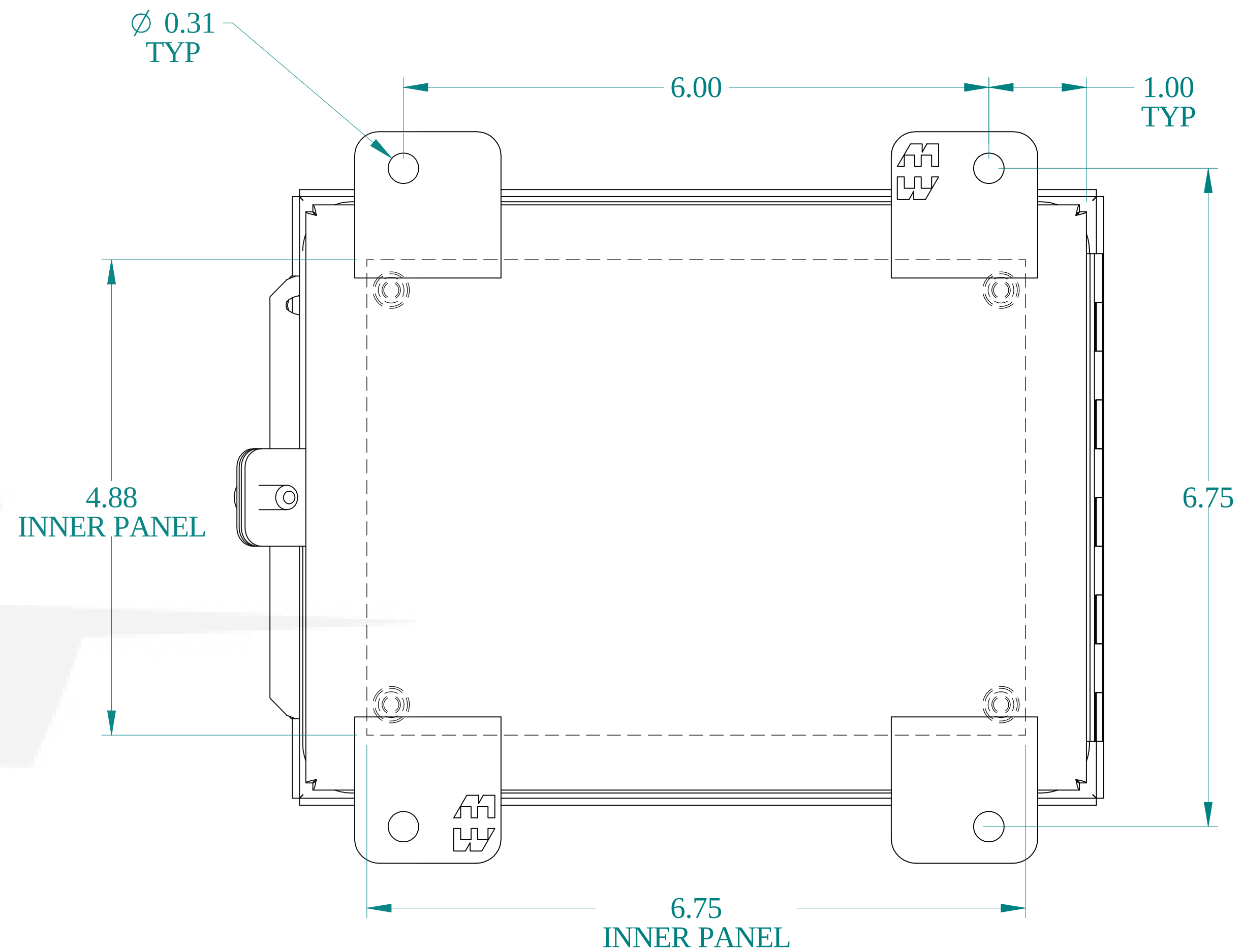
BACK VIEW
