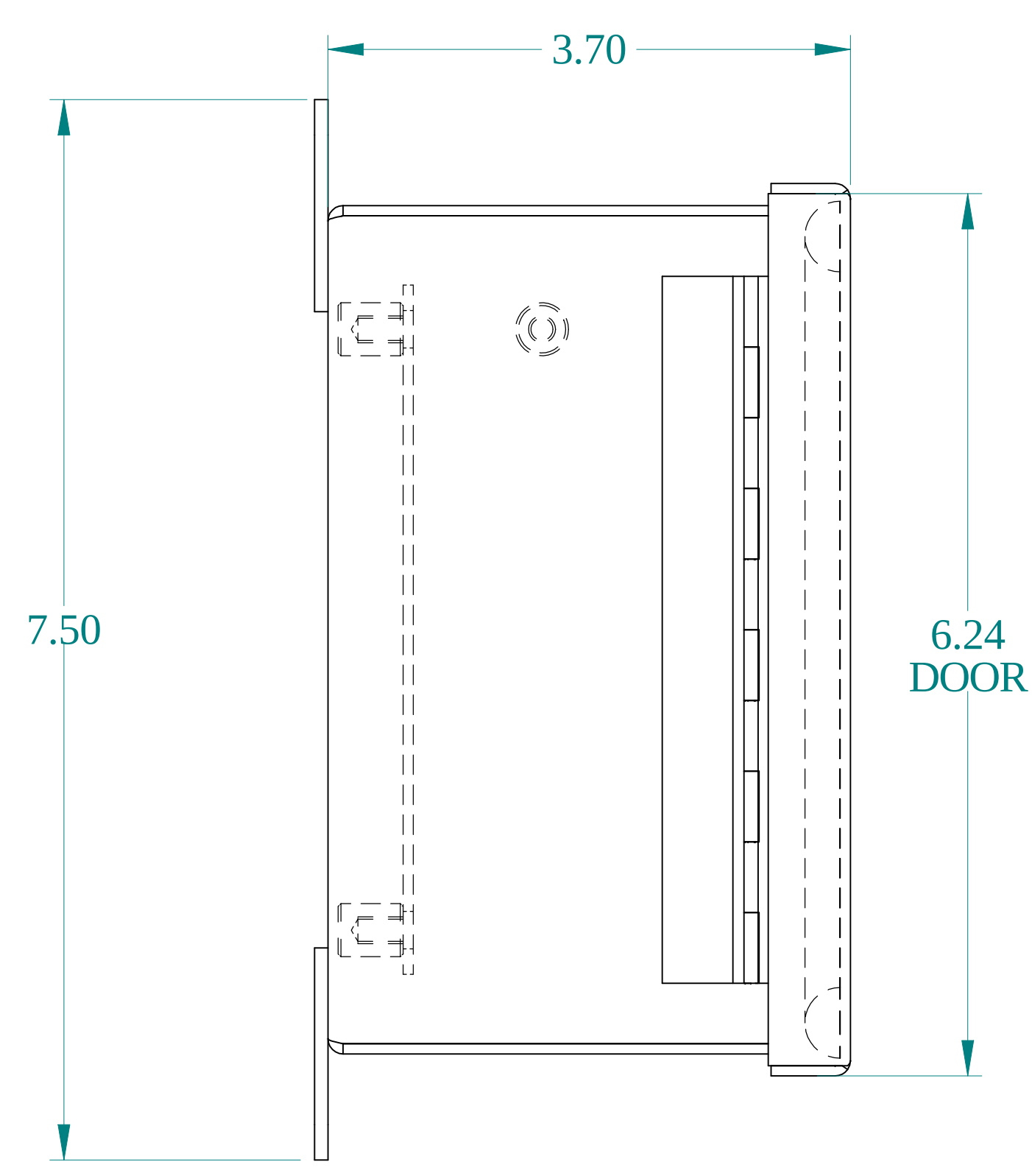
SIDE VIEW
