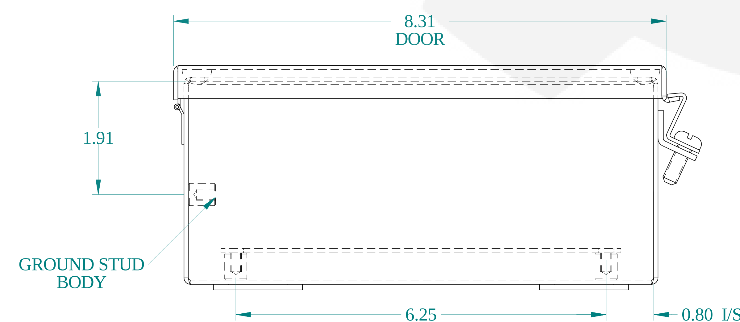
BOTTOM VIEW
