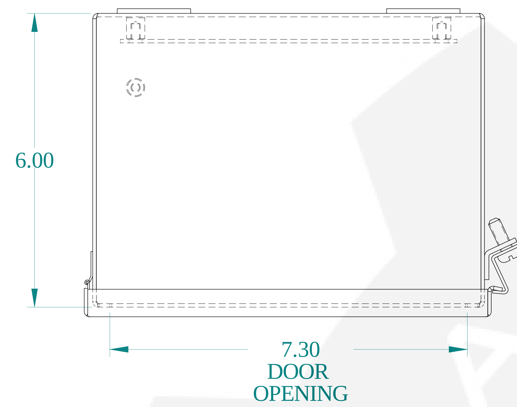
TOP VIEW
