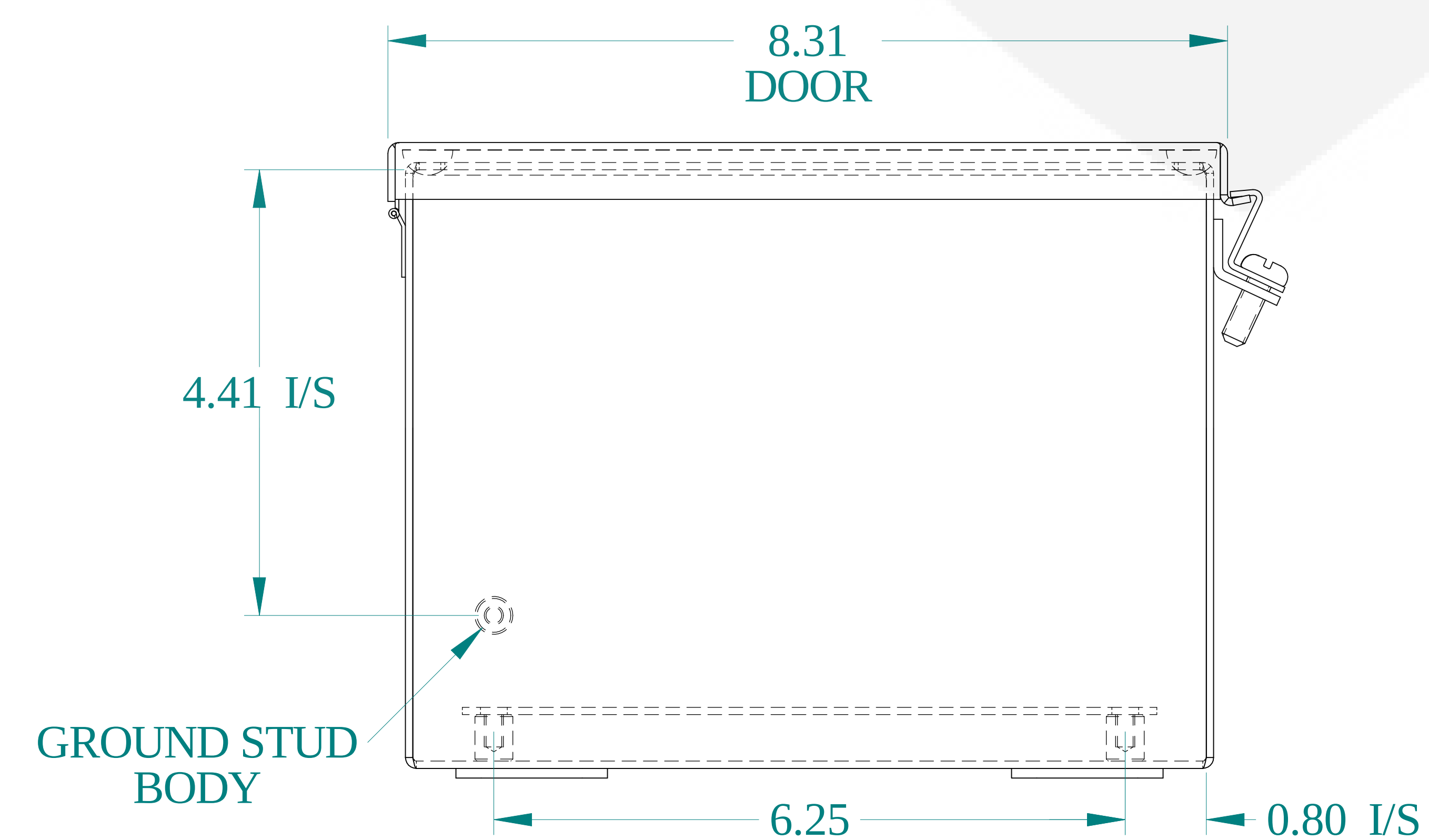
BOTTOM VIEW
