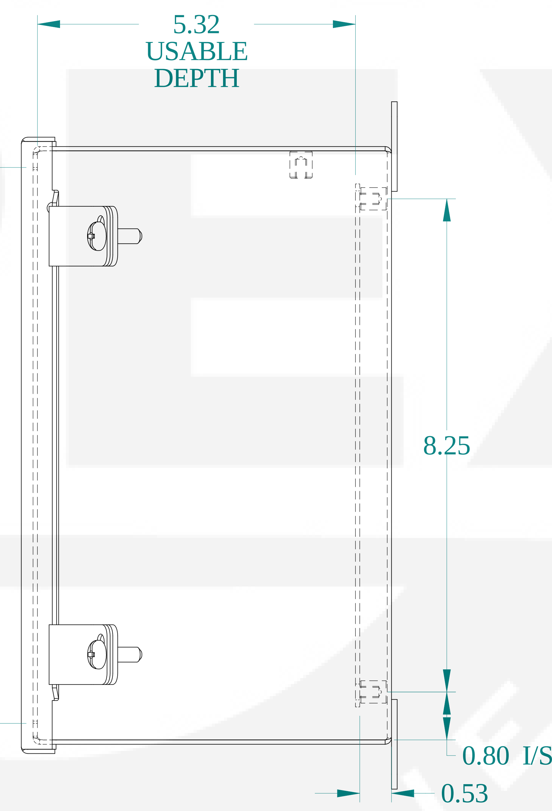
SIDE VIEW
