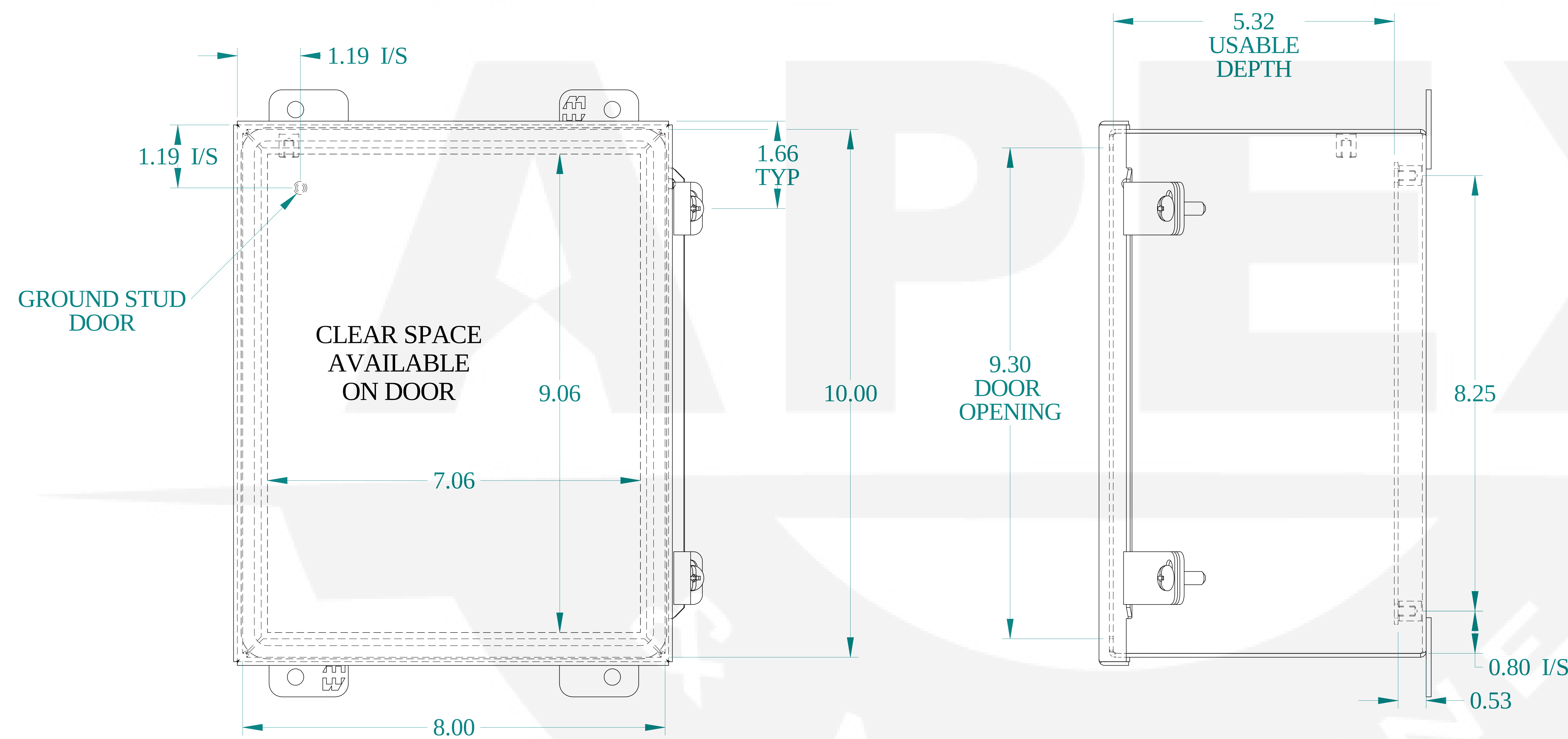
FRONT VIEW
