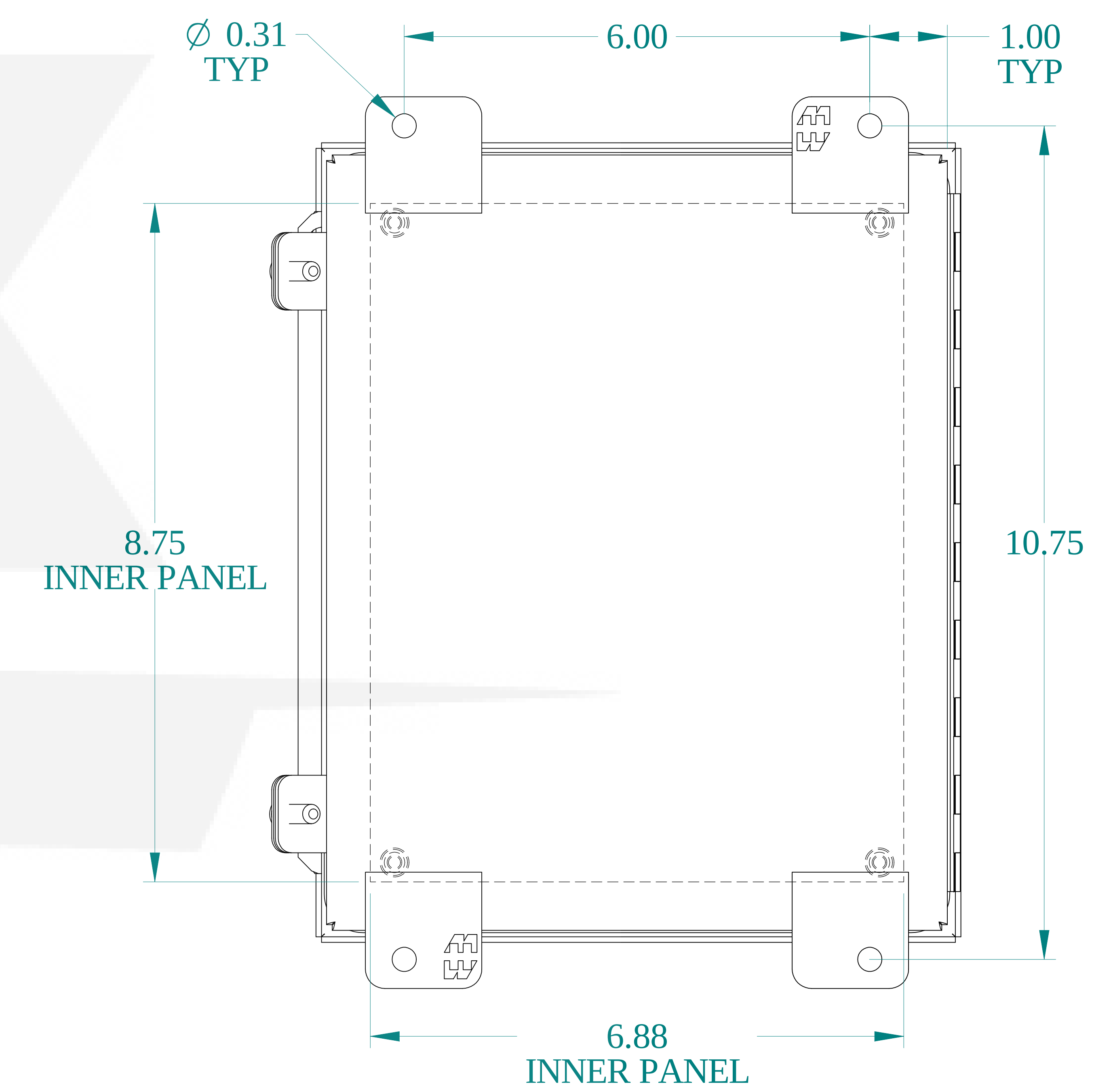
BACK VIEW
