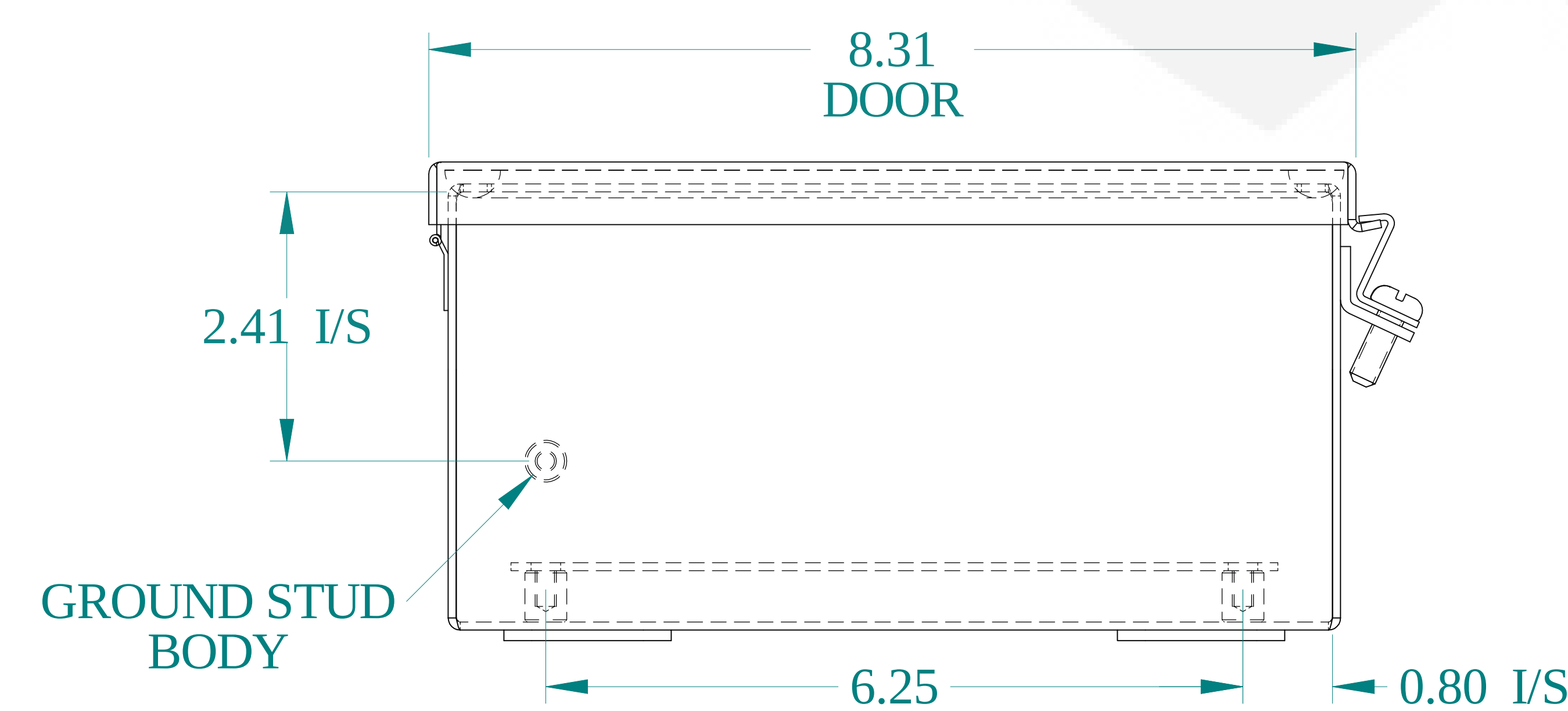
BOTTOM VIEW
