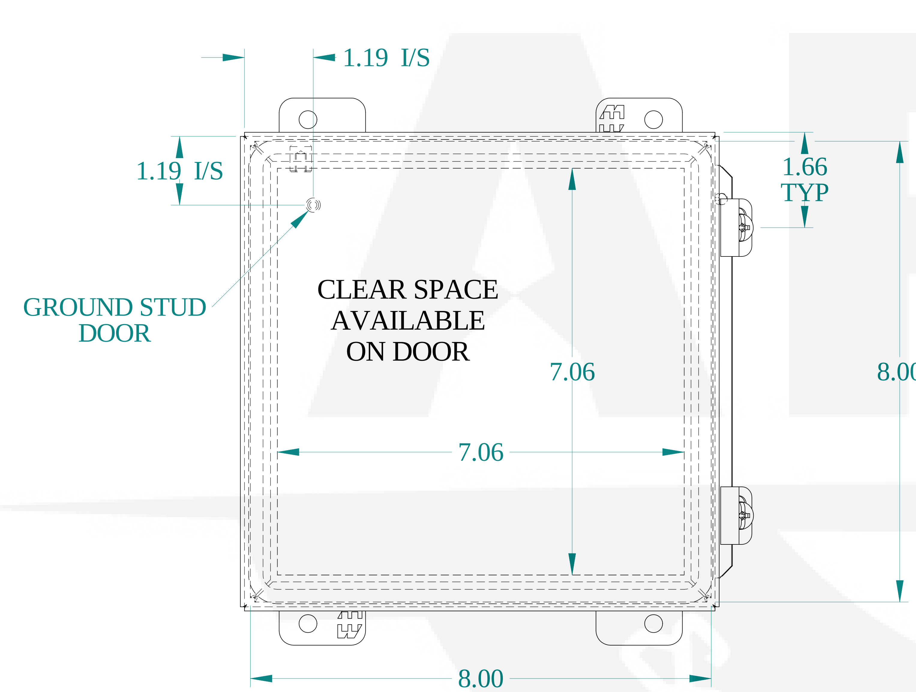
FRONT VIEW
