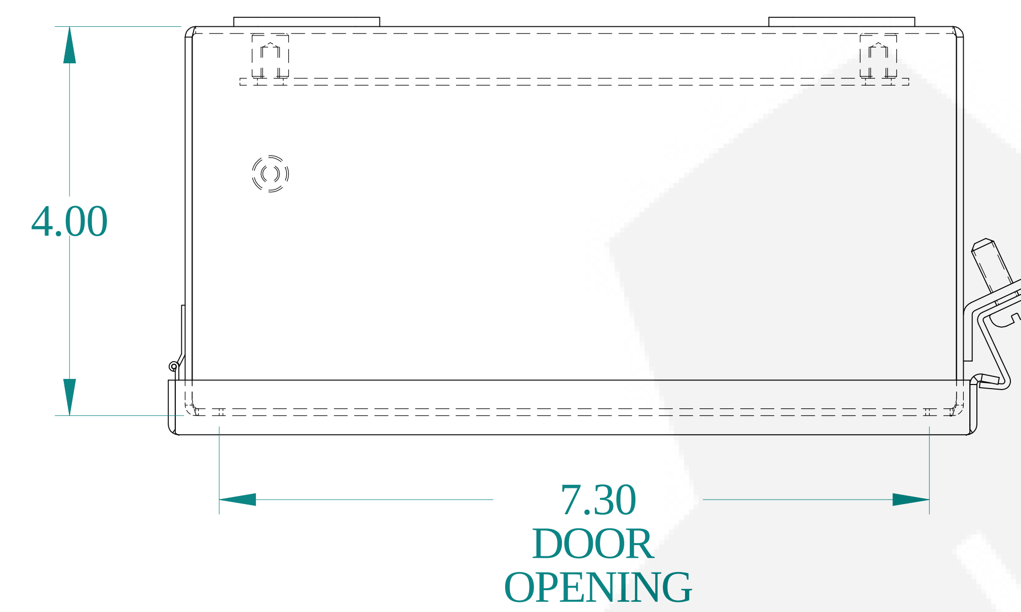
TOP VIEW
