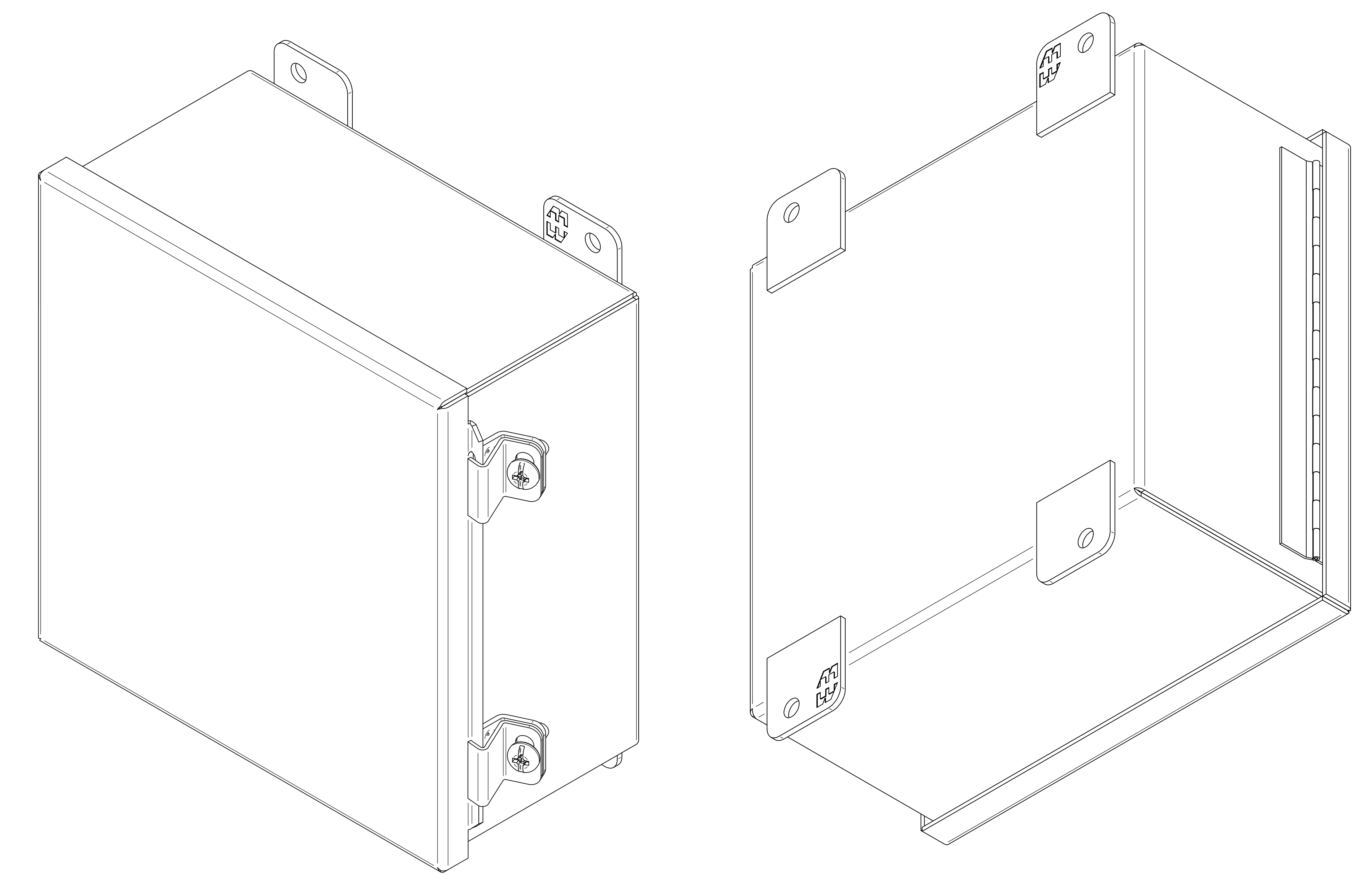
ISOMETRIC VIEWS
