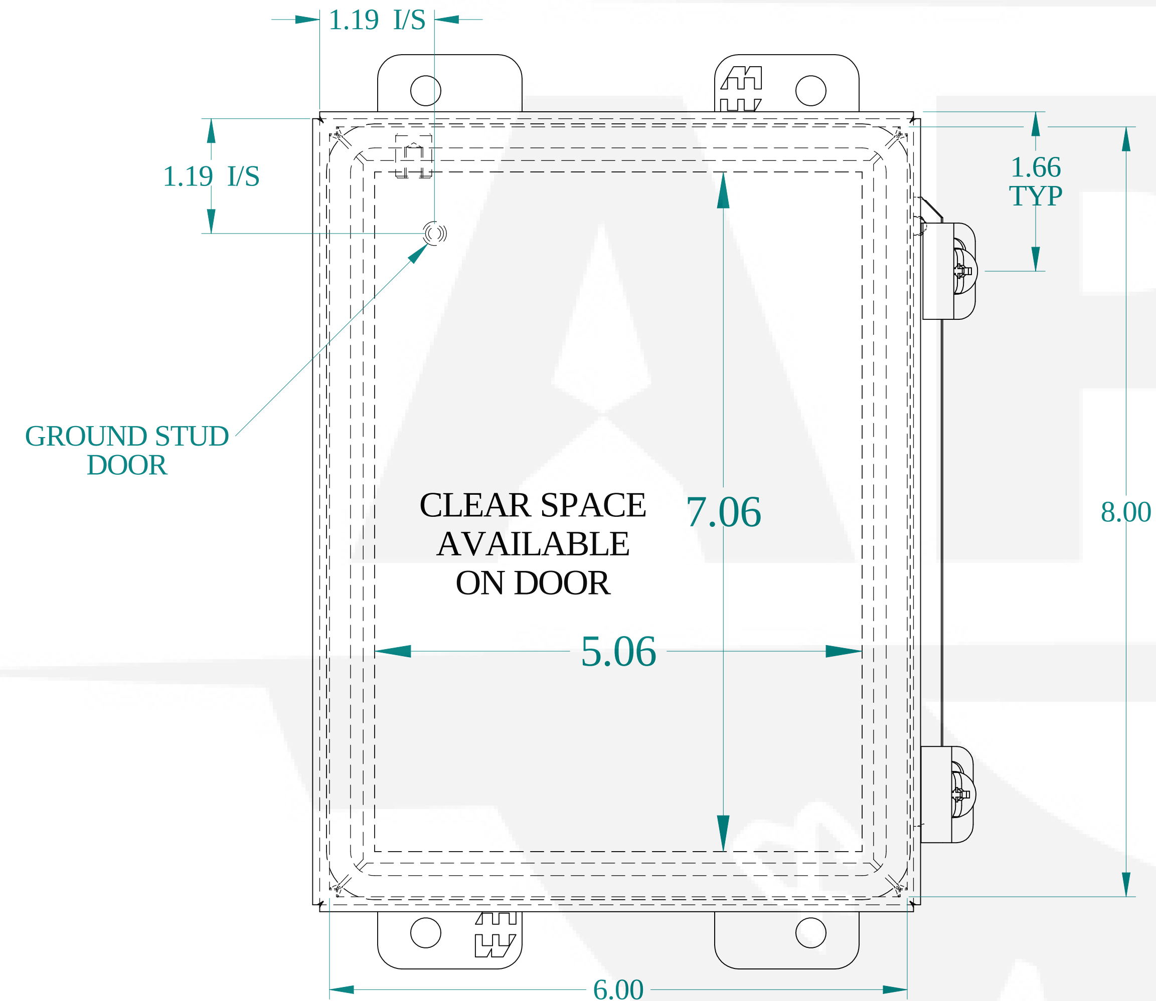
FRONT VIEW
