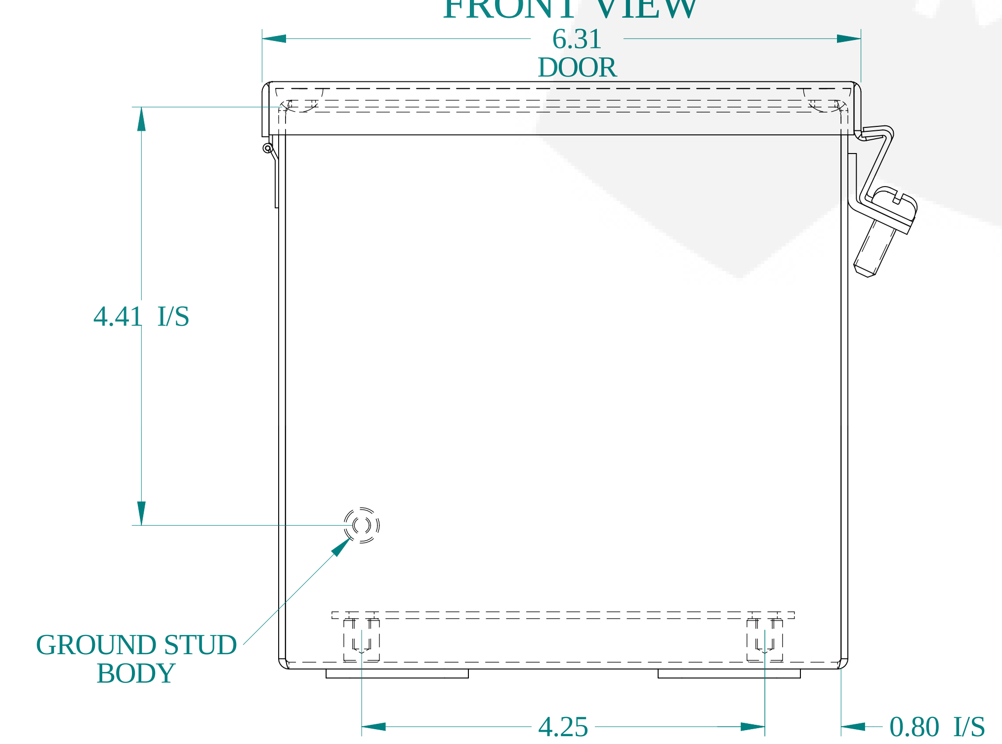
BOTTOM VIEW
