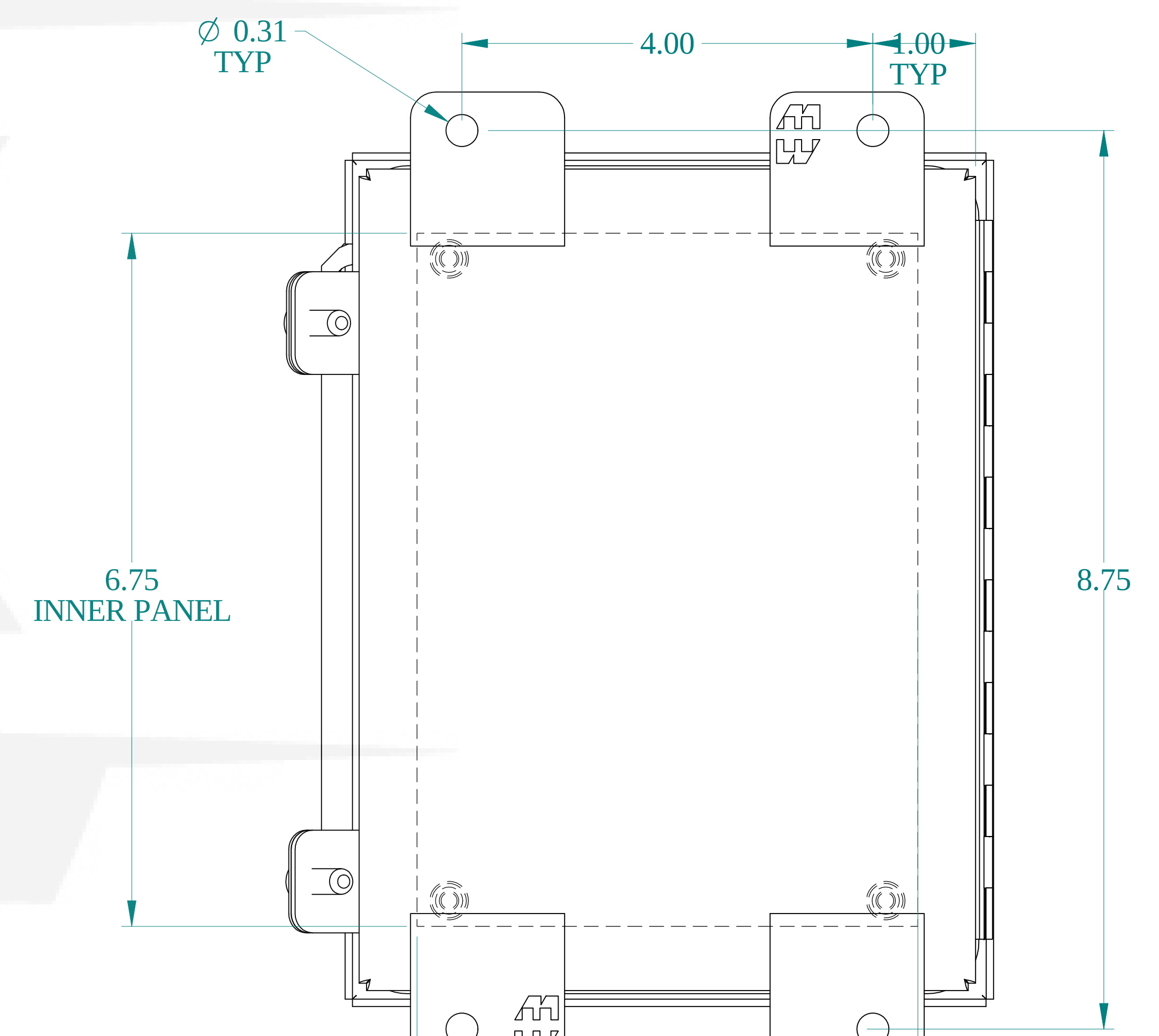
BACK VIEW
