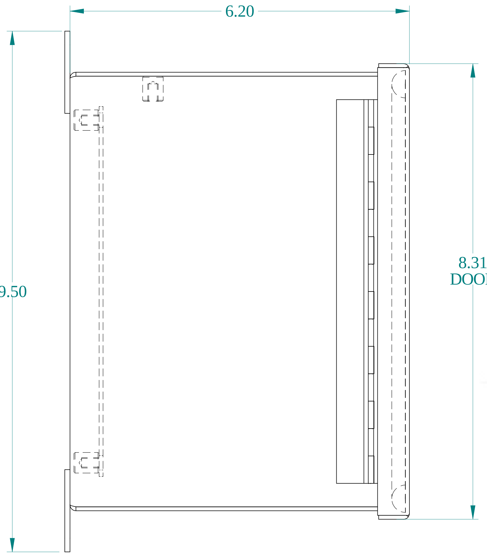
SIDE VIEW
