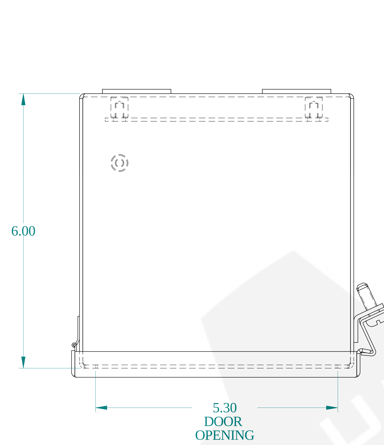
TOP VIEW
