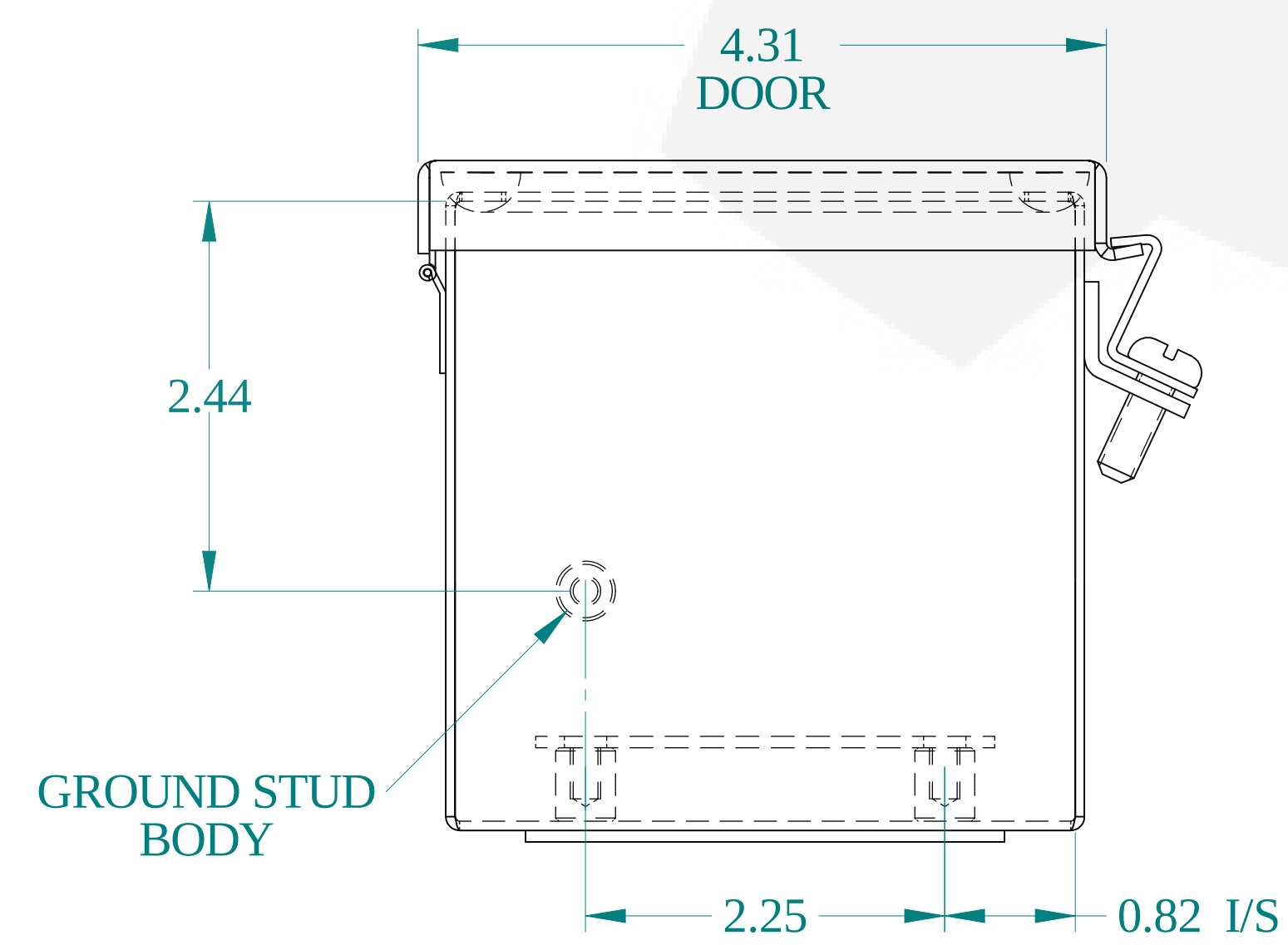
BOTTOM VIEW
