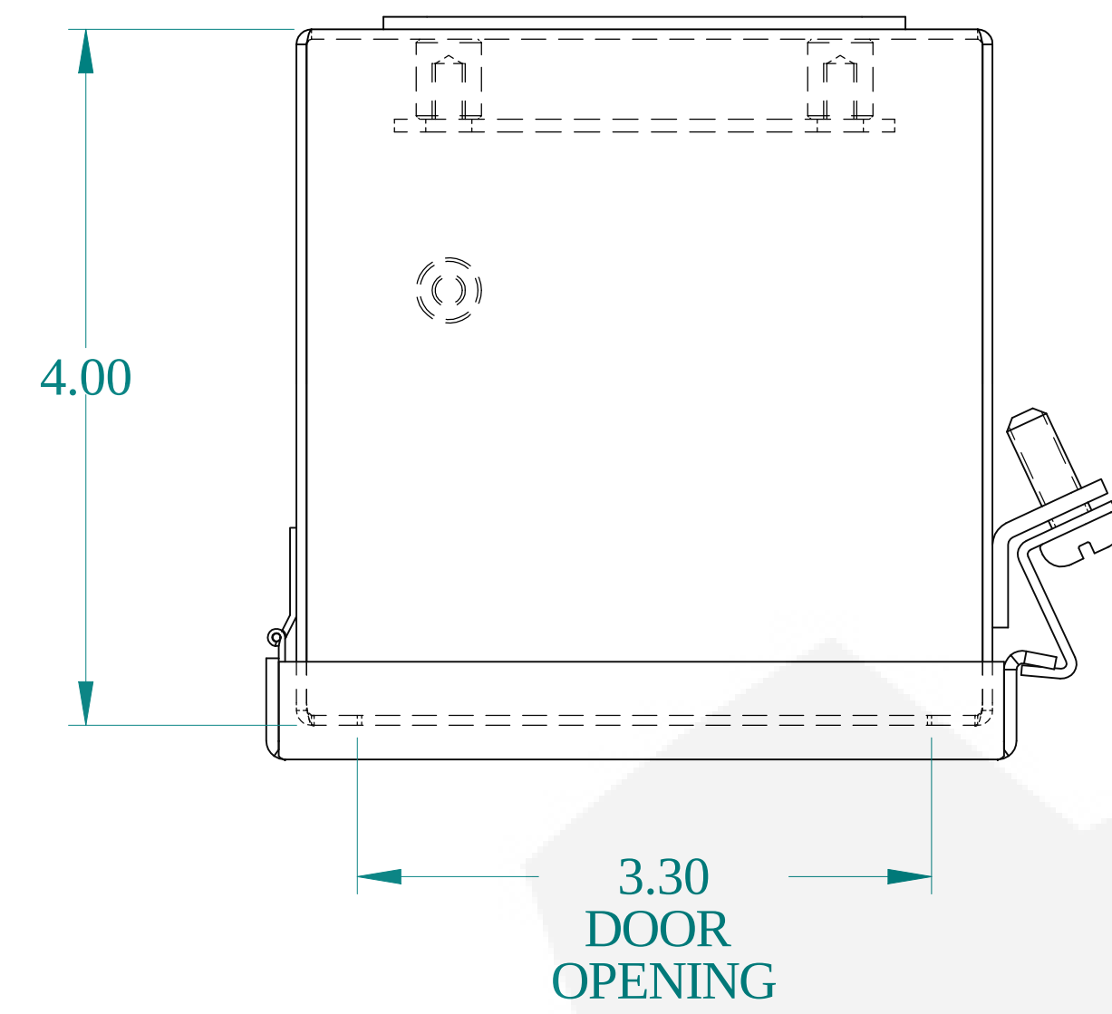
TOP VIEW
