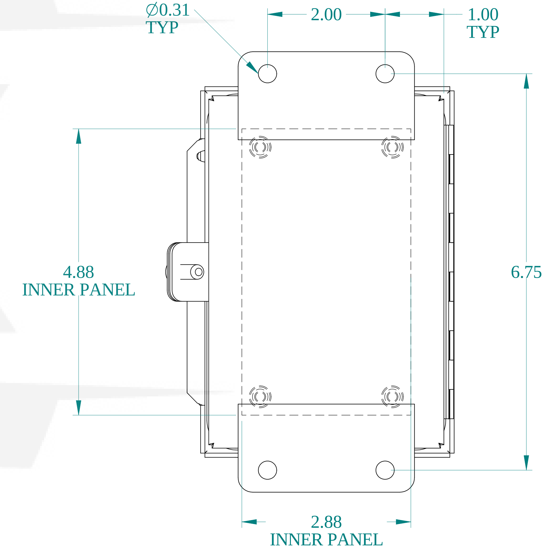
BACK VIEW
