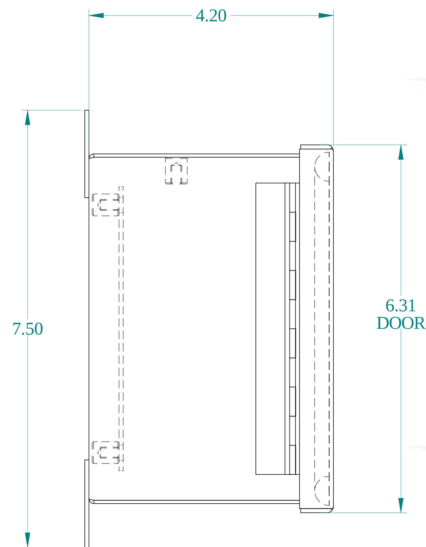
SIDE VIEW
