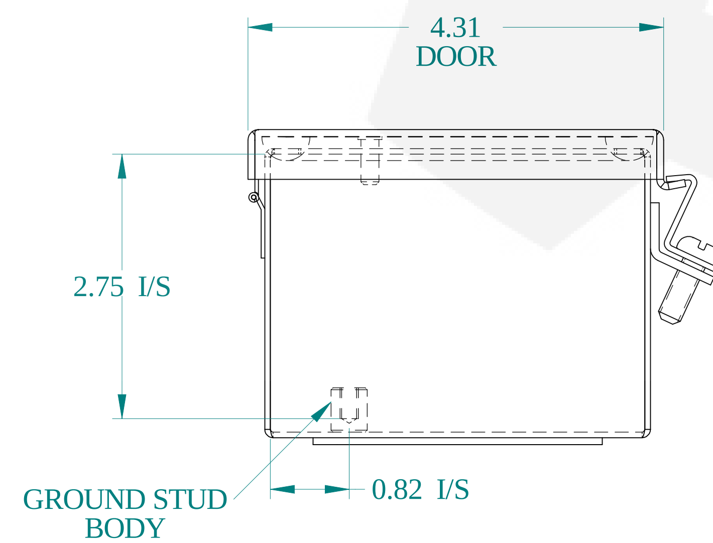
BOTTOM VIEW
