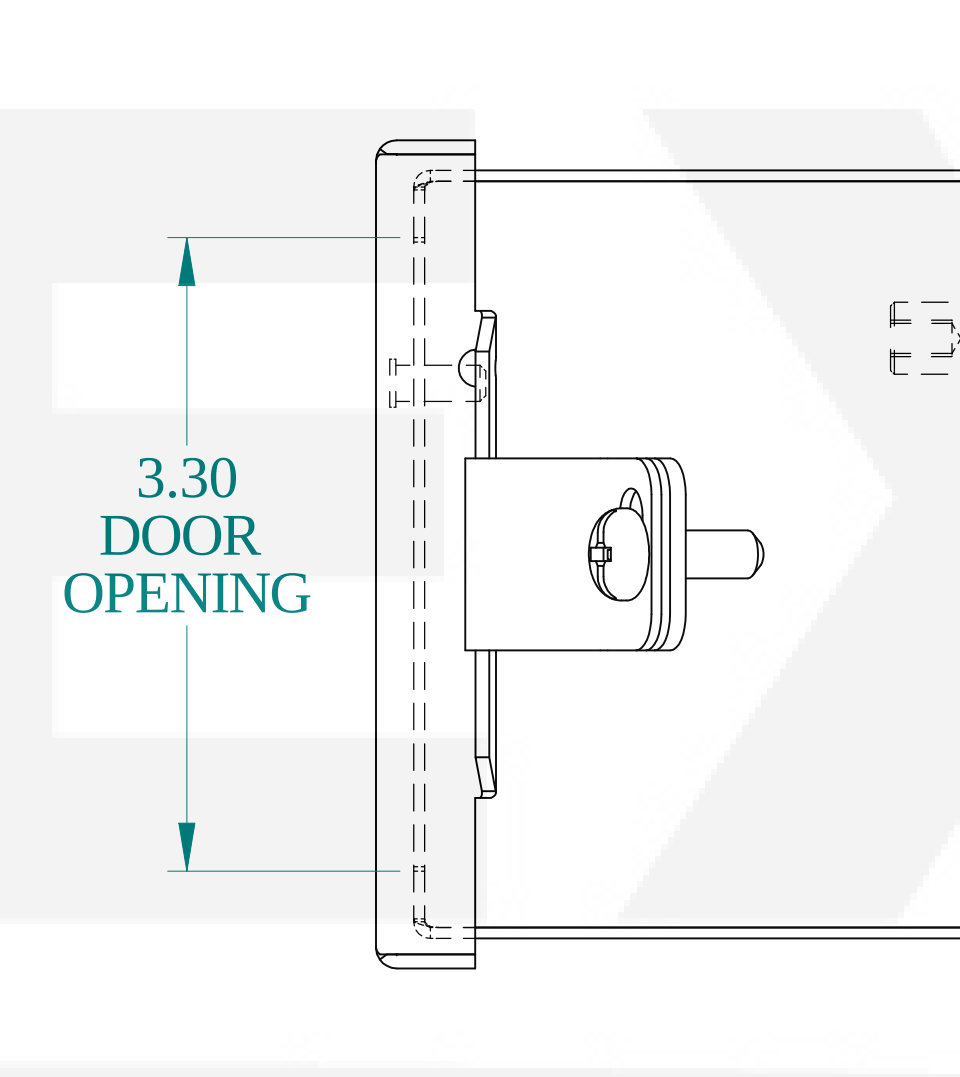
SIDE VIEW
