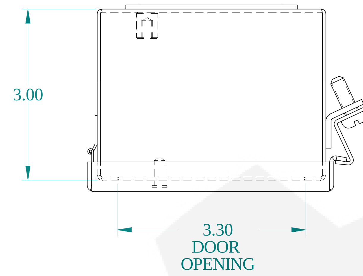
TOP VIEW
