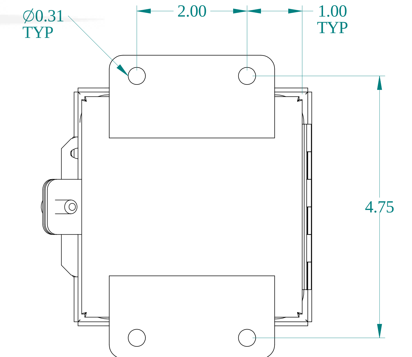
BACK VIEW
