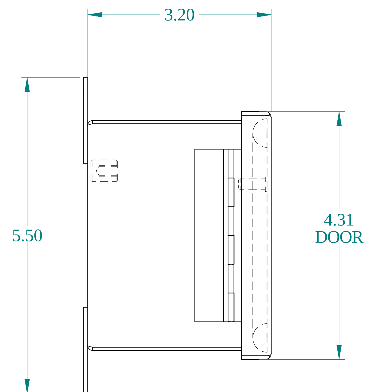
SIDE VIEW
