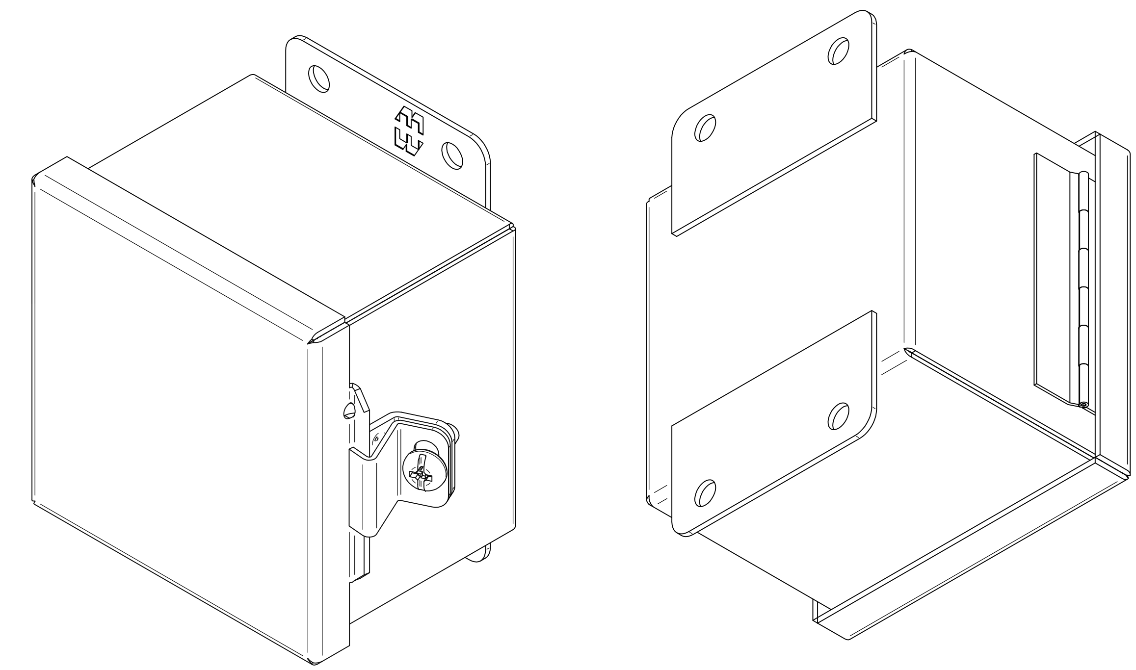
ISOMETRIC VIEWS
