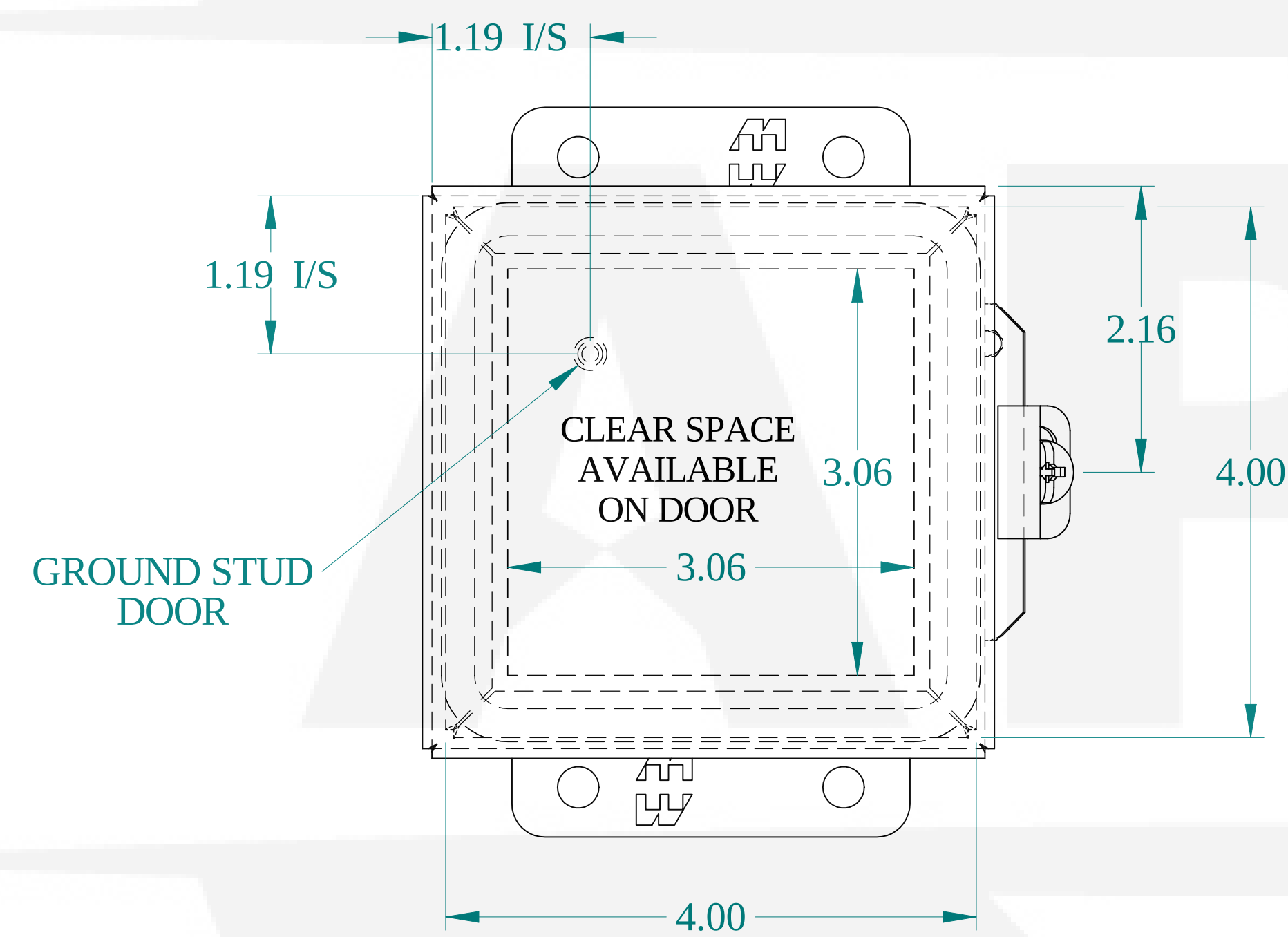
FRONT VIEW
