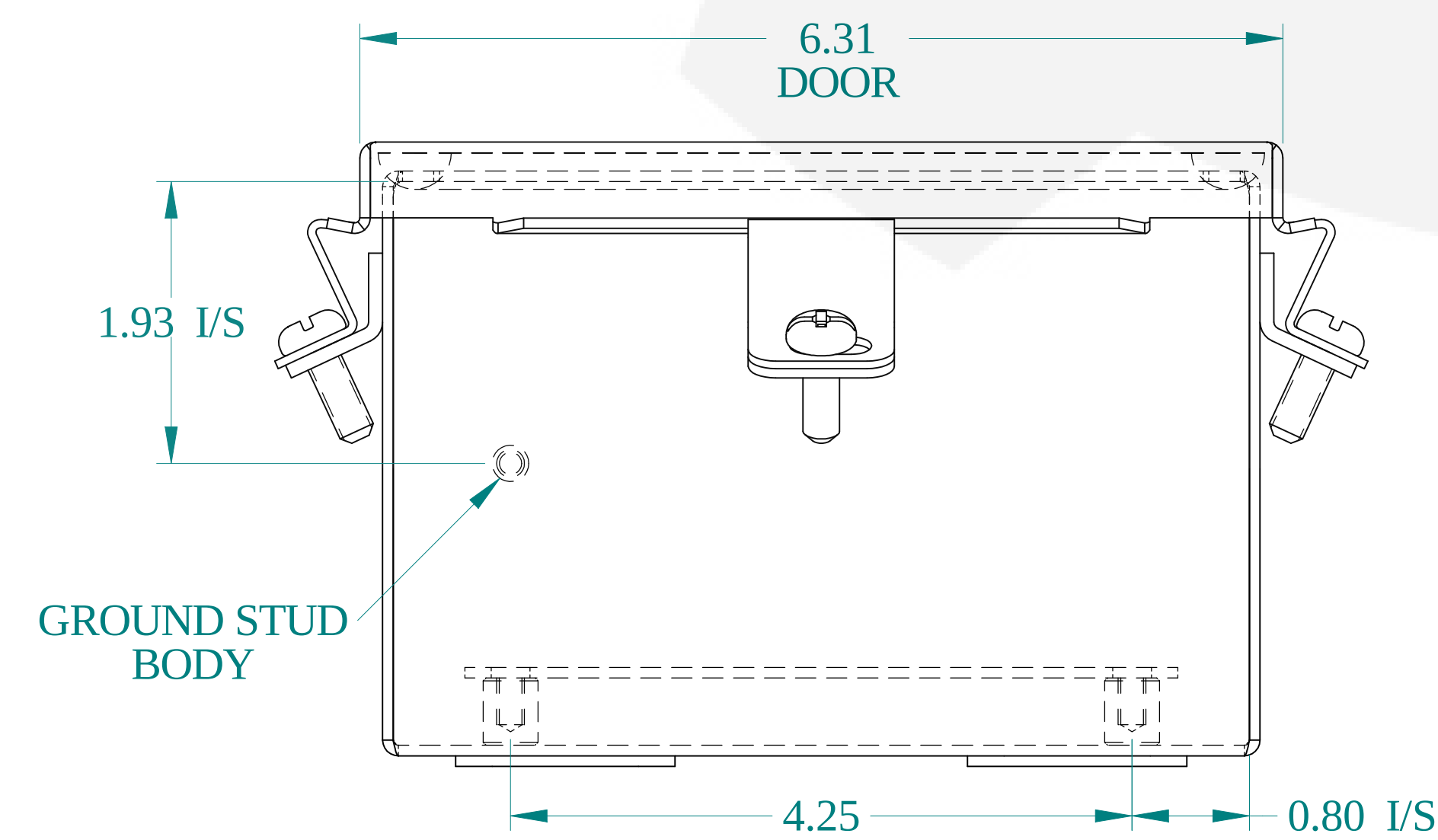
BOTTOM VIEW
