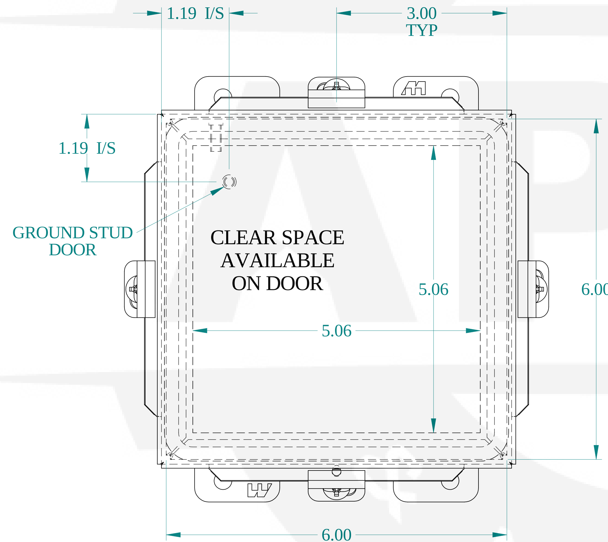
FRONT VIEW
