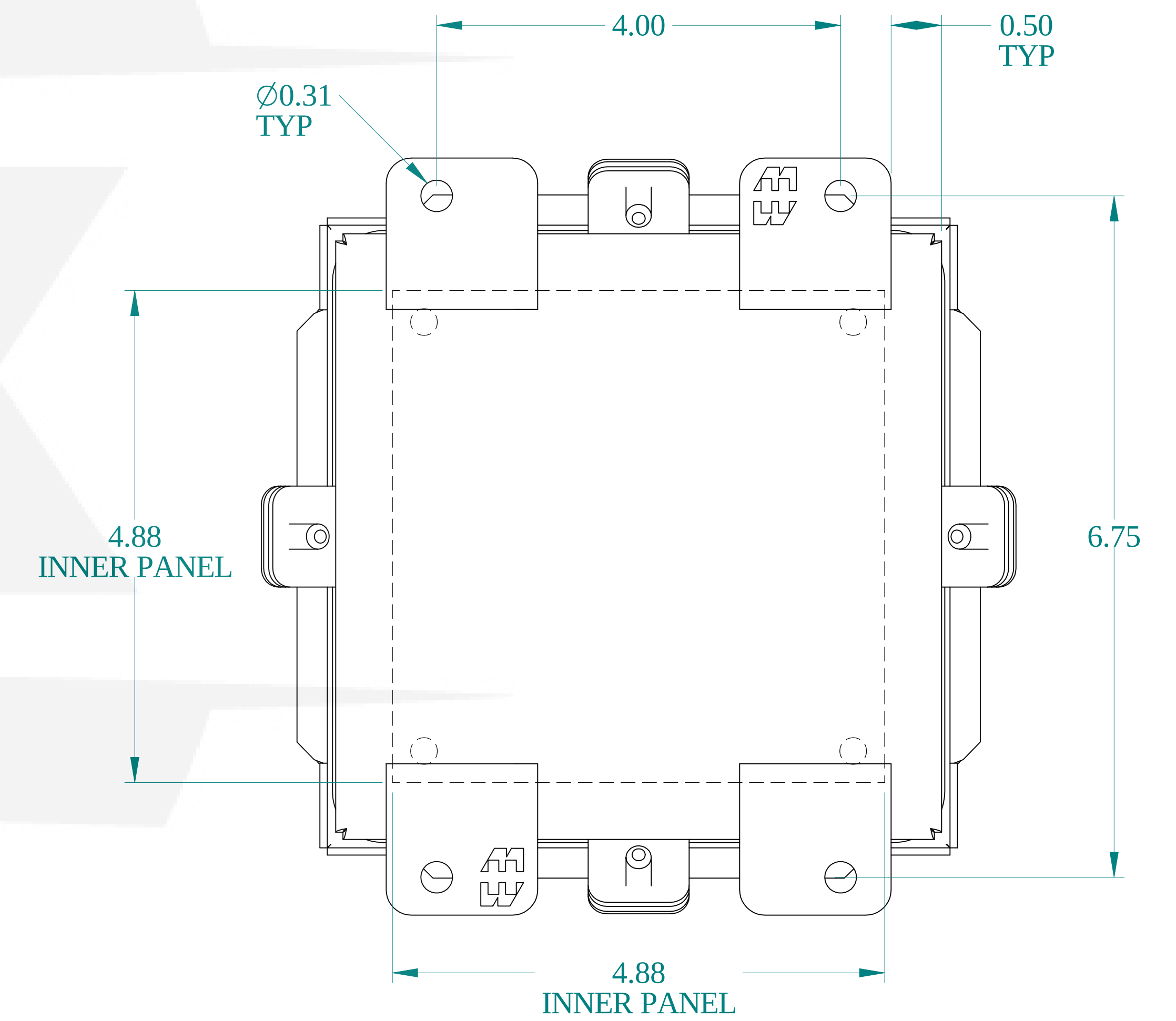
BACK VIEW
