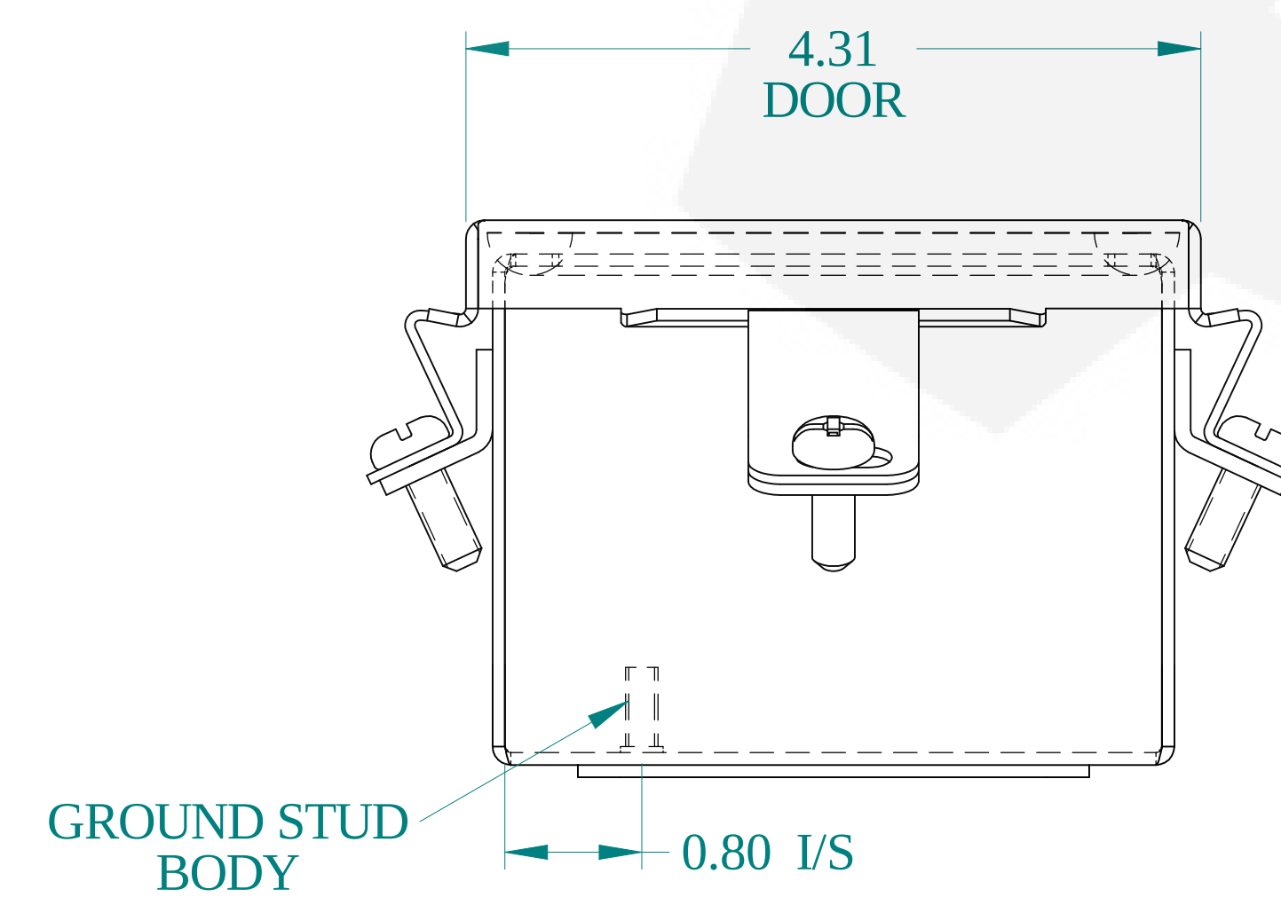
BOTTOM VIEW
