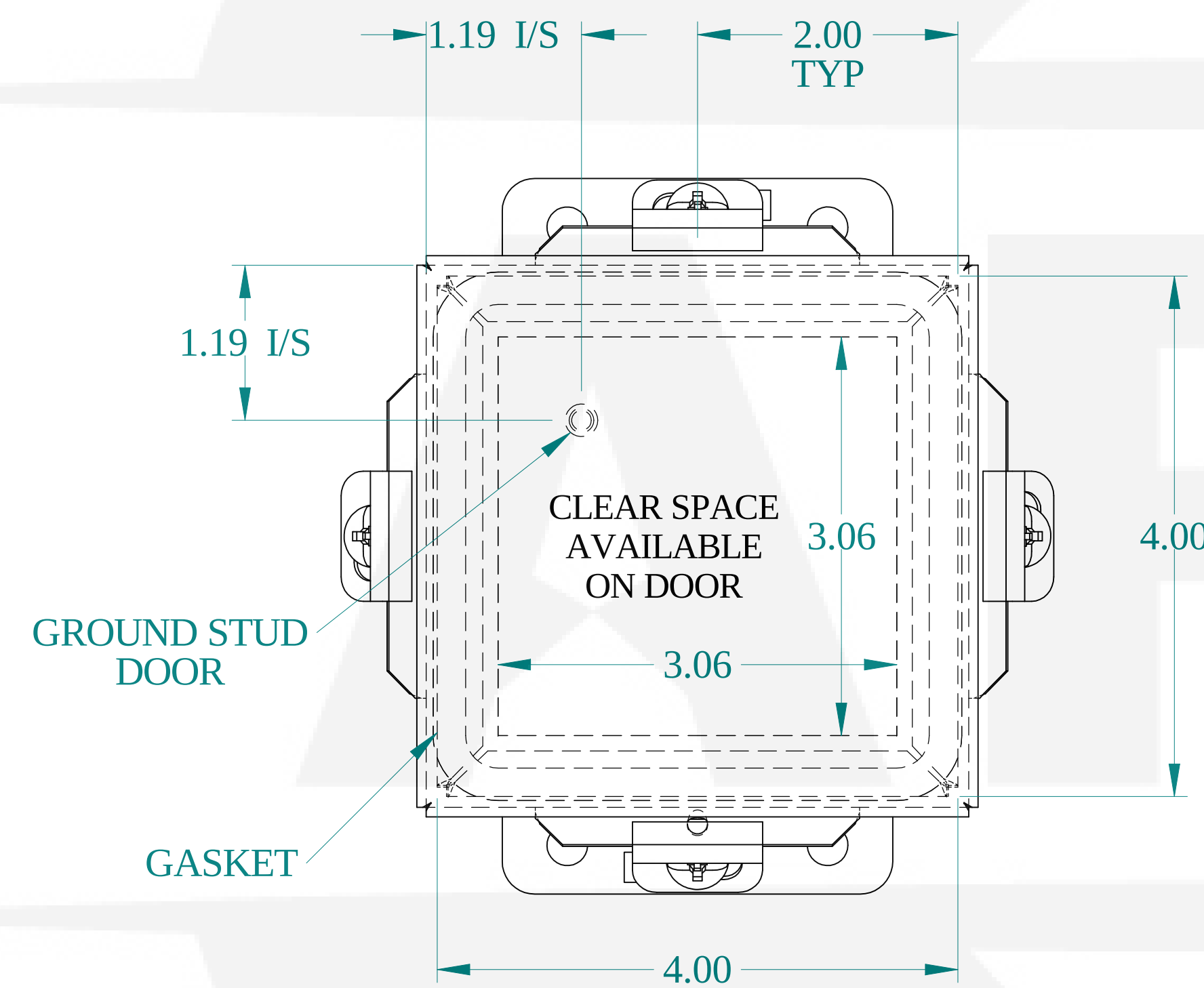
FRONT VIEW
