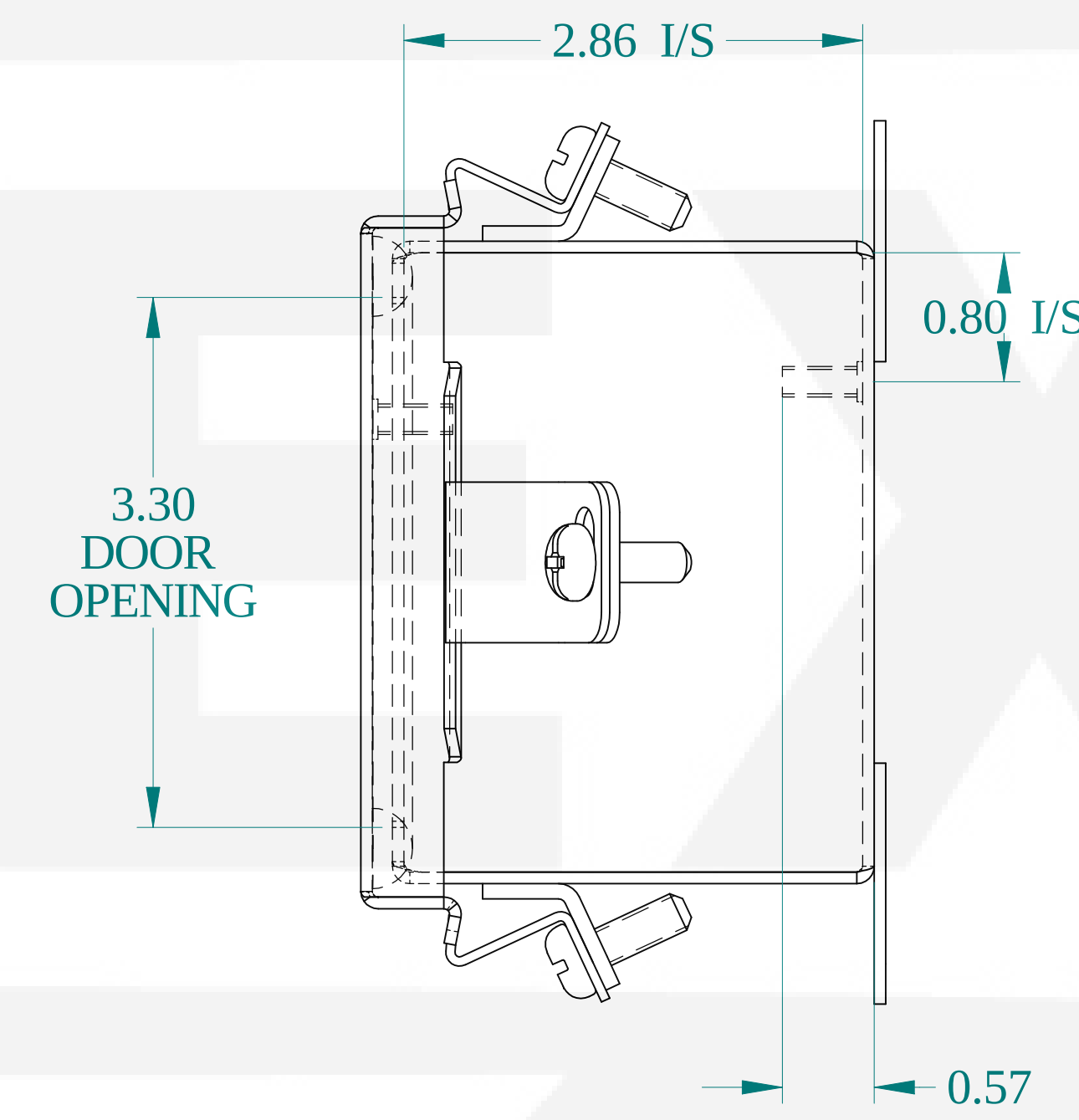
SIDE VIEW
