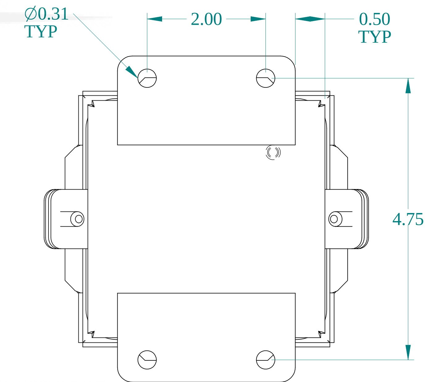
BACK VIEW
