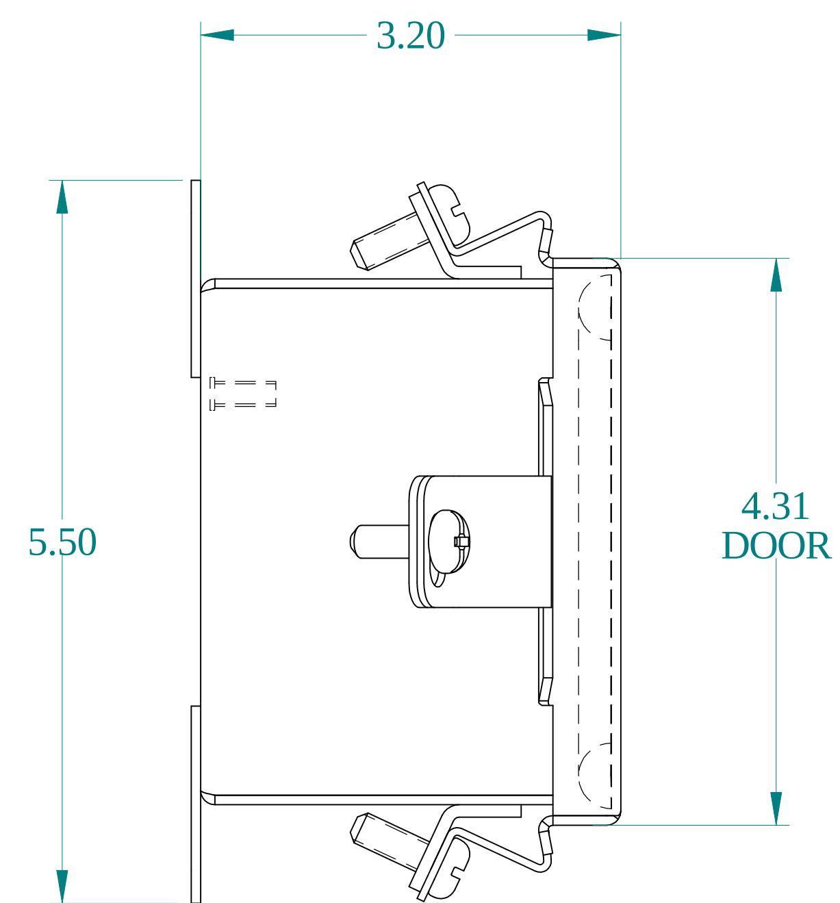
SIDE VIEW
