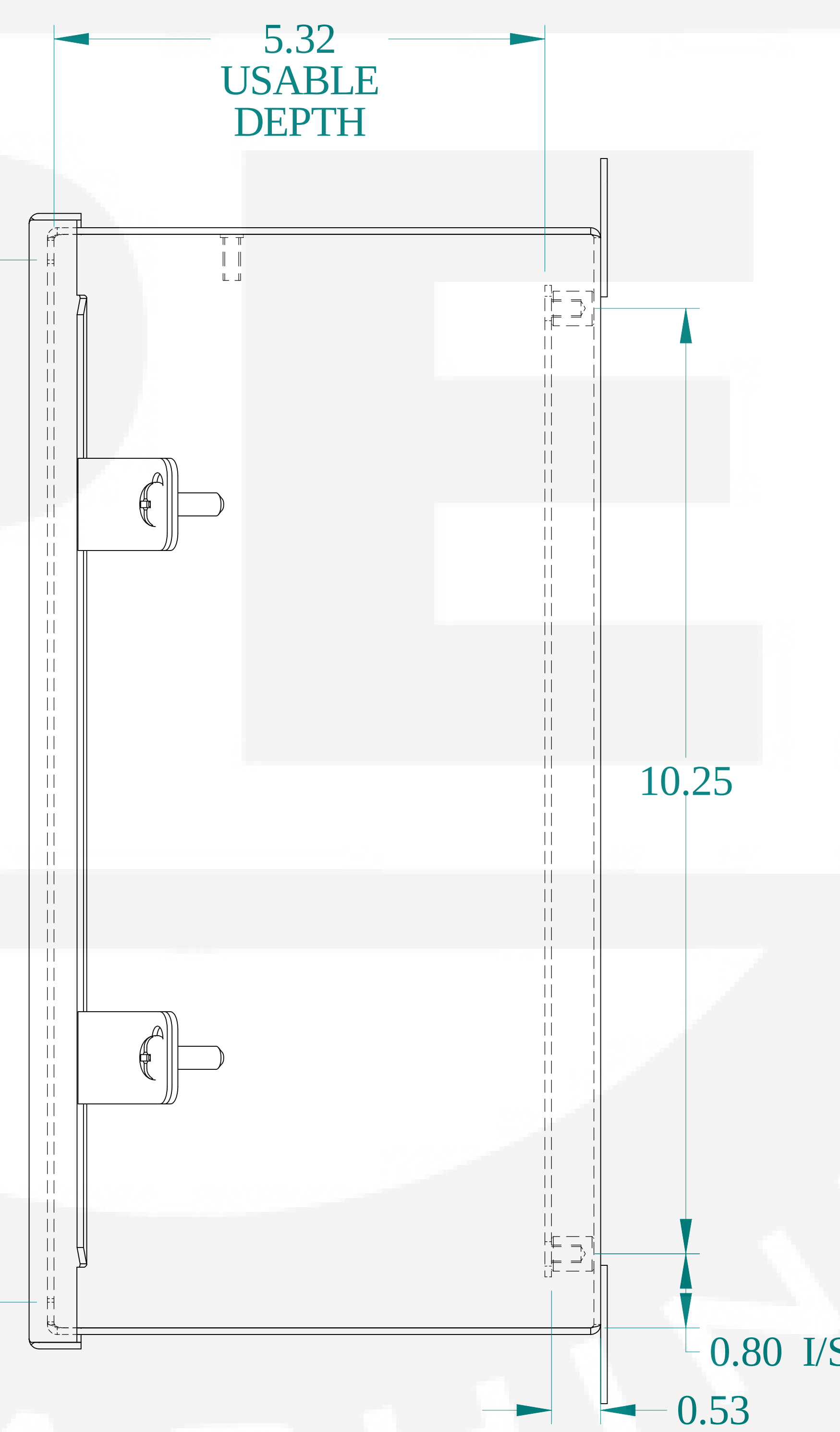
SIDE VIEW
