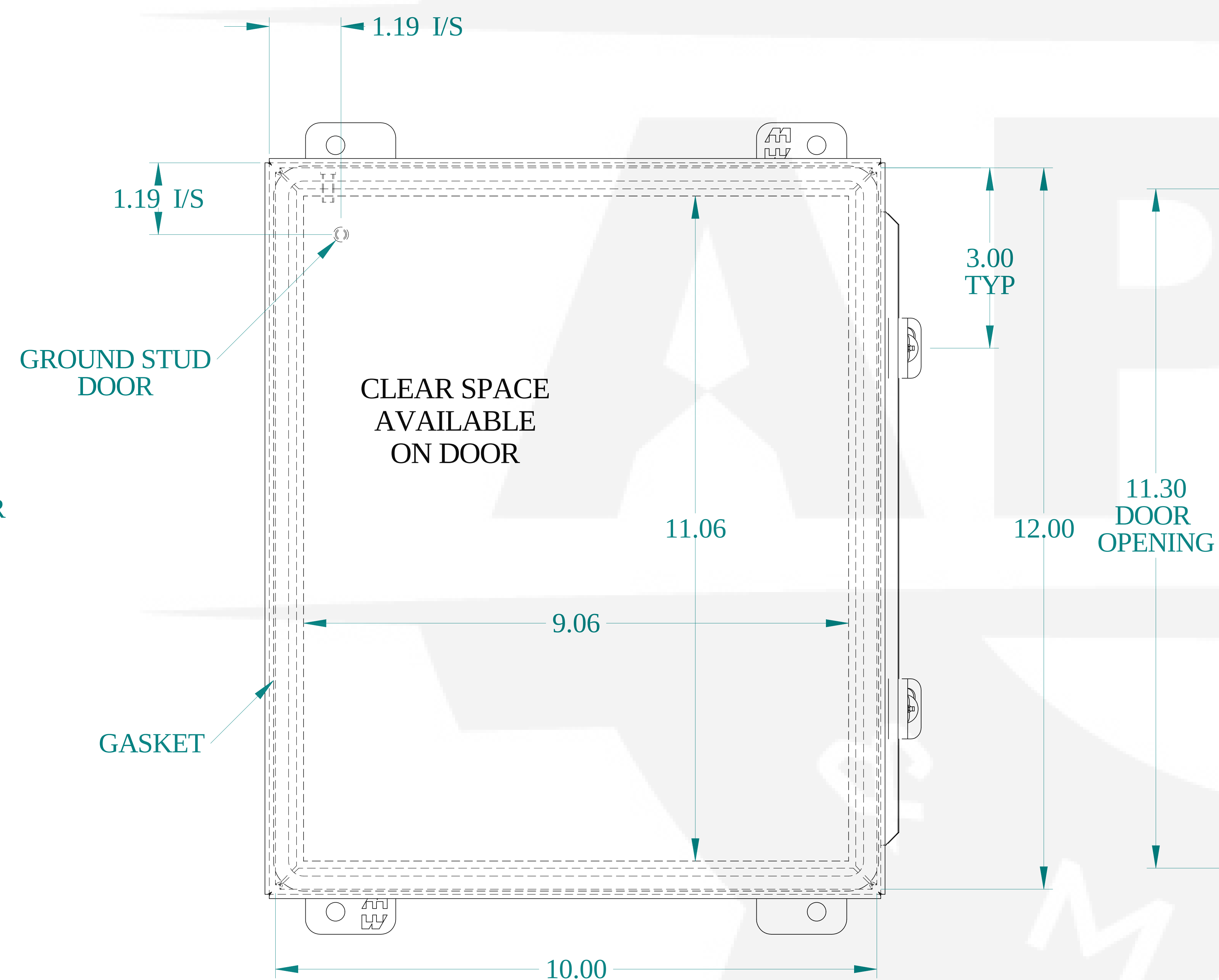
FRONT VIEW
