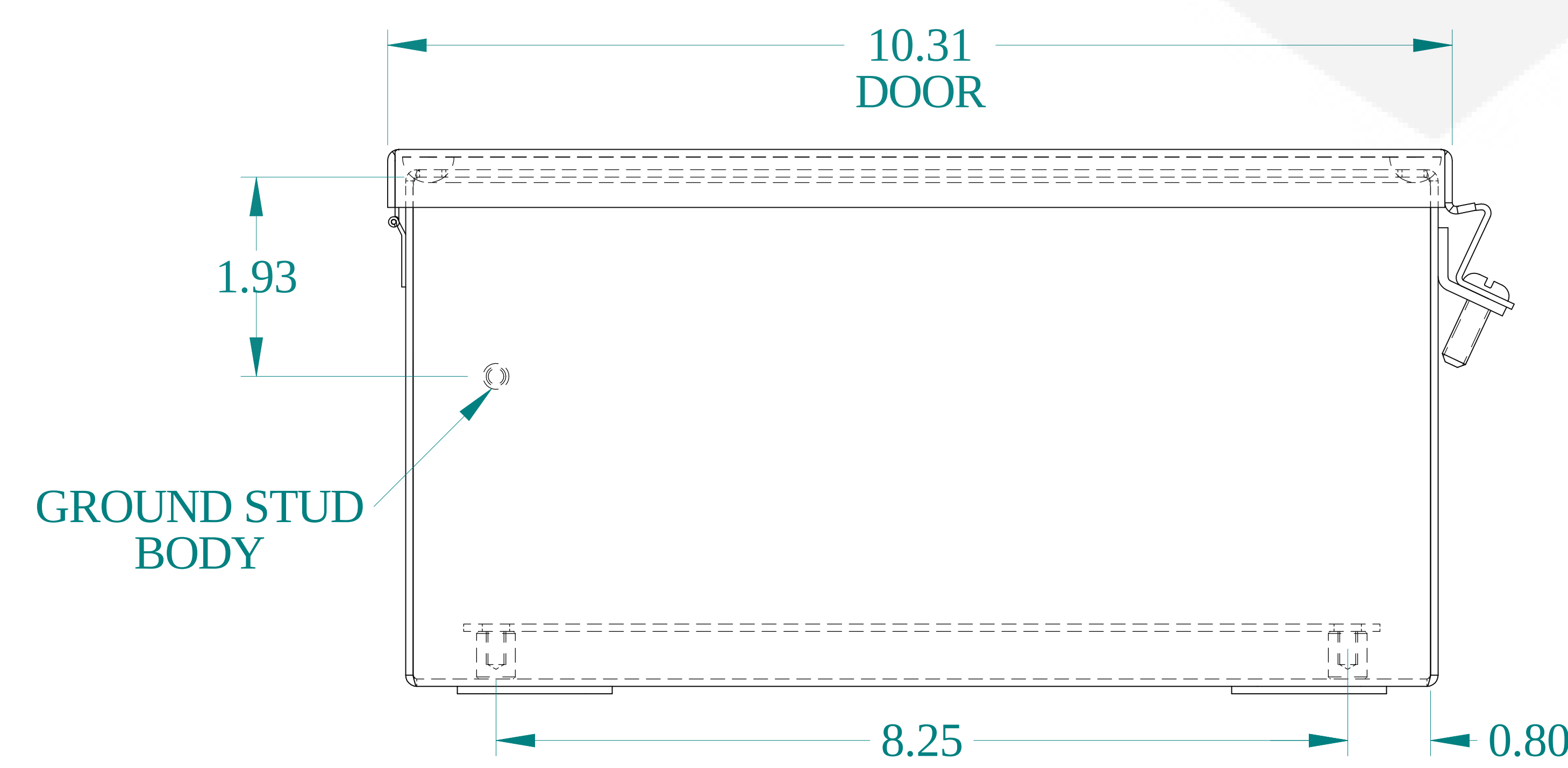
BOTTOM VIEW
