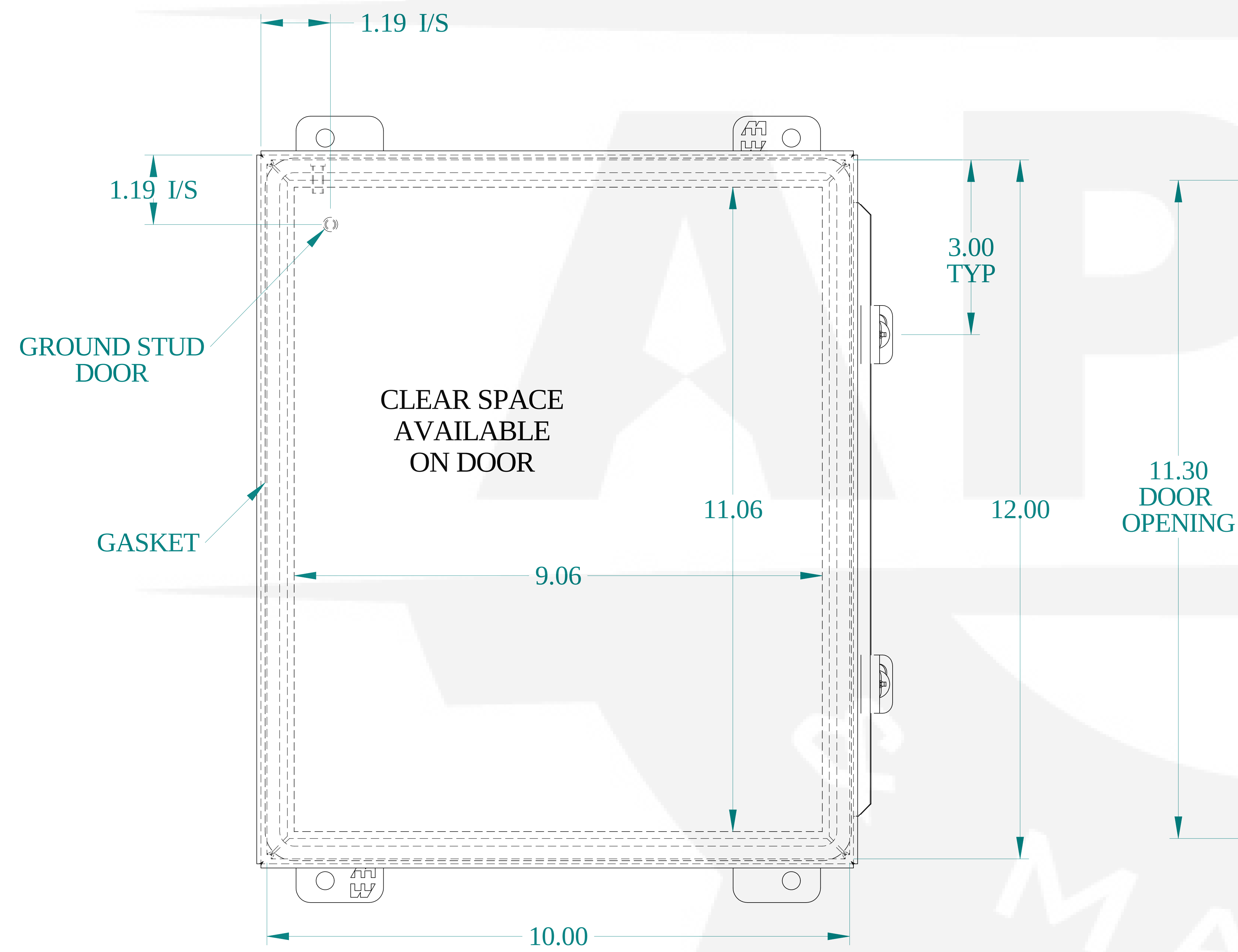
FRONT VIEW
