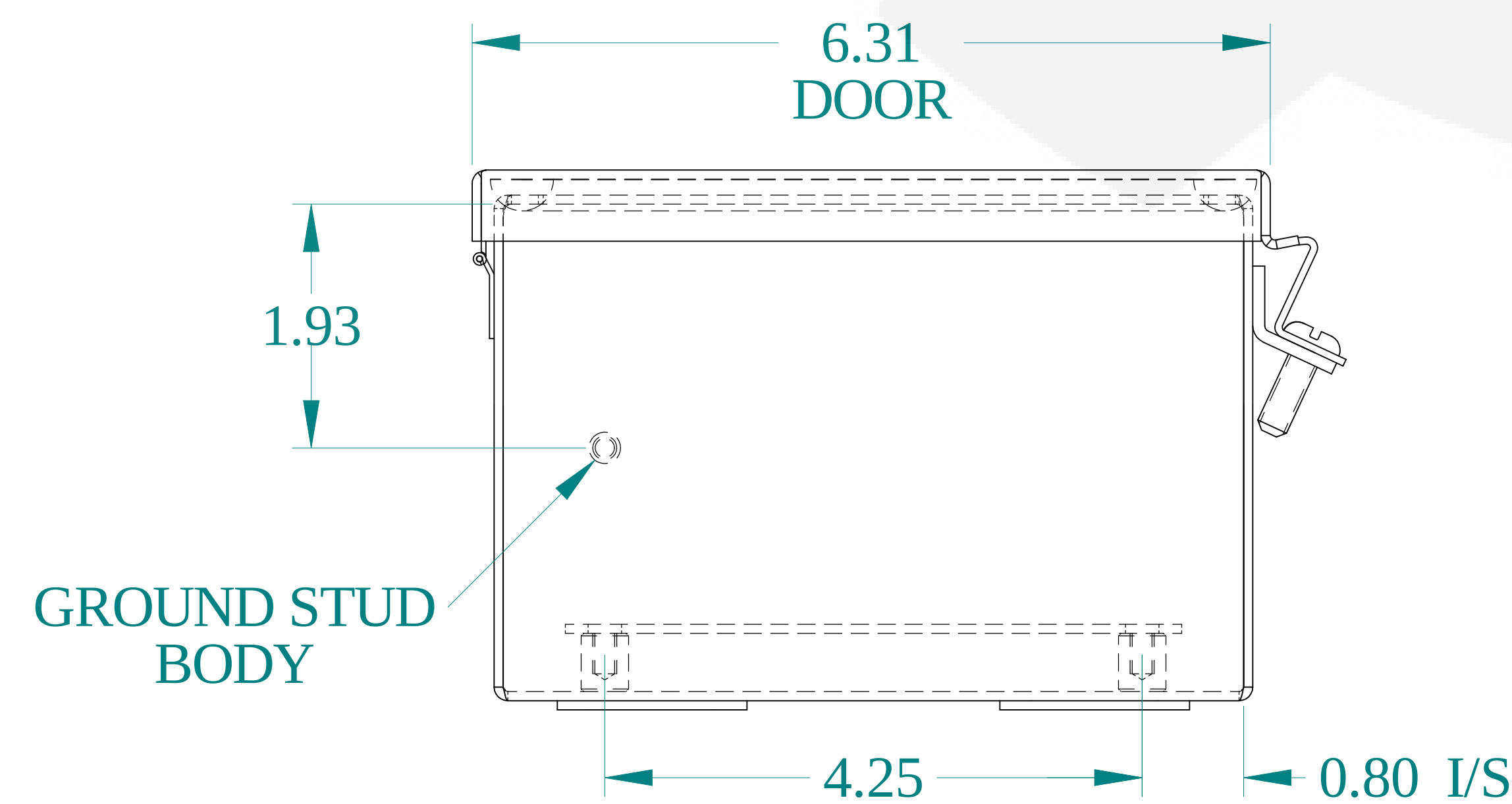
BOTTOM VIEW
