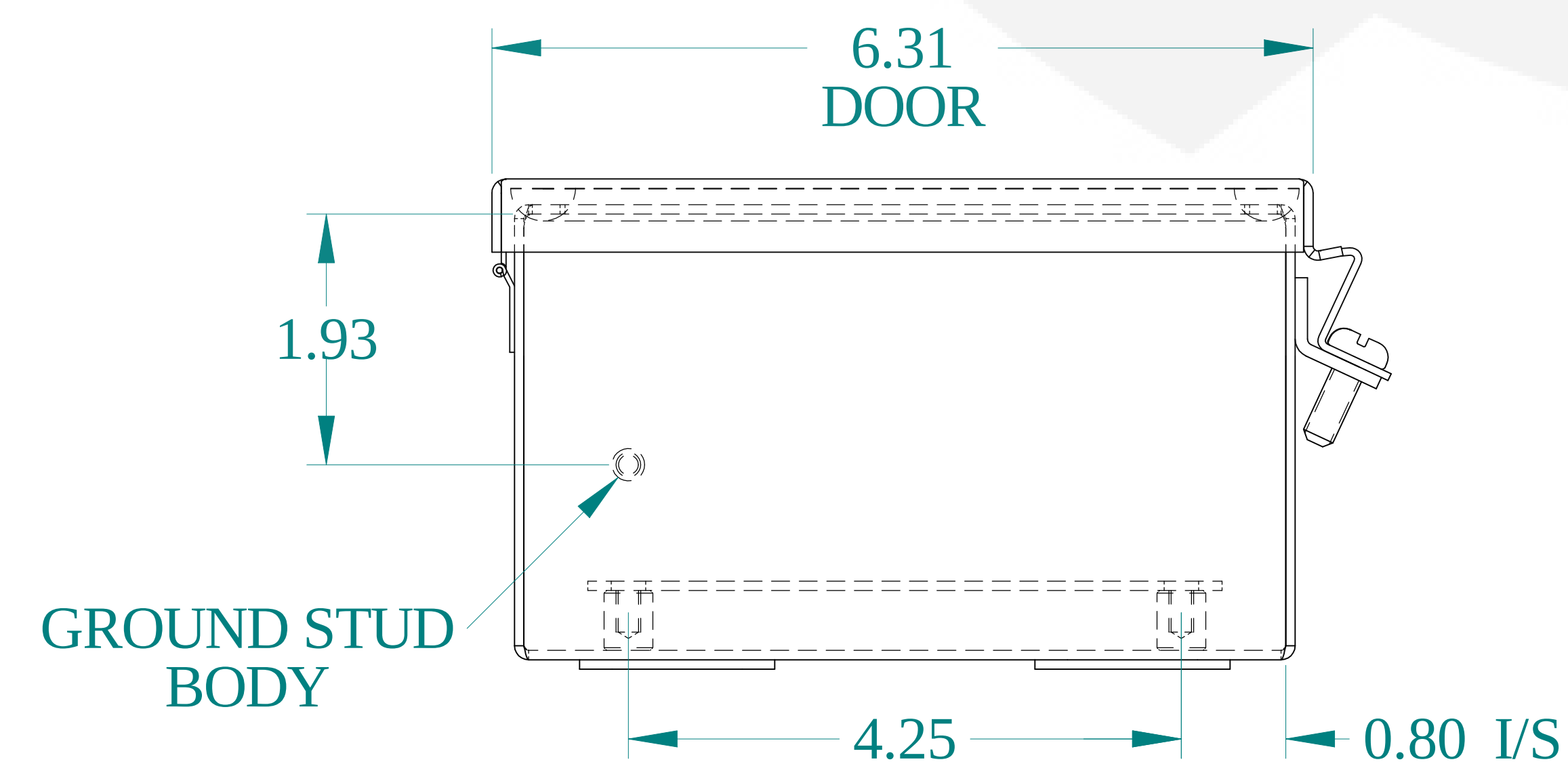
BOTTOM VIEW
