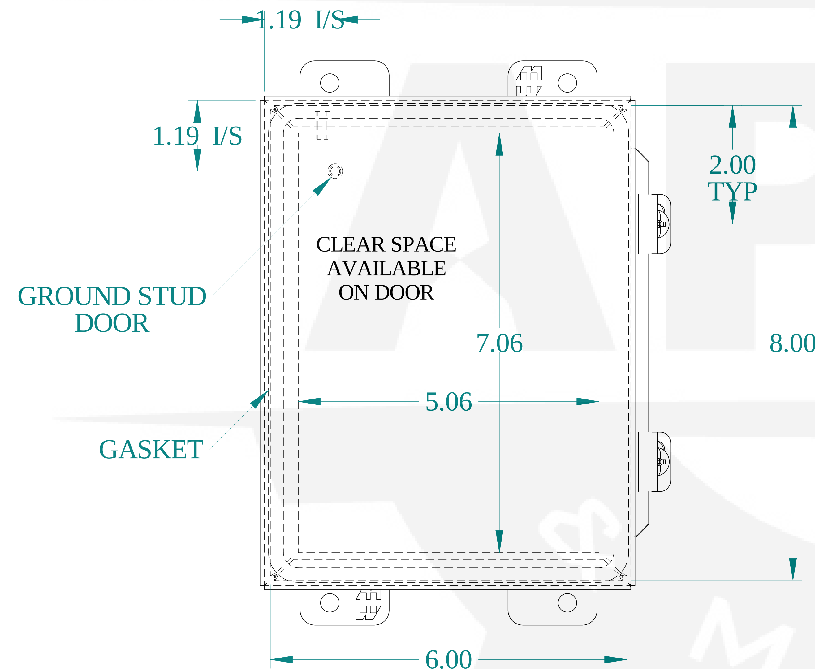
FRONT VIEW
