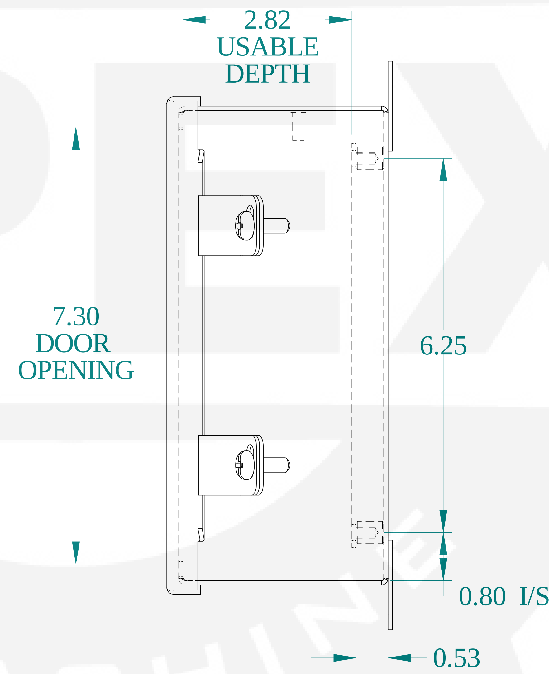
SIDE VIEW
