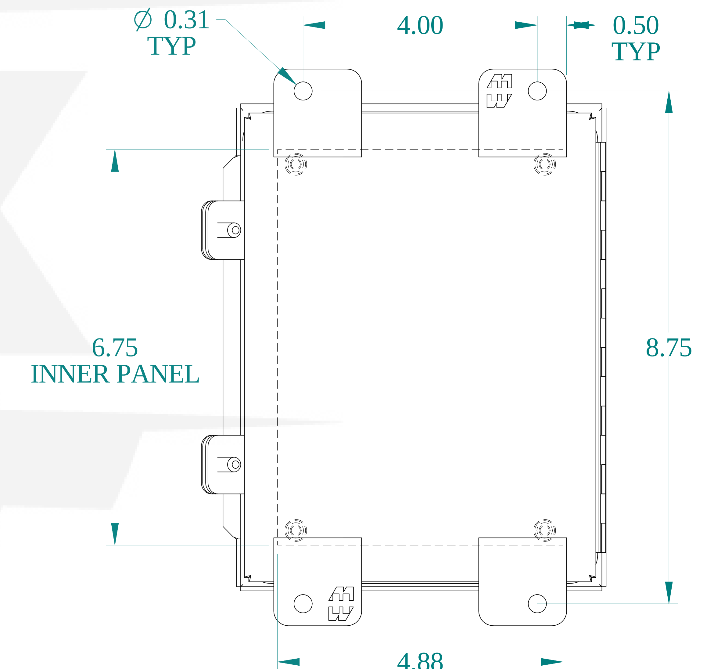
BACK VIEW
