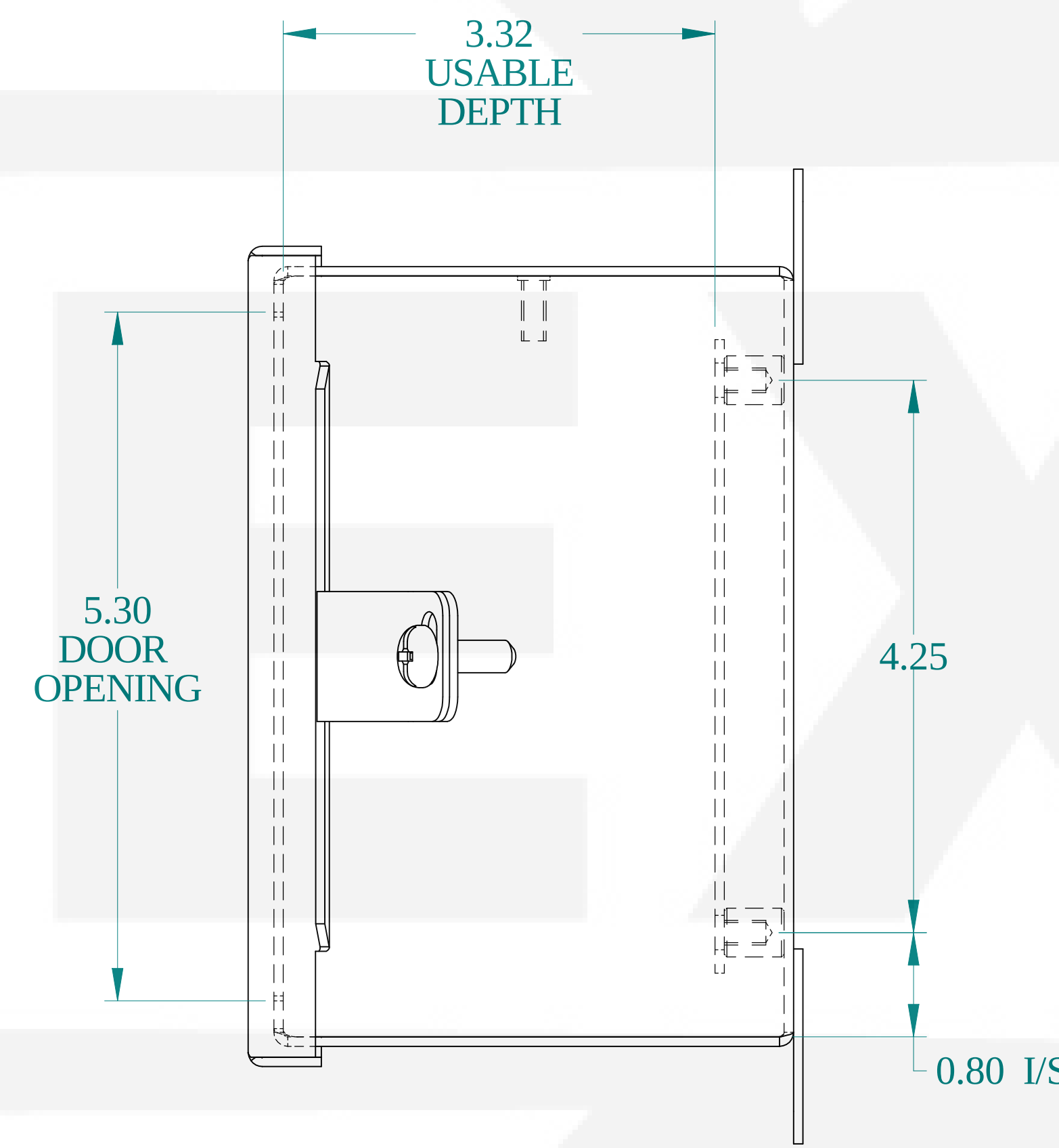
SIDE VIEW
