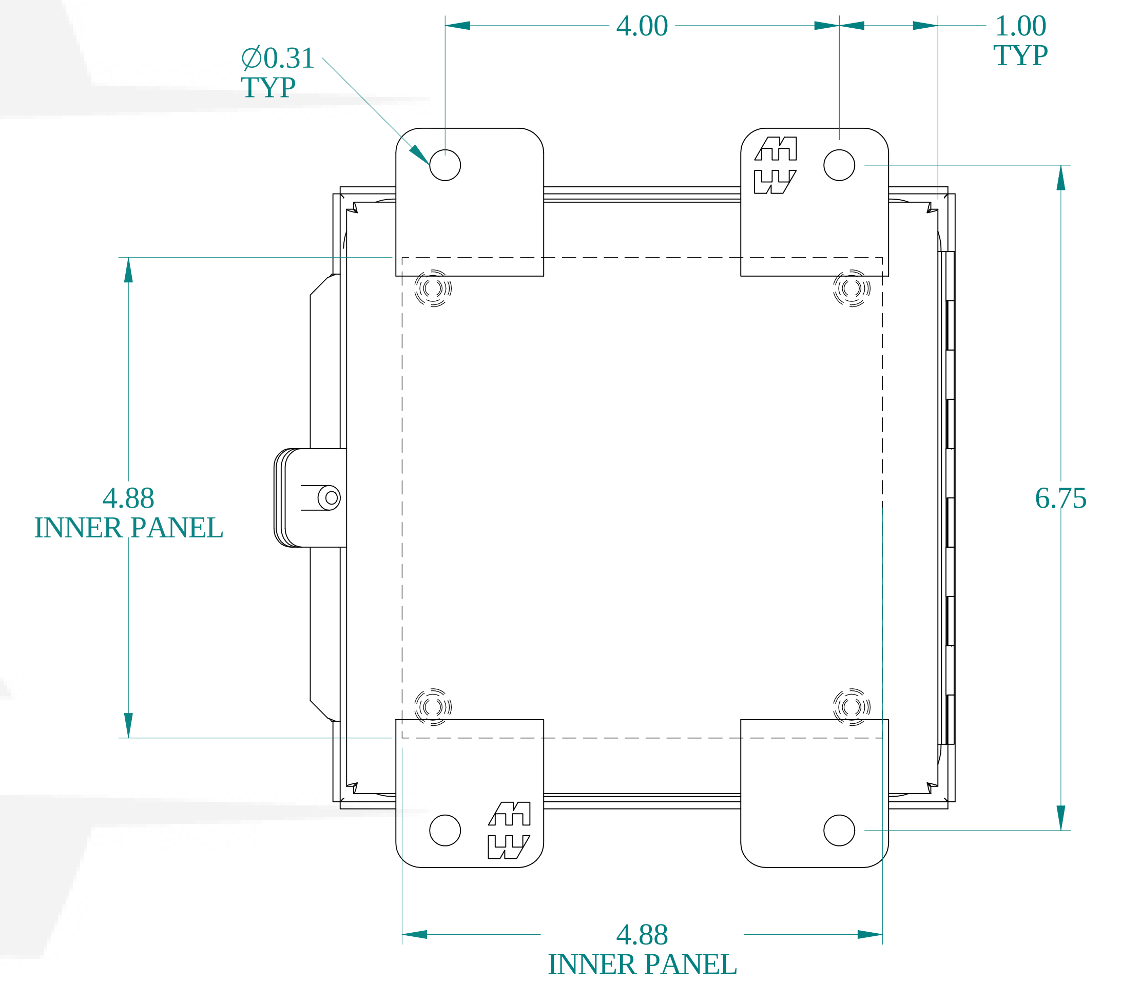
BACK VIEW
