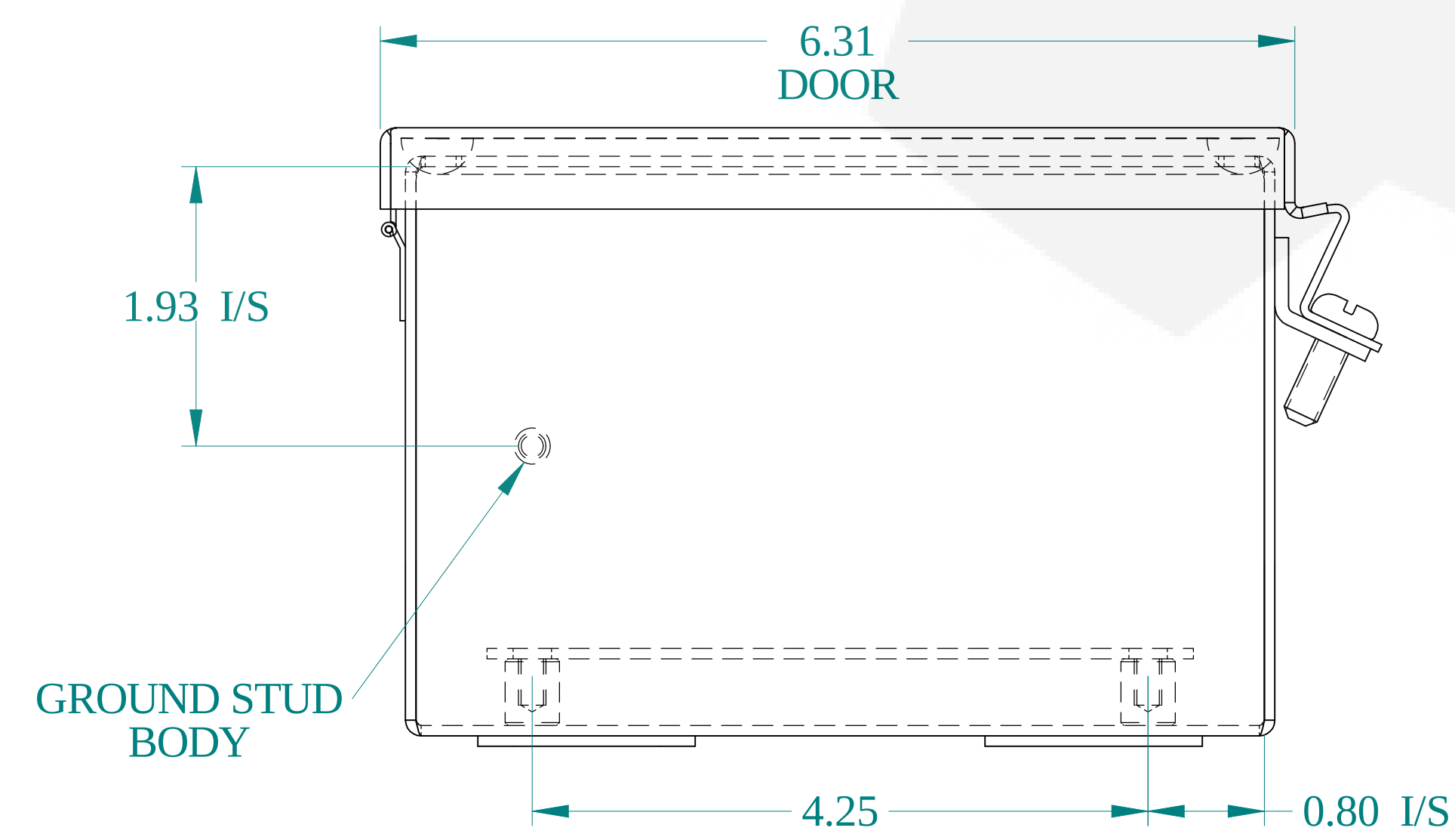
BOTTOM VIEW
