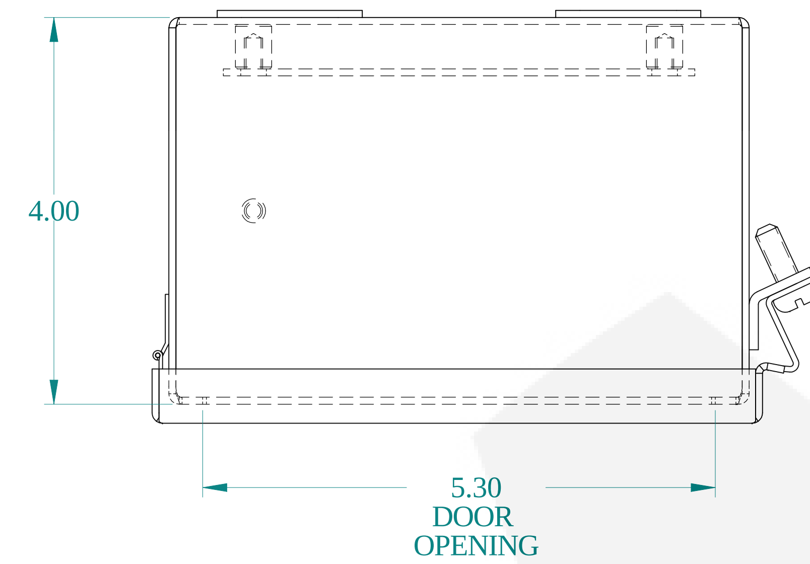
TOP VIEW
