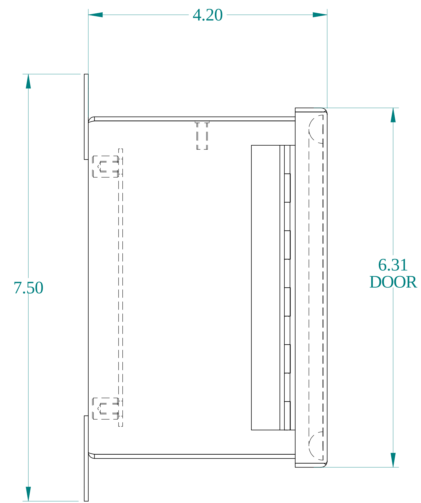
SIDE VIEW
