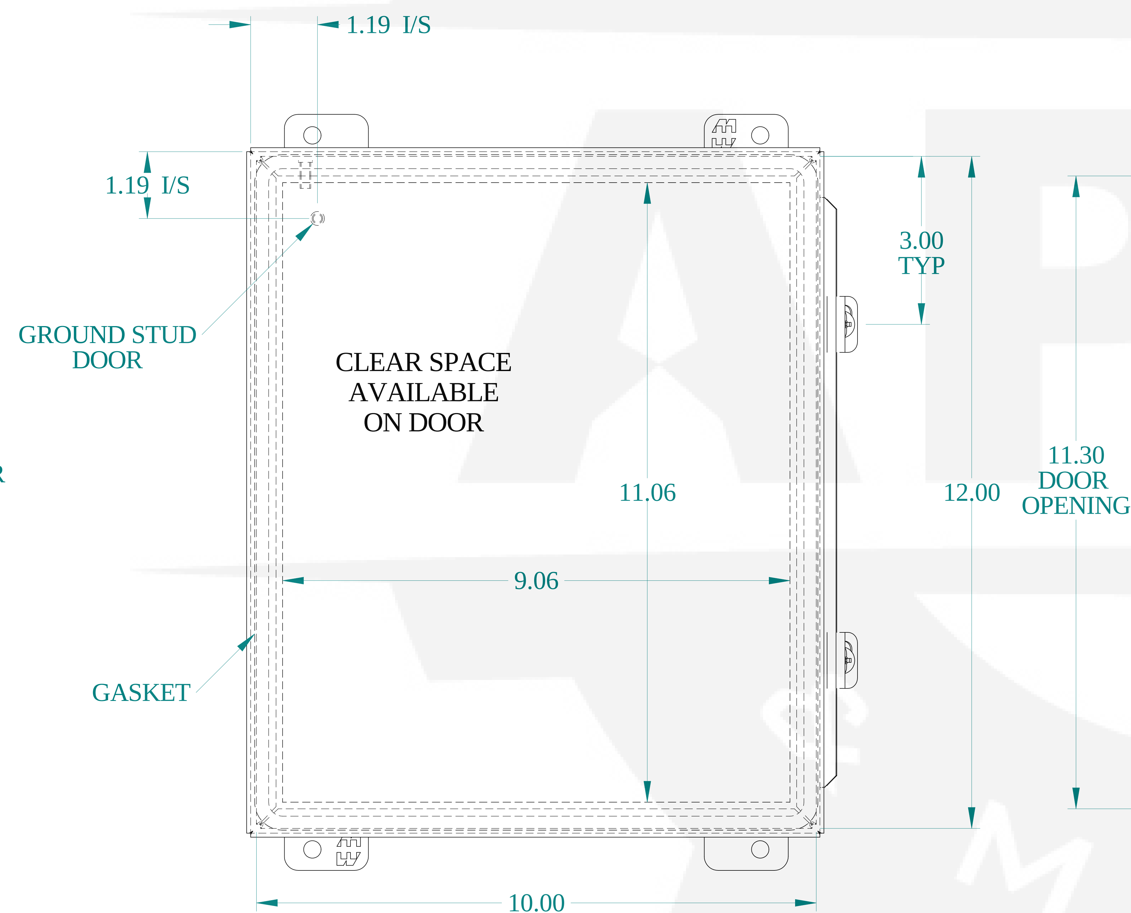
FRONT VIEW
