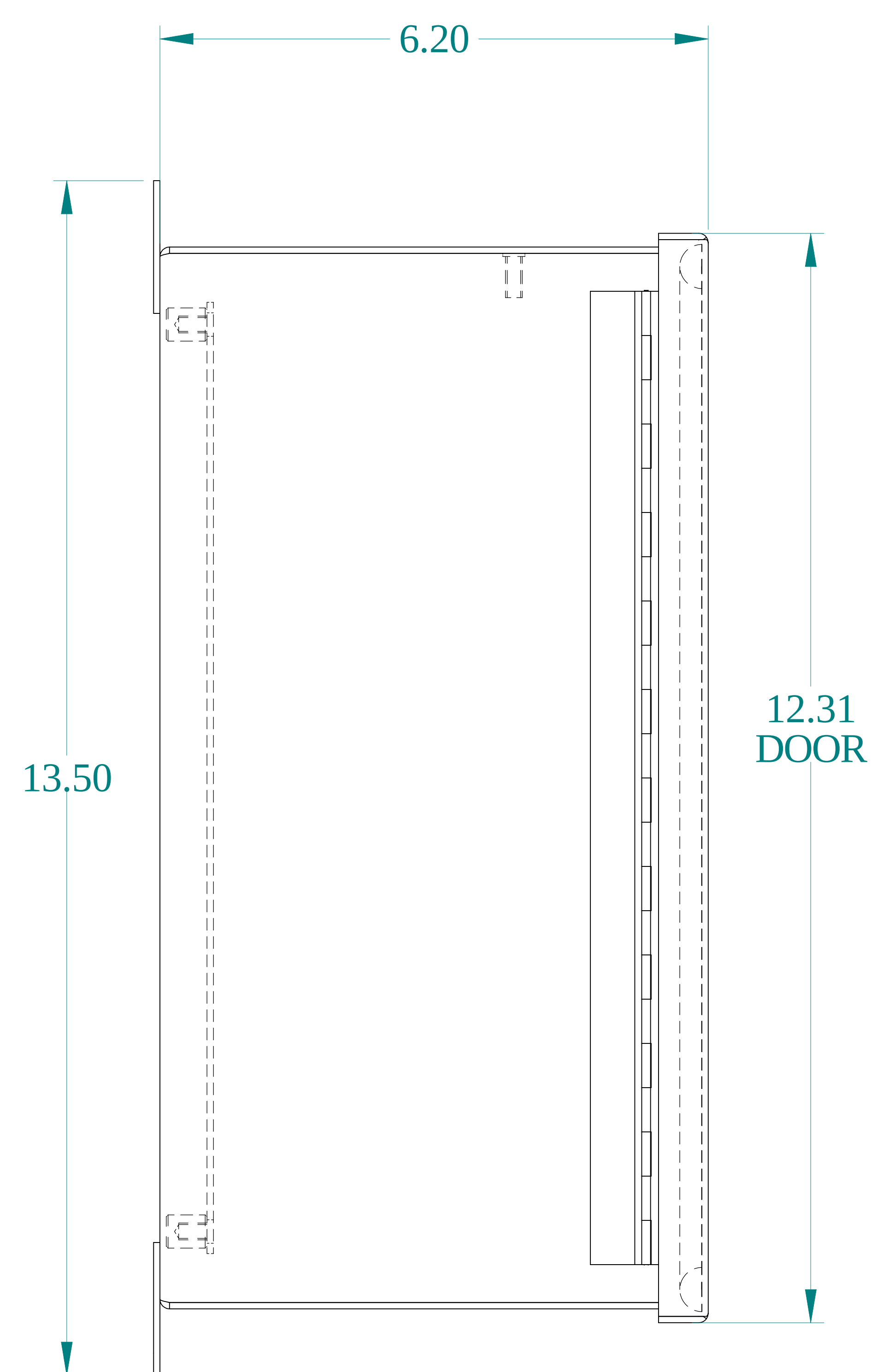
SIDE VIEW
