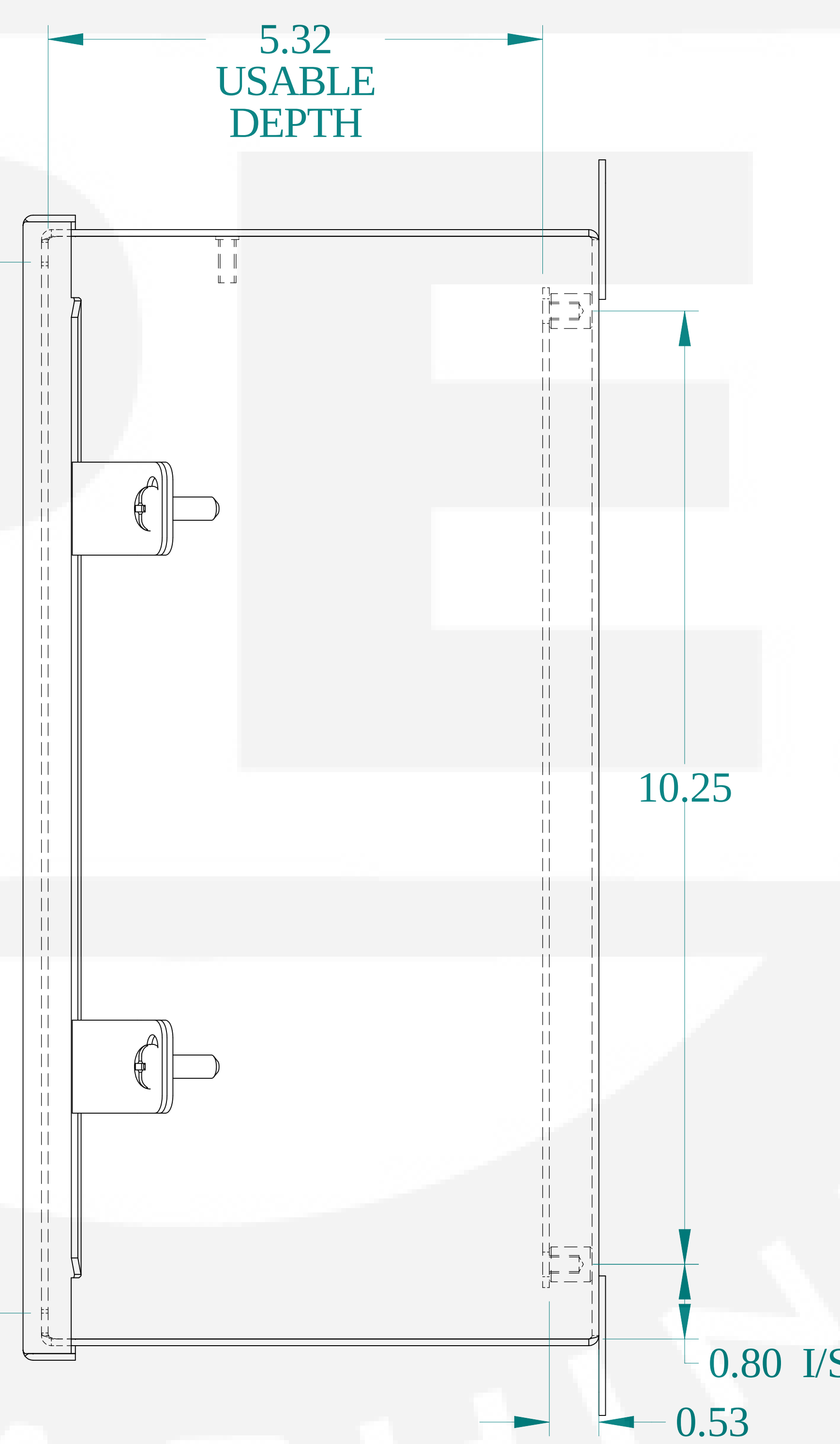
SIDE VIEW
