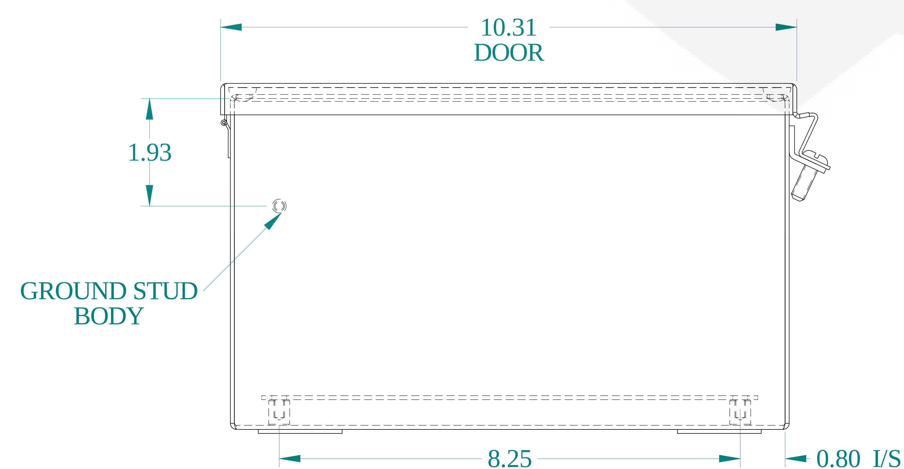
BOTTOM VIEW
