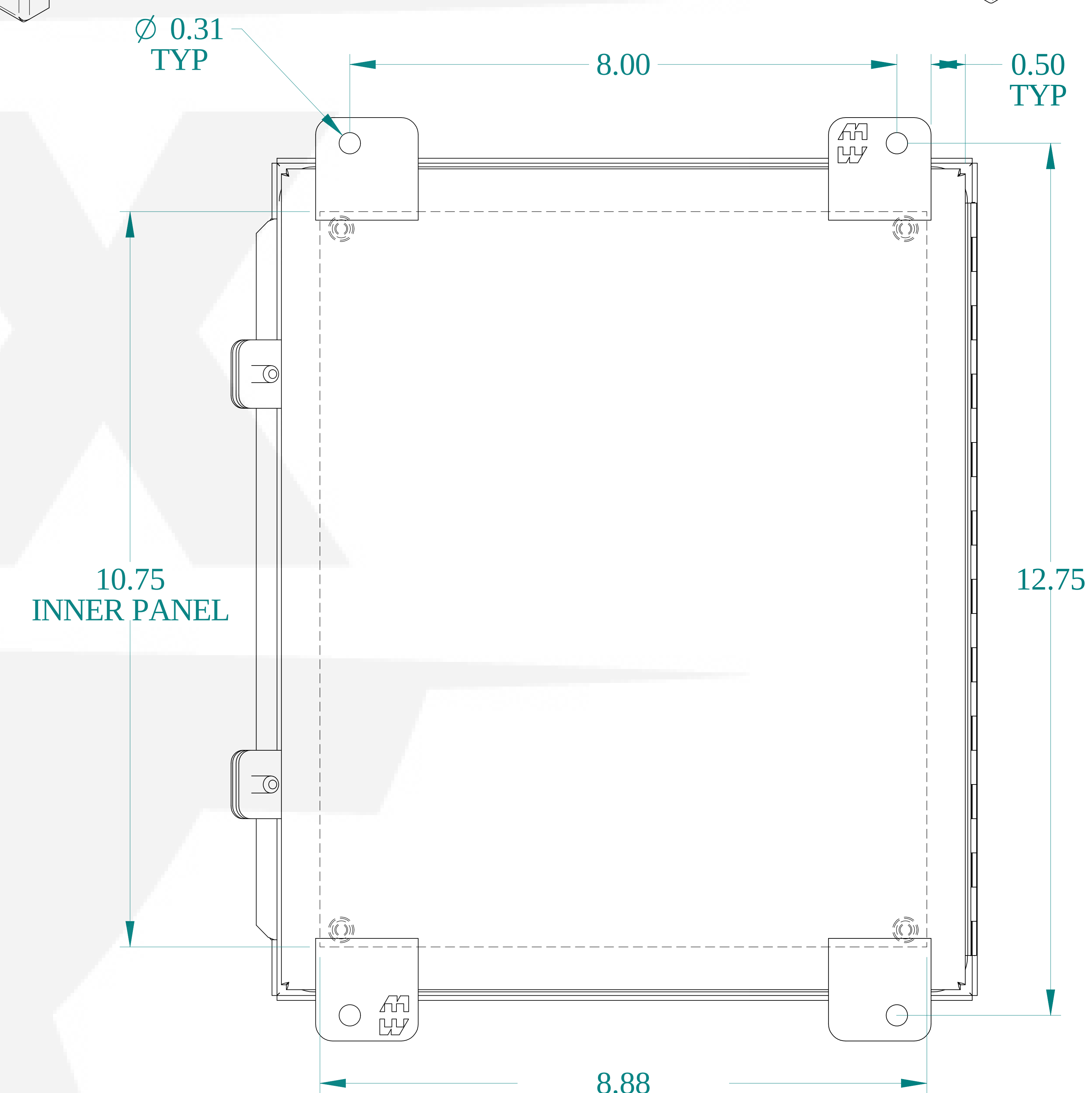
BACK VIEW
