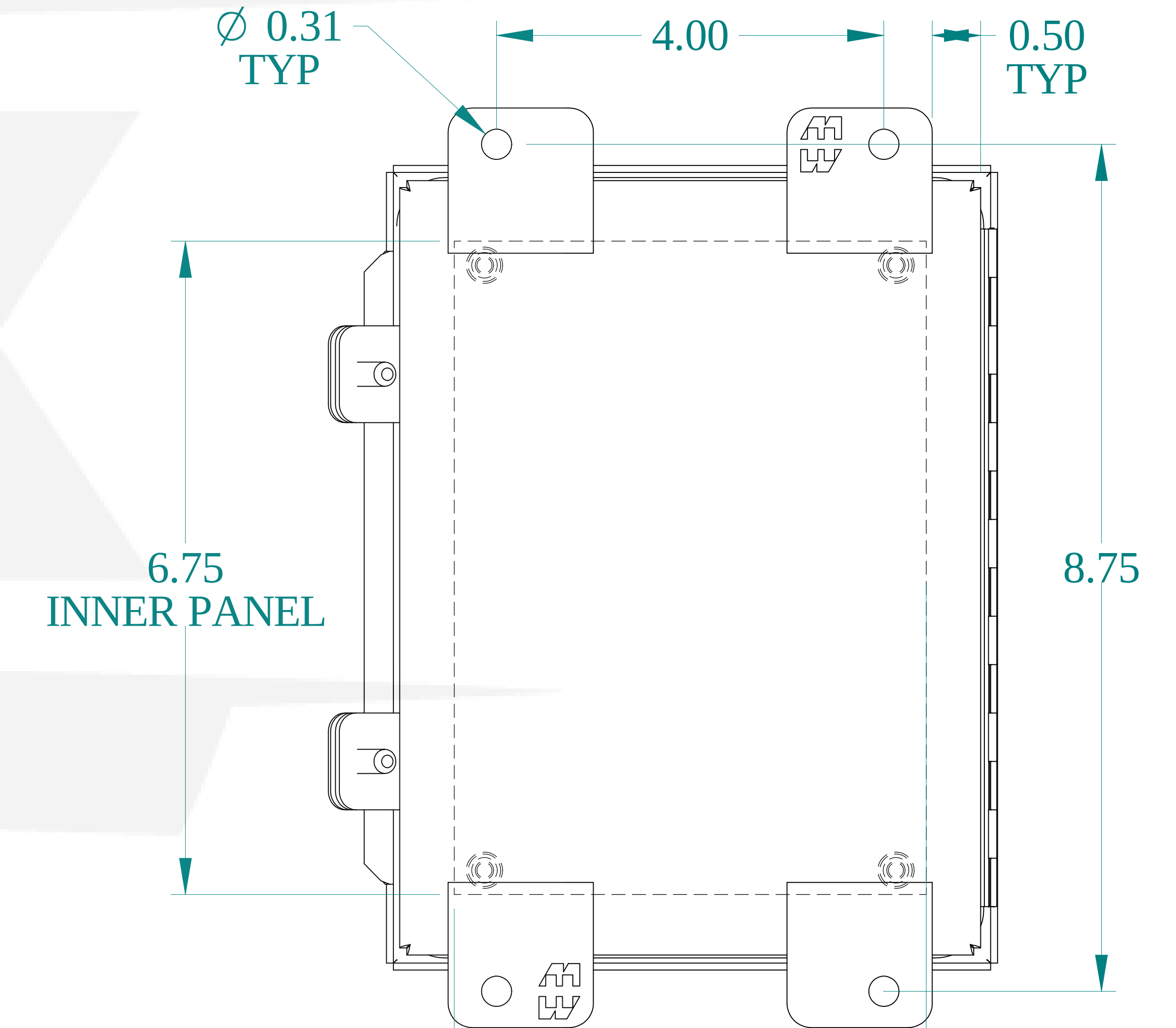
BACK VIEW
