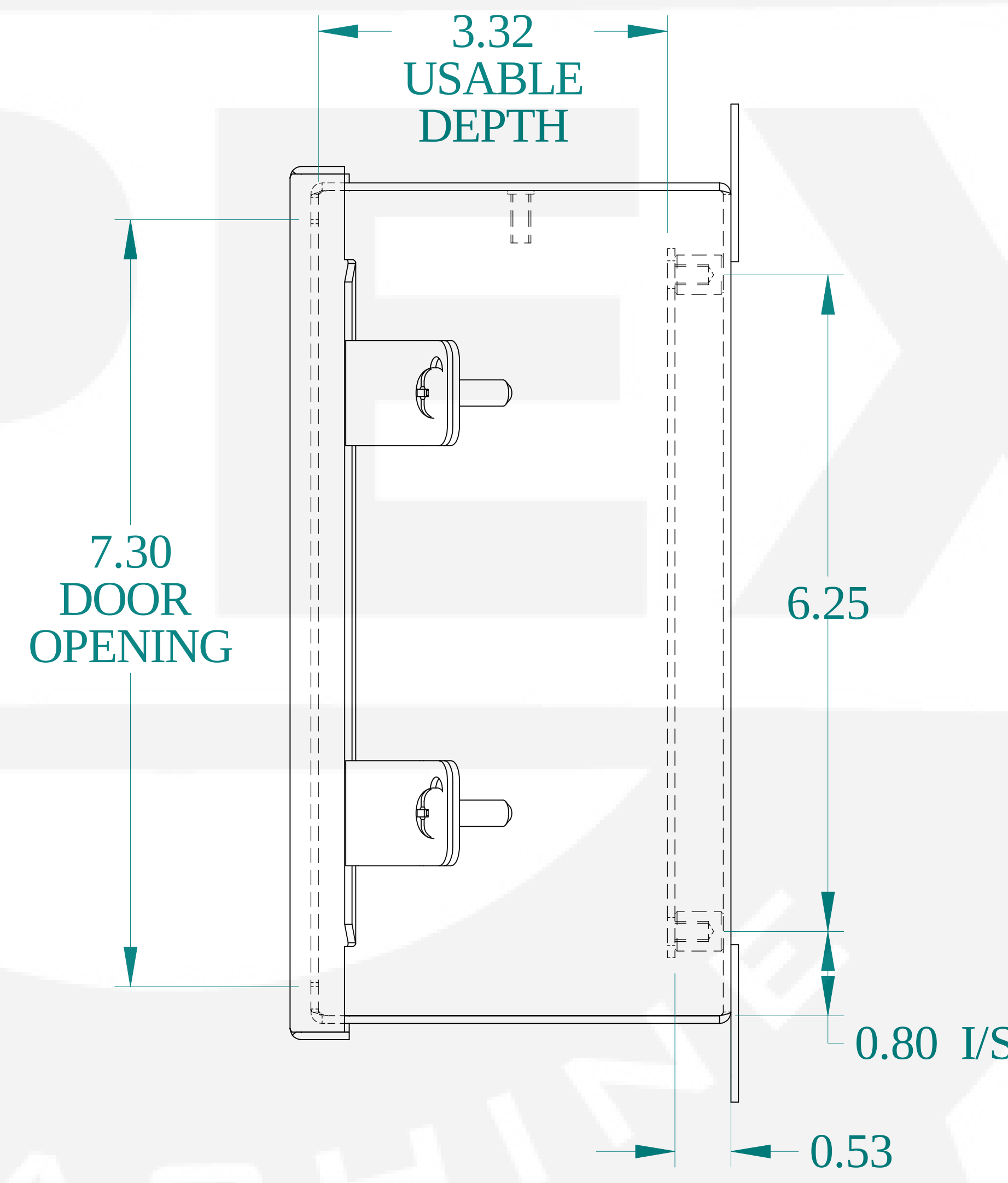
SIDE VIEW
