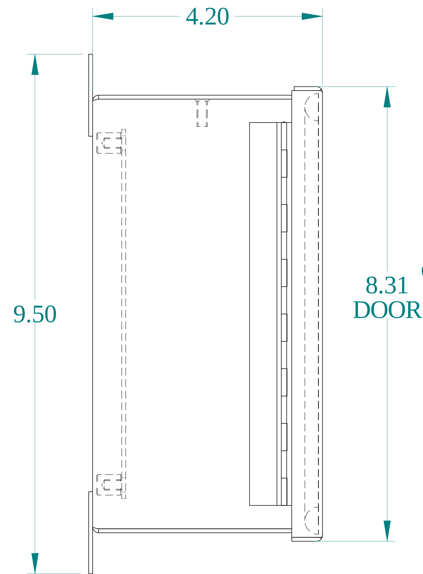
SIDE VIEW
