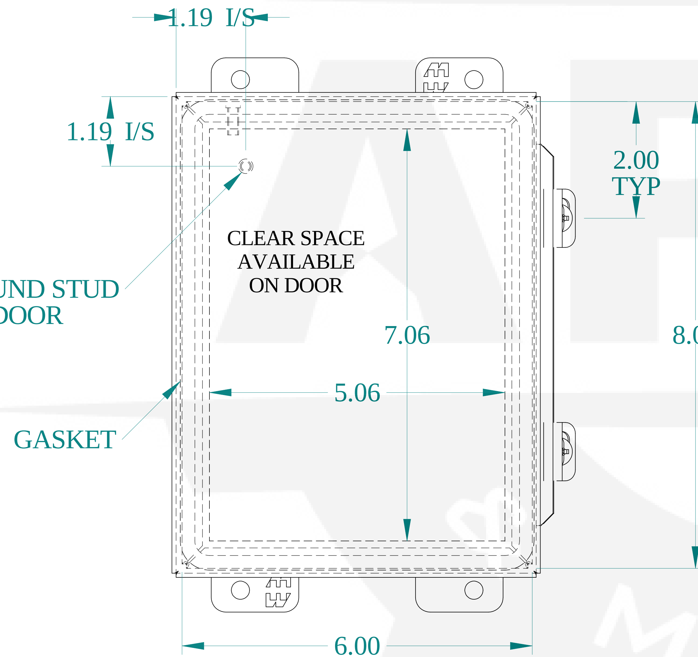
FRONT VIEW
