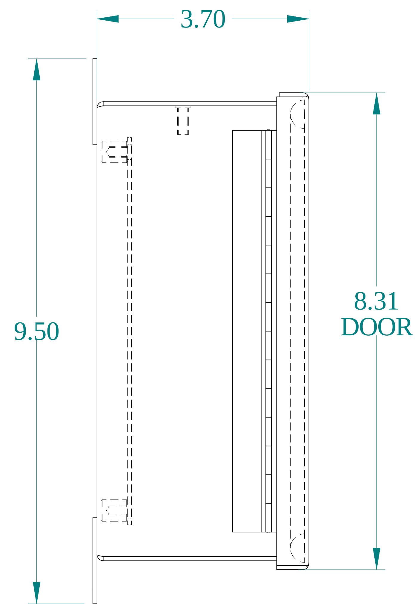
SIDE VIEW
