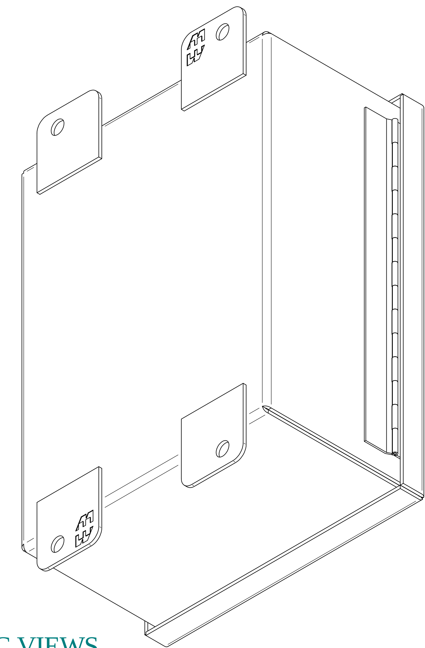
ISOMETRIC VIEWS
