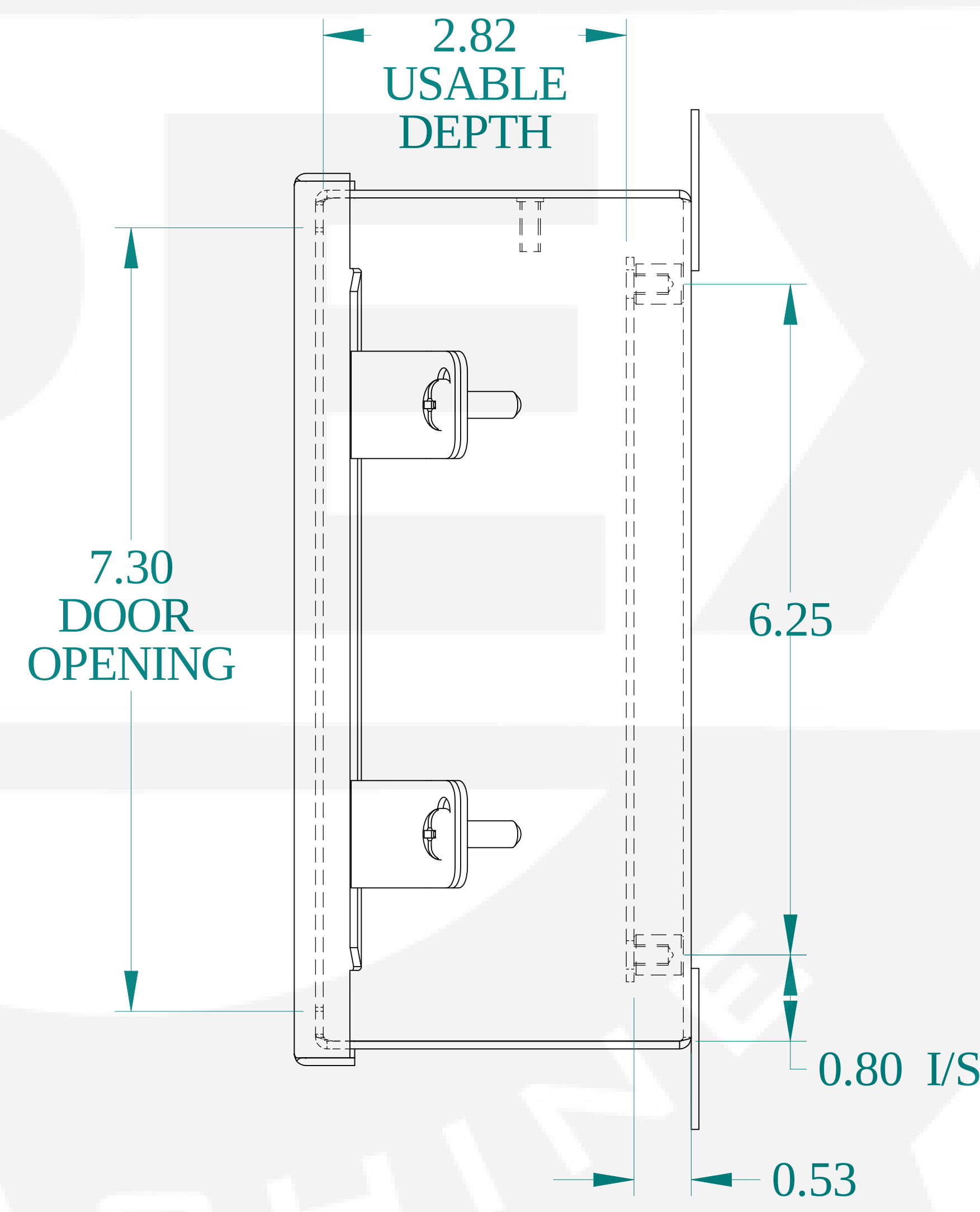
SIDE VIEW
