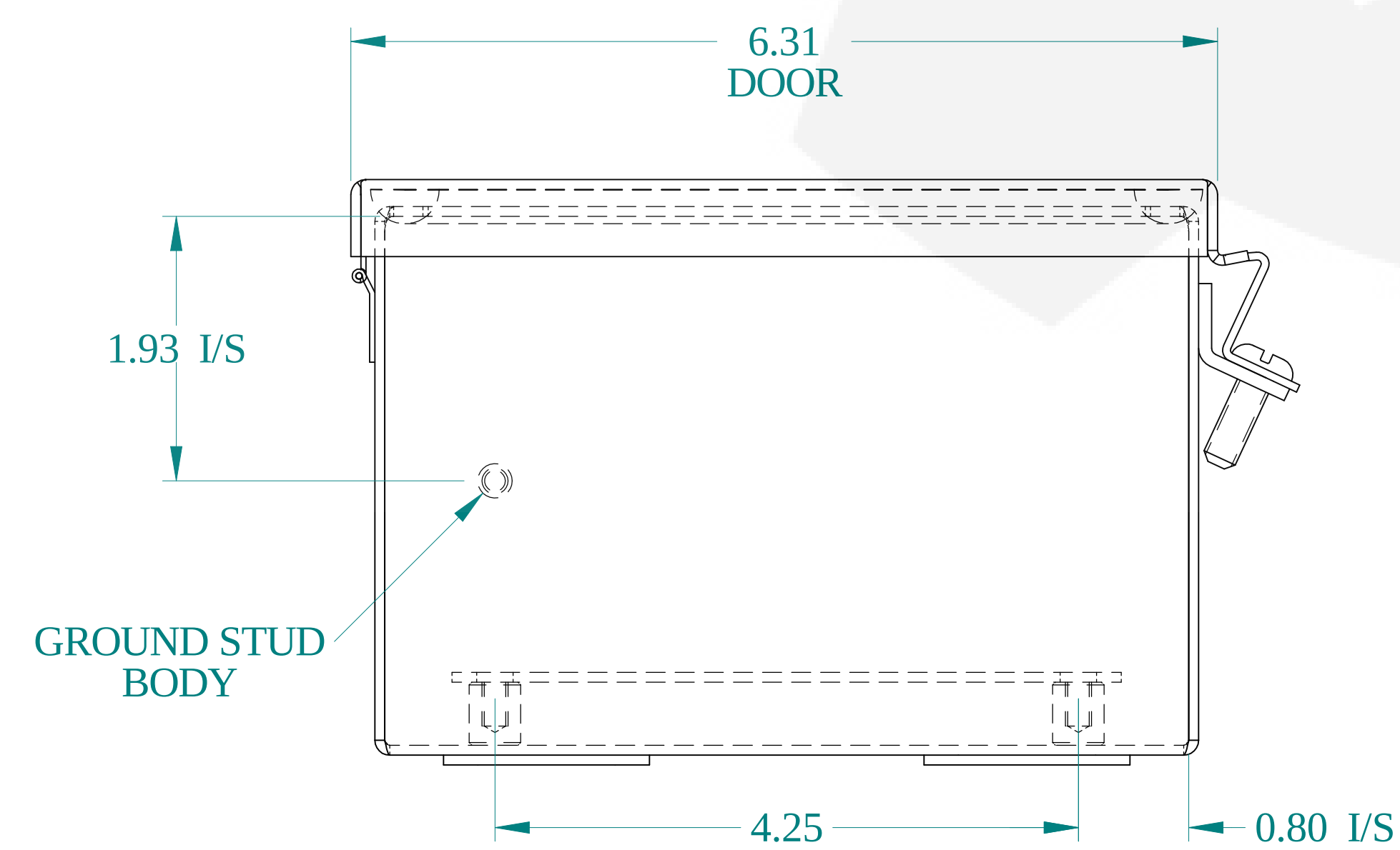
BOTTOM VIEW
