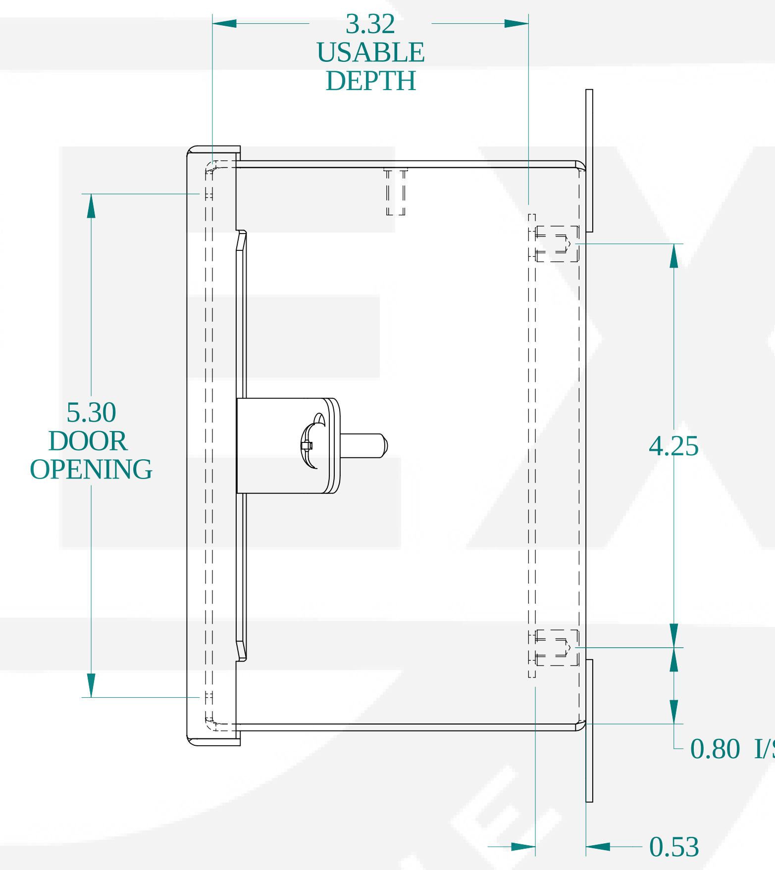
SIDE VIEW
