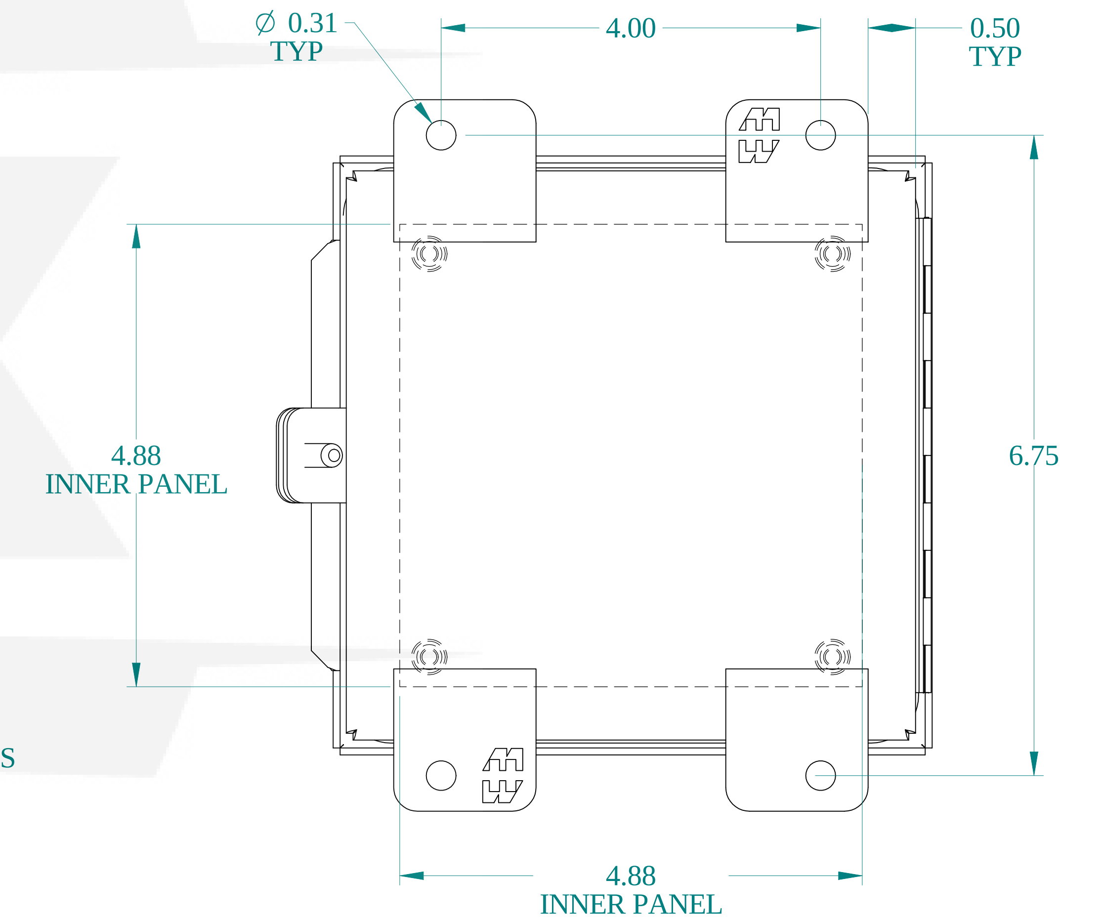
BACK VIEW
