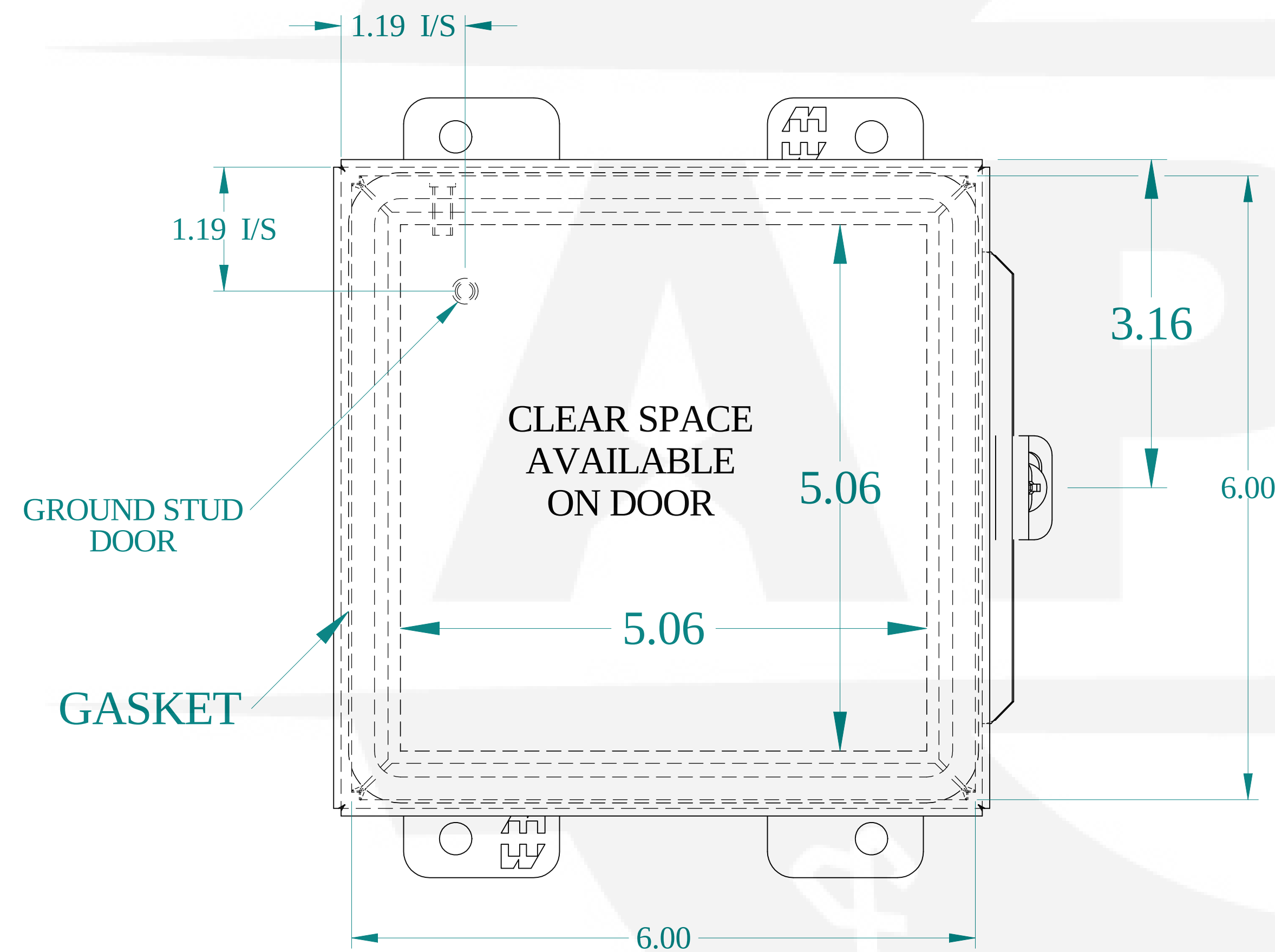
FRONT VIEW
