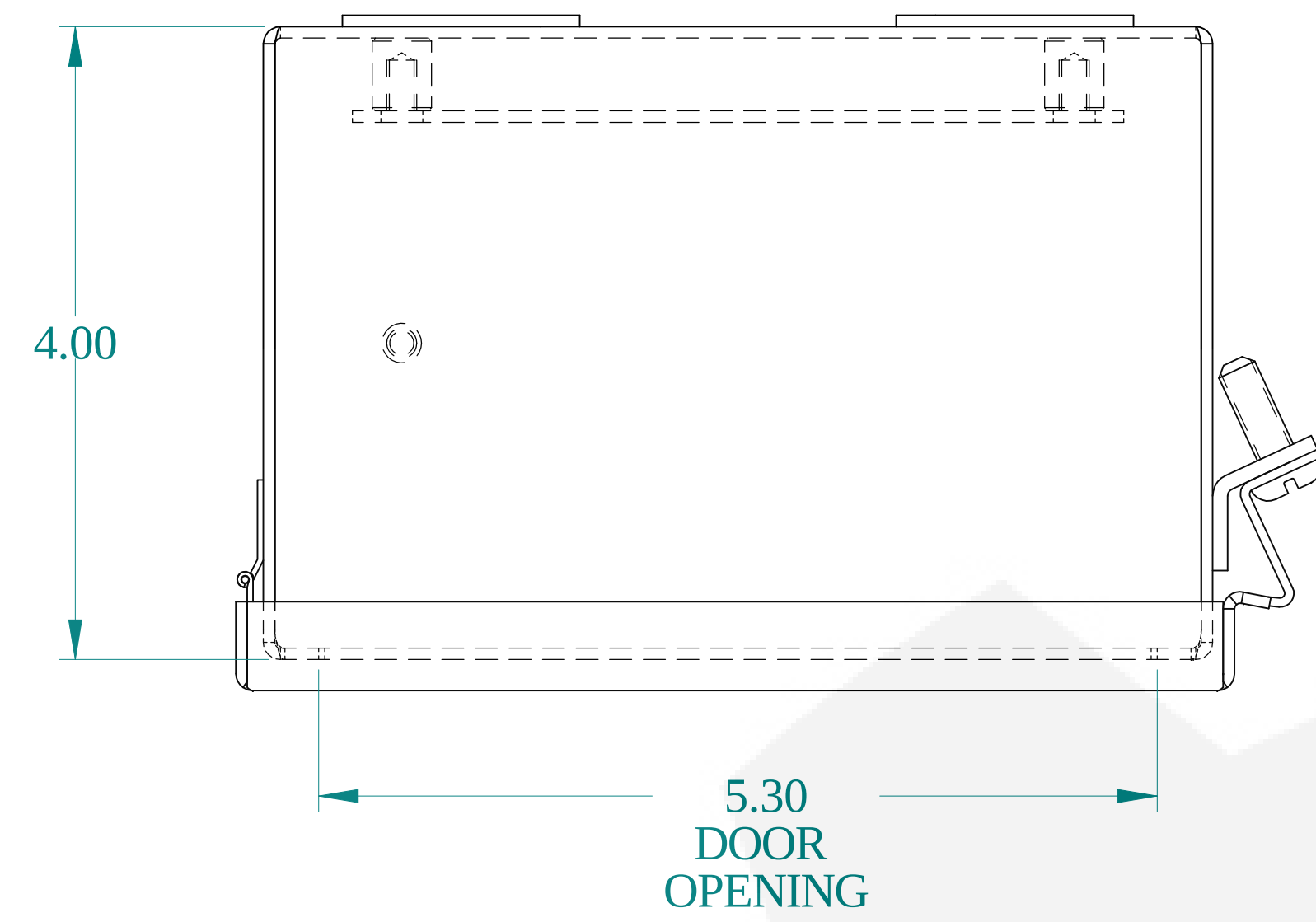
TOP VIEW
