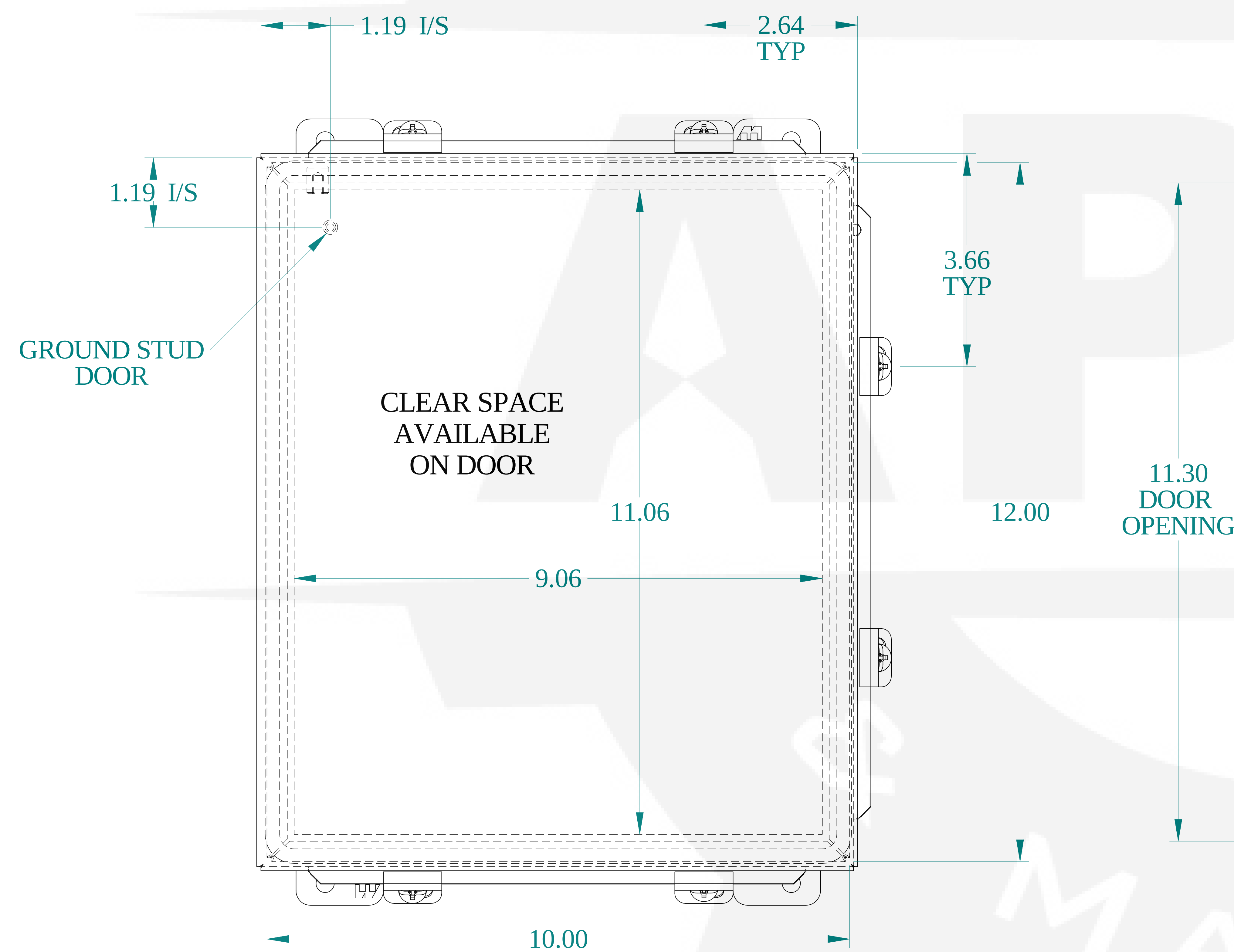
FRONT VIEW
