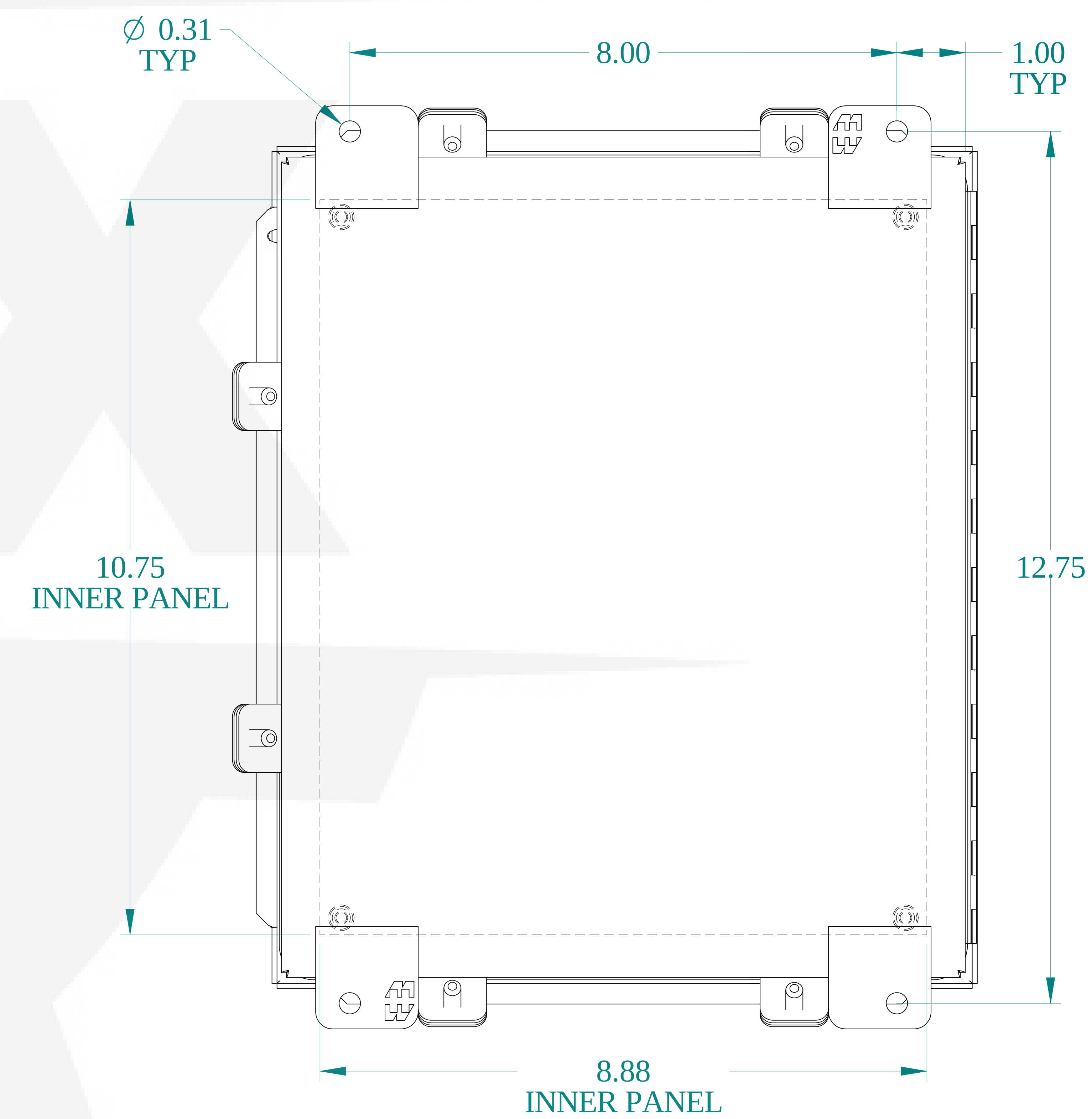
BACK VIEW
