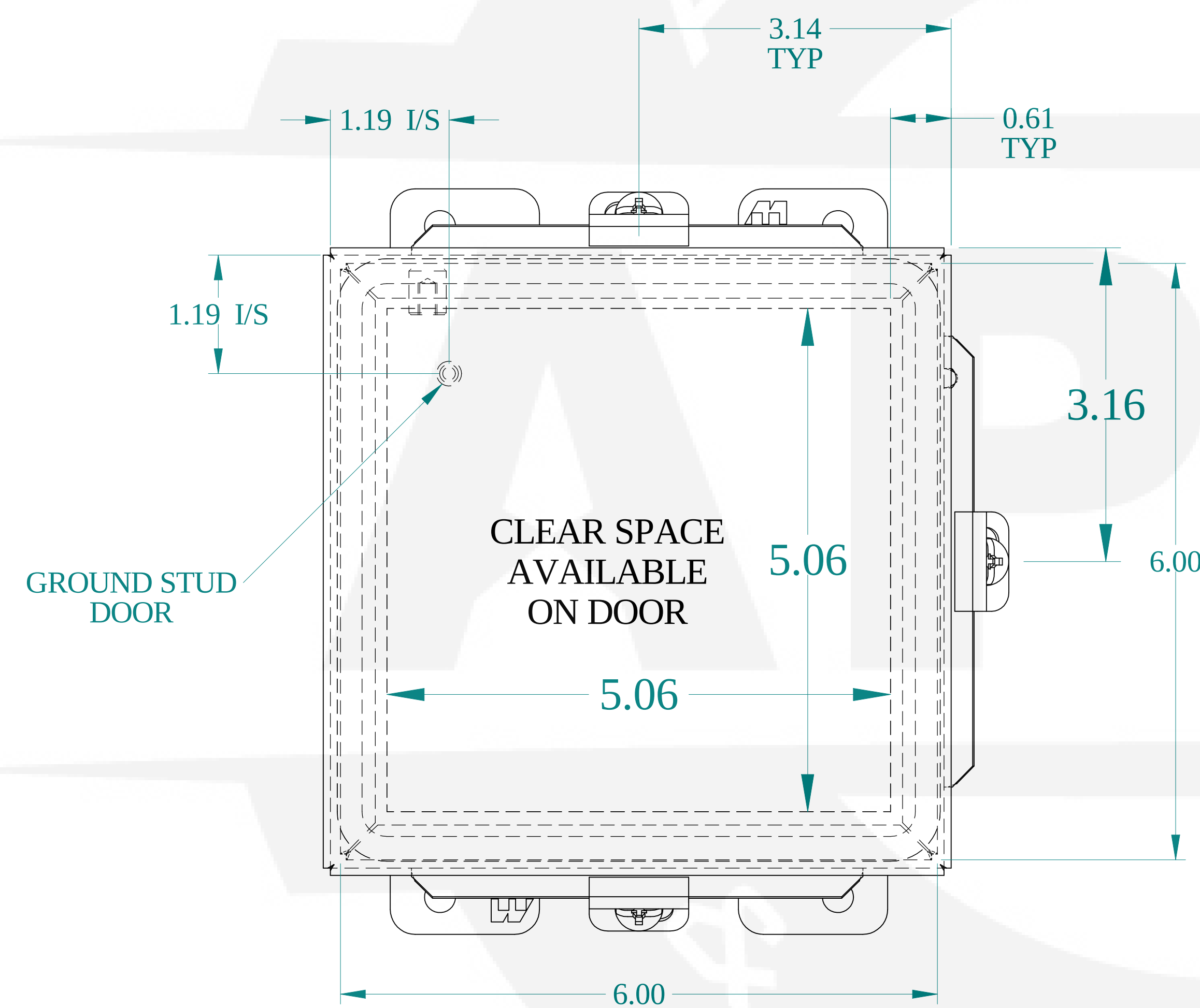
FRONT VIEW
