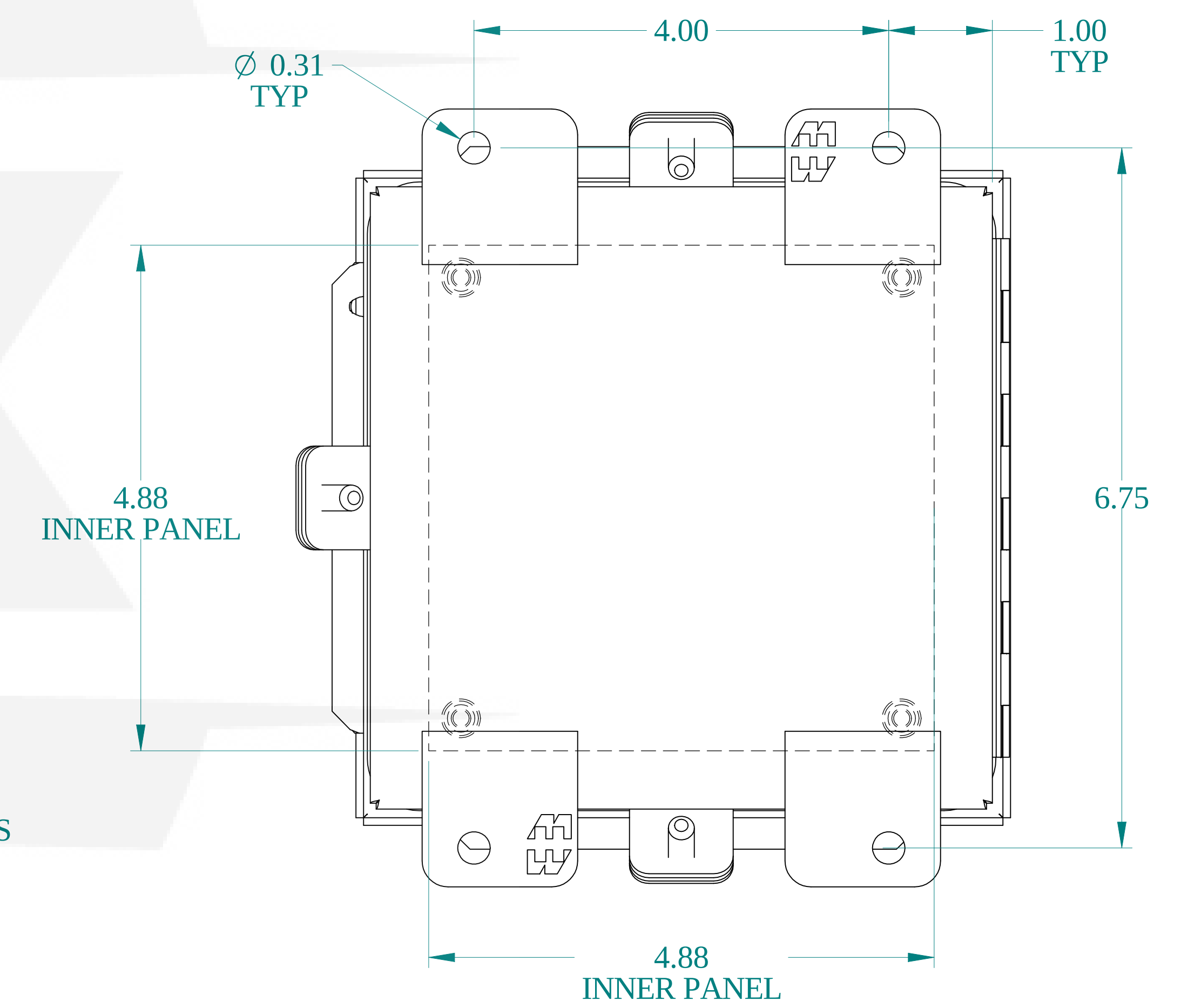
BACK VIEW
