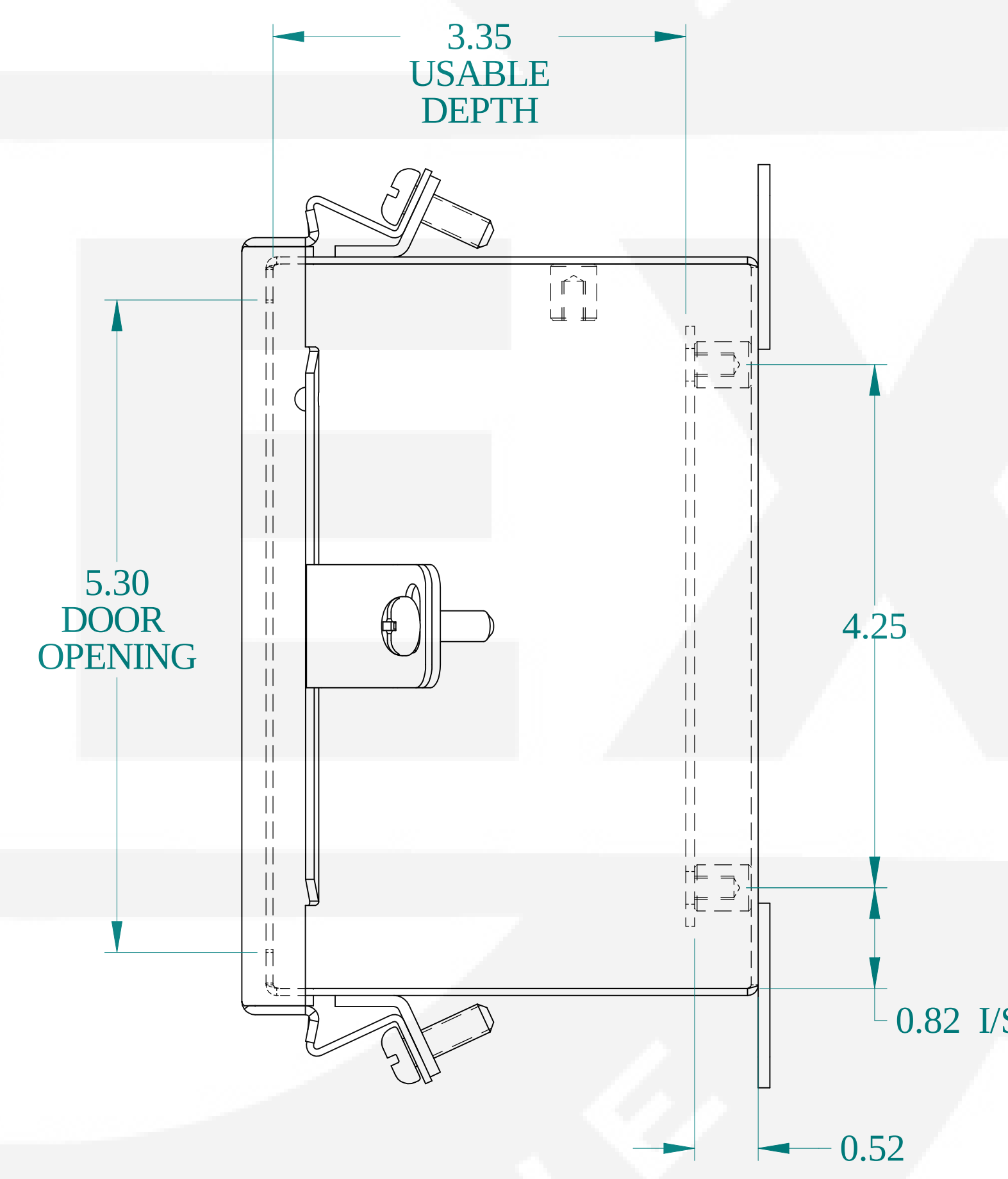
SIDE VIEW
