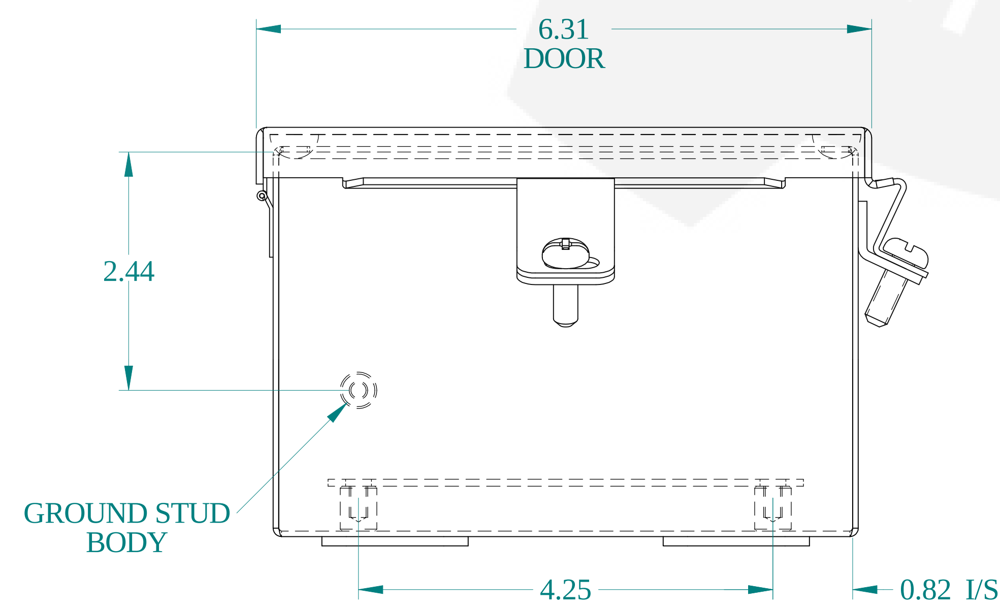
BOTTOM VIEW
