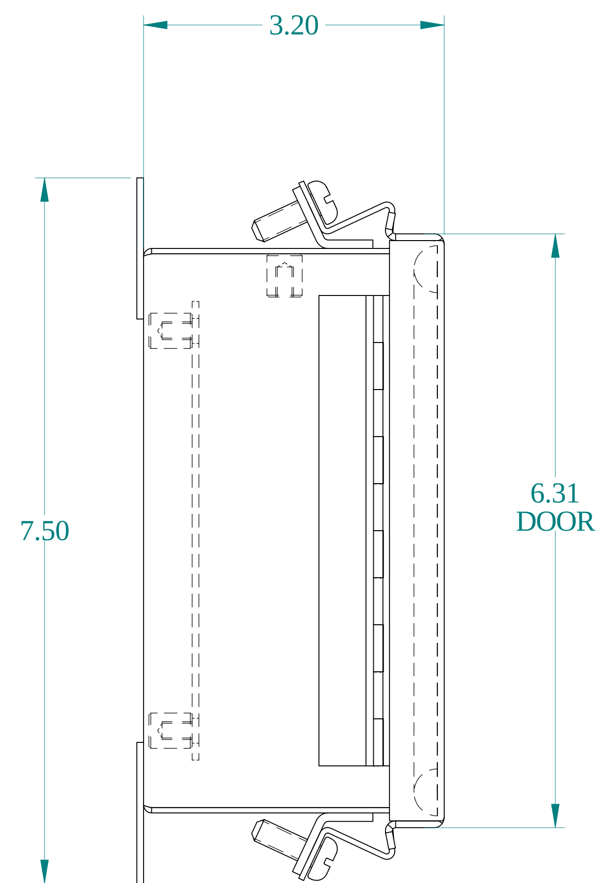
SIDE VIEW
