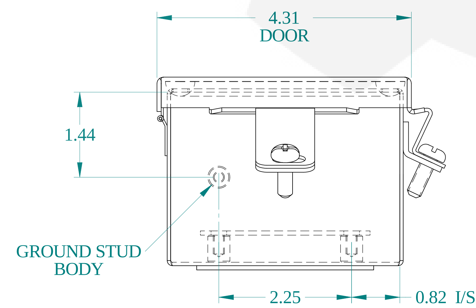
BOTTOM VIEW
