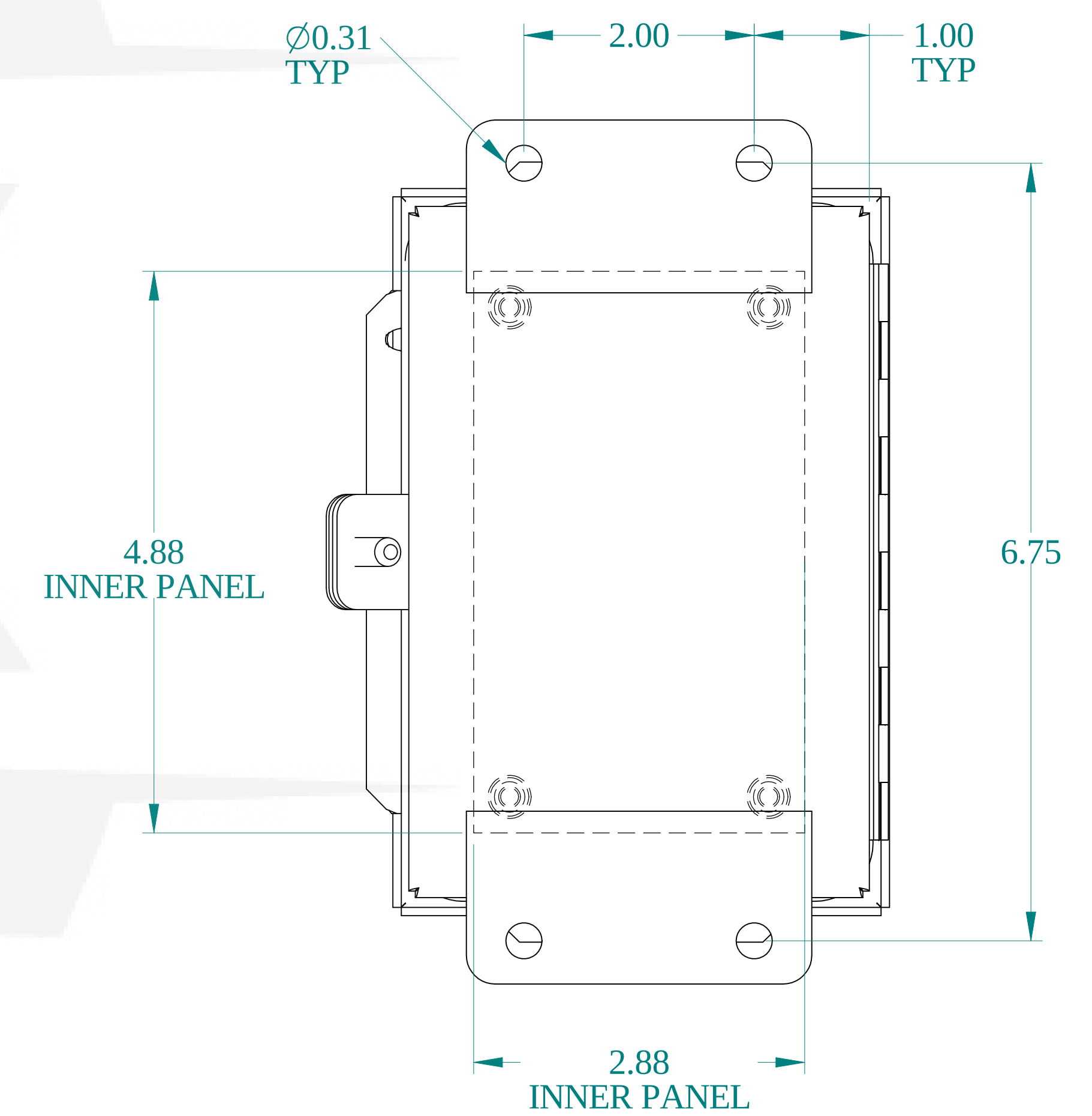
BACK VIEW
