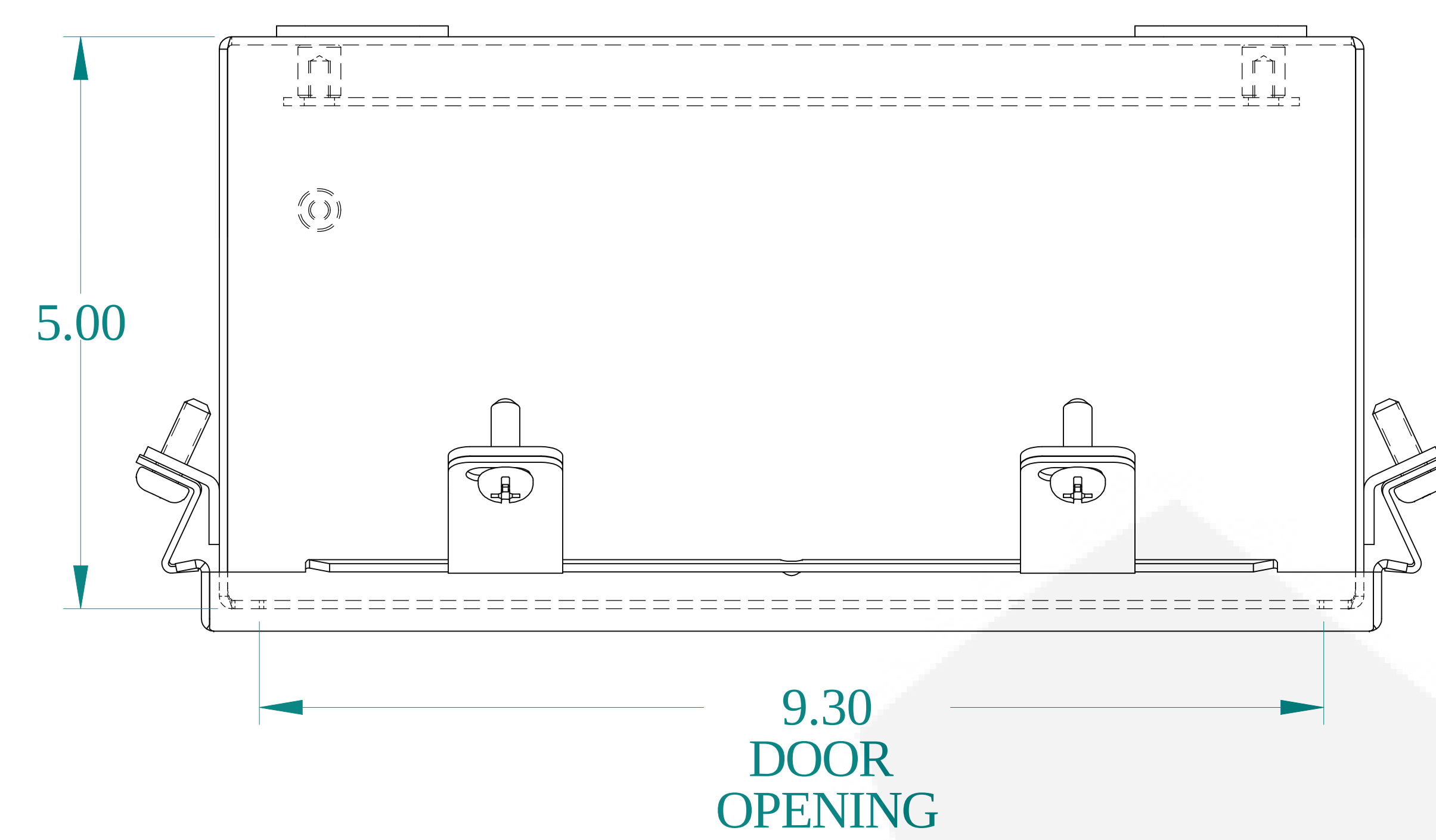
TOP VIEW
