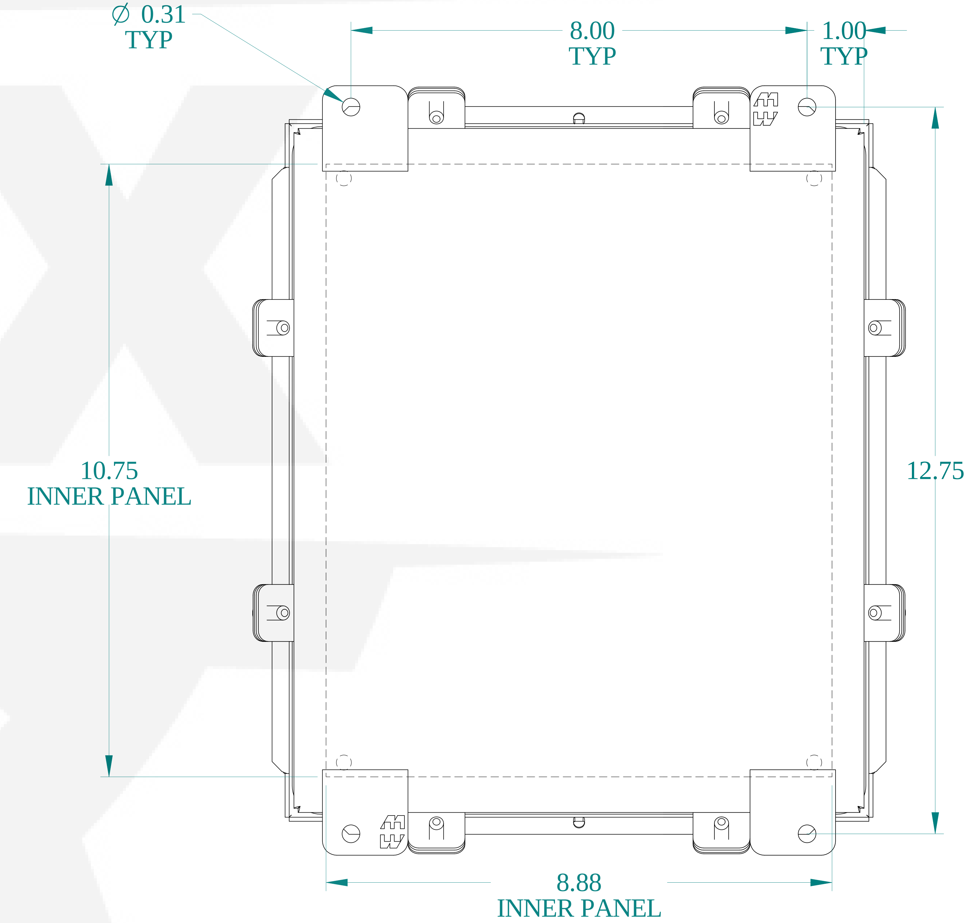
BACK VIEW
