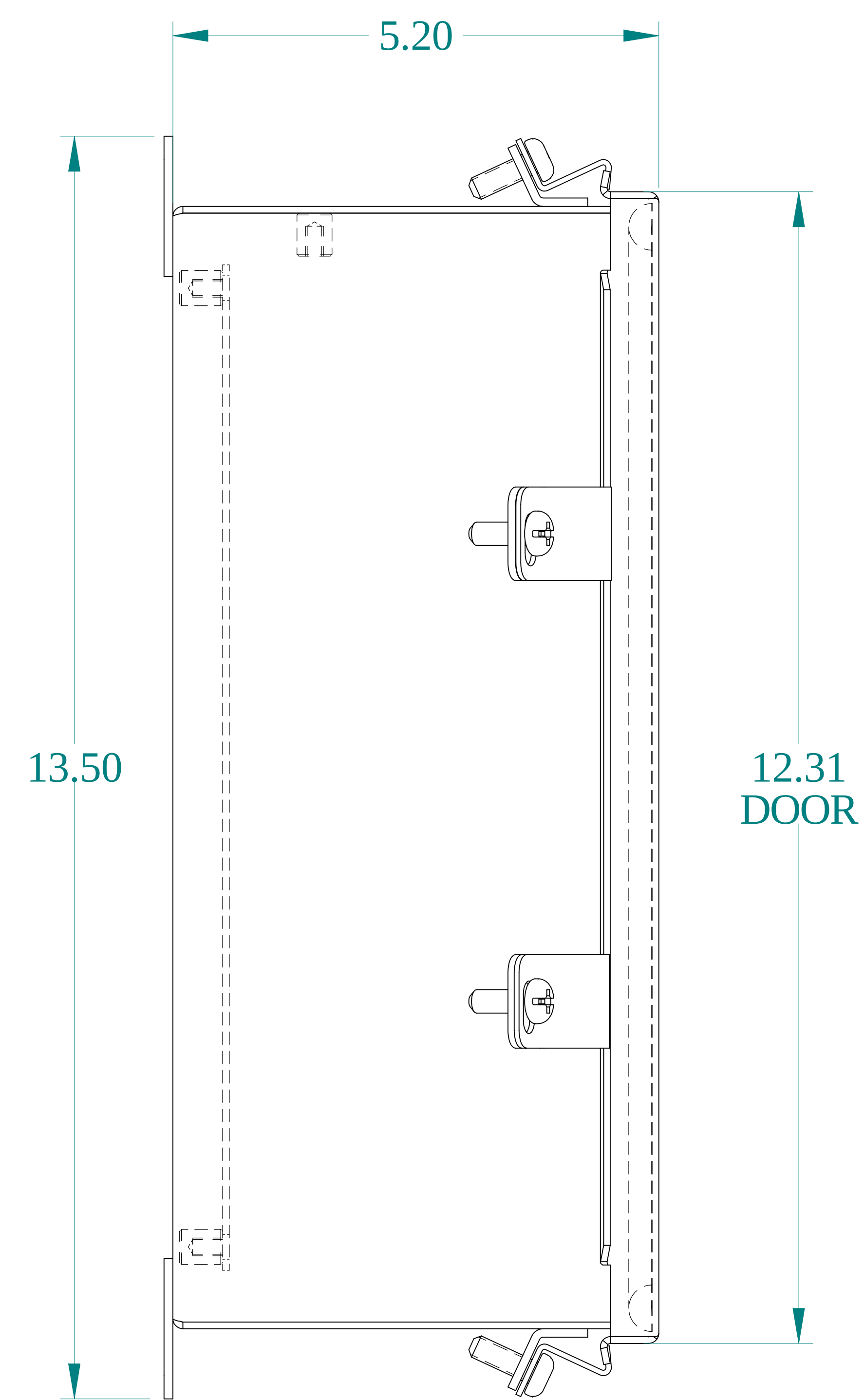
SIDE VIEW
