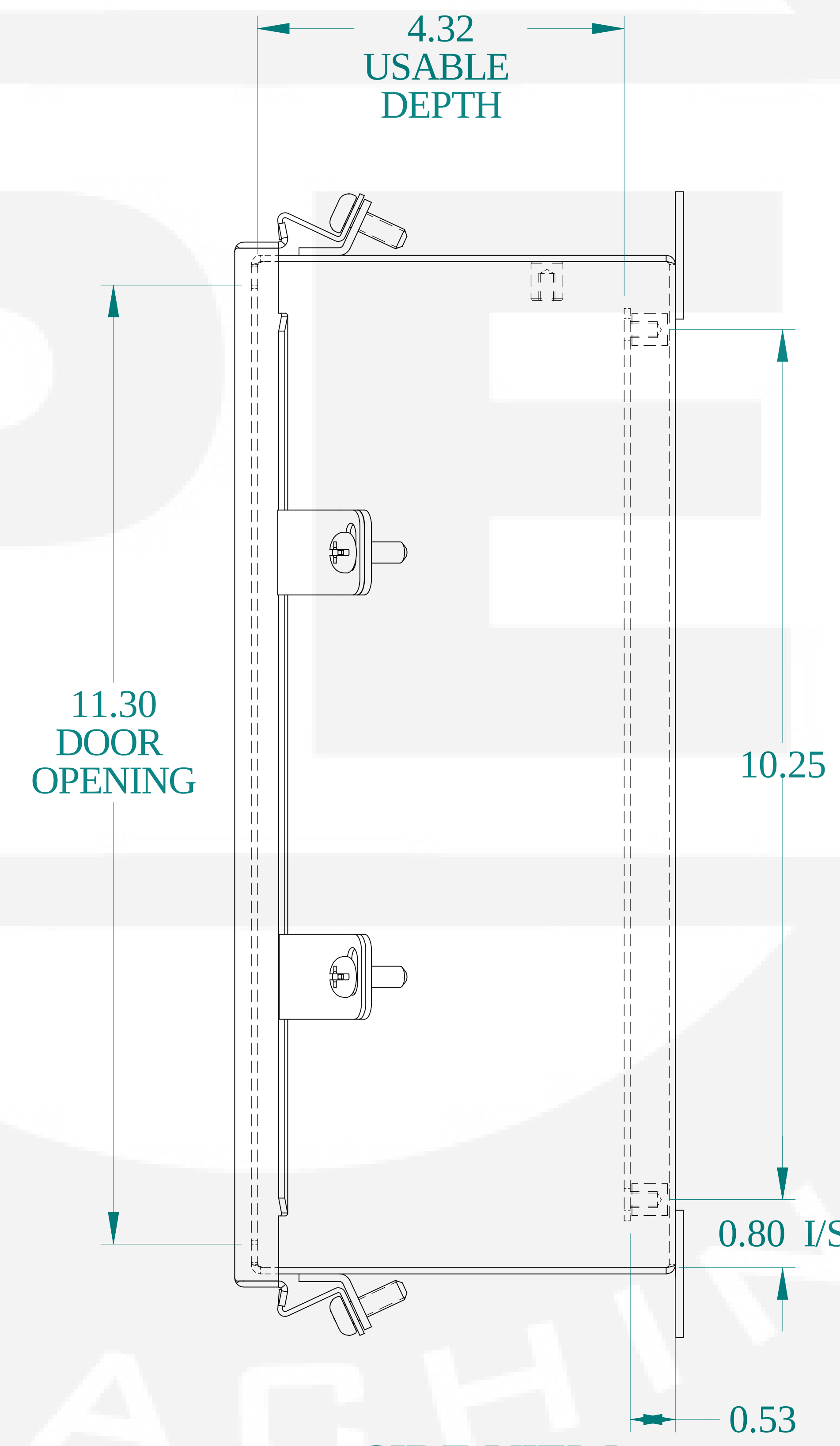
SIDE VIEW
