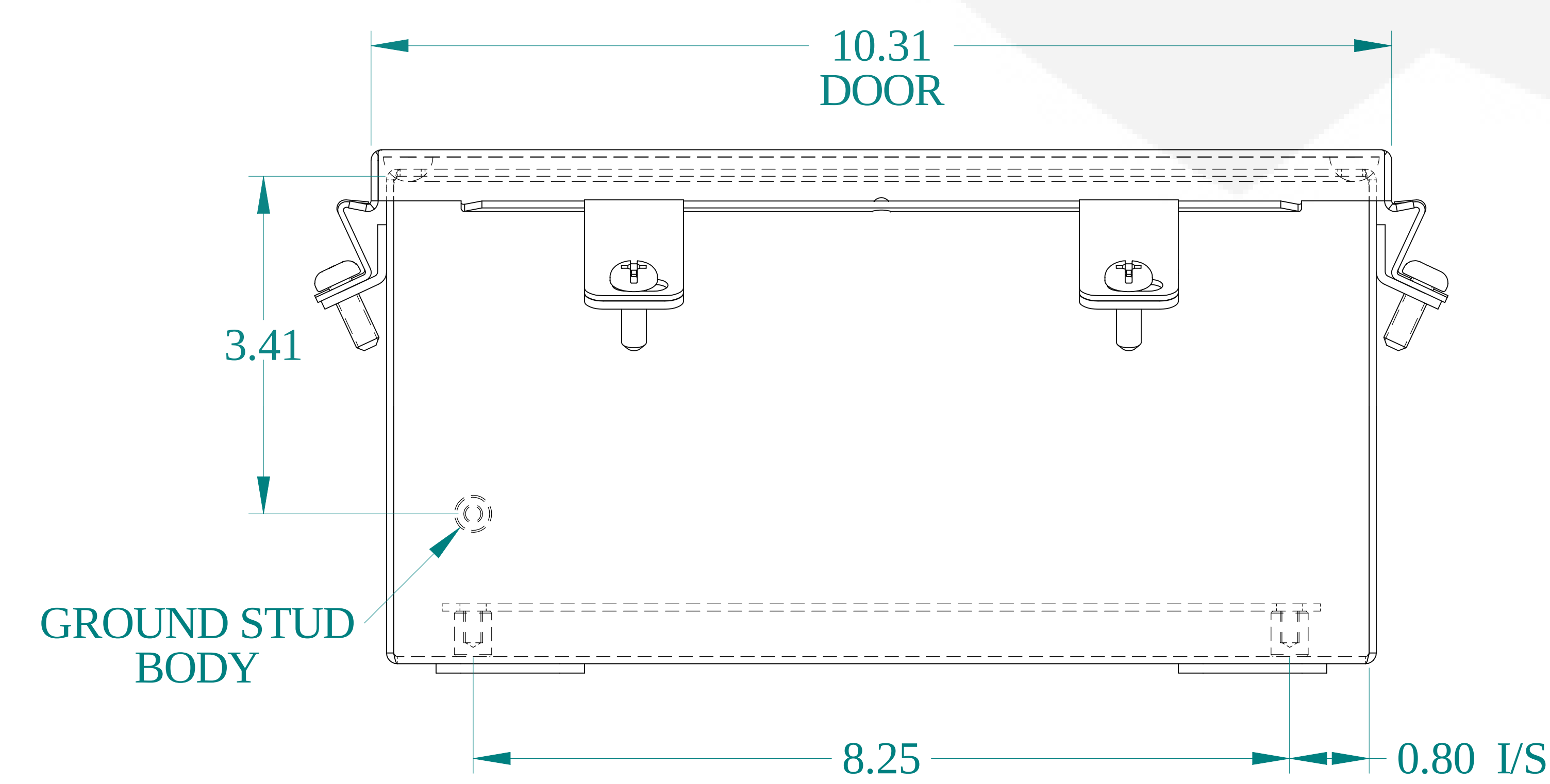
BOTTOM VIEW
