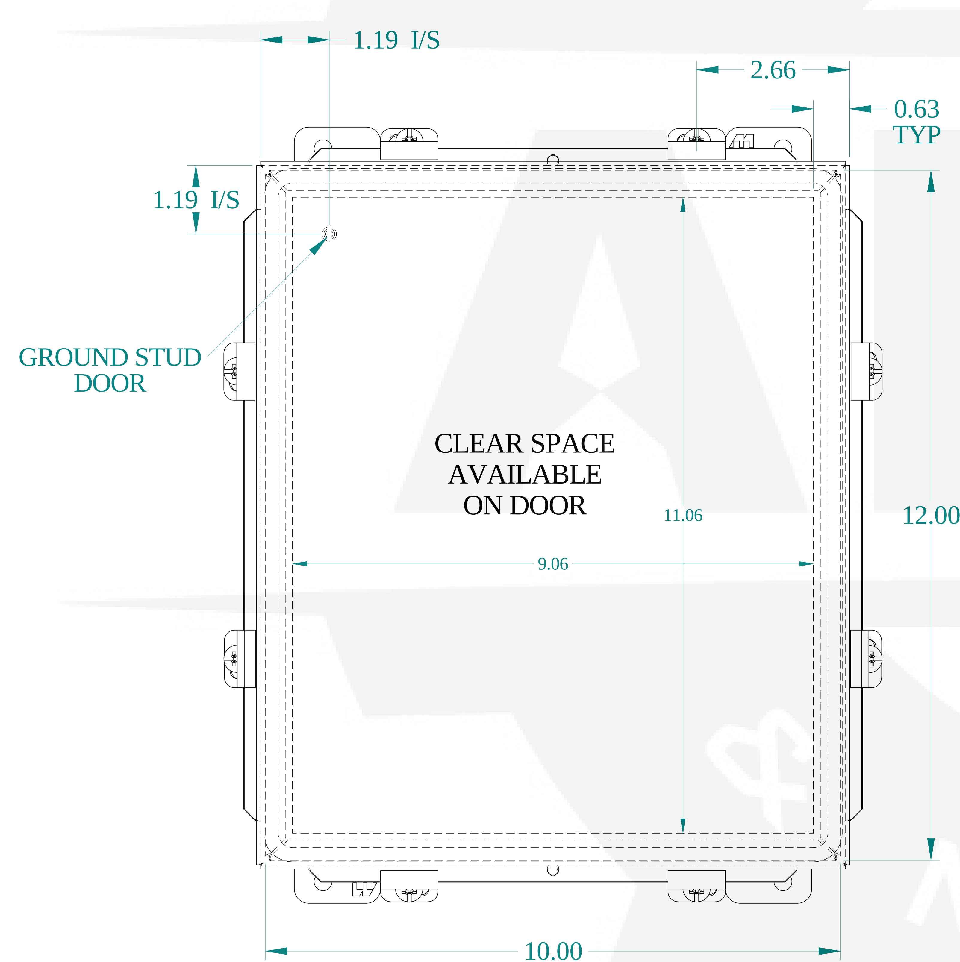
FRONT VIEW
