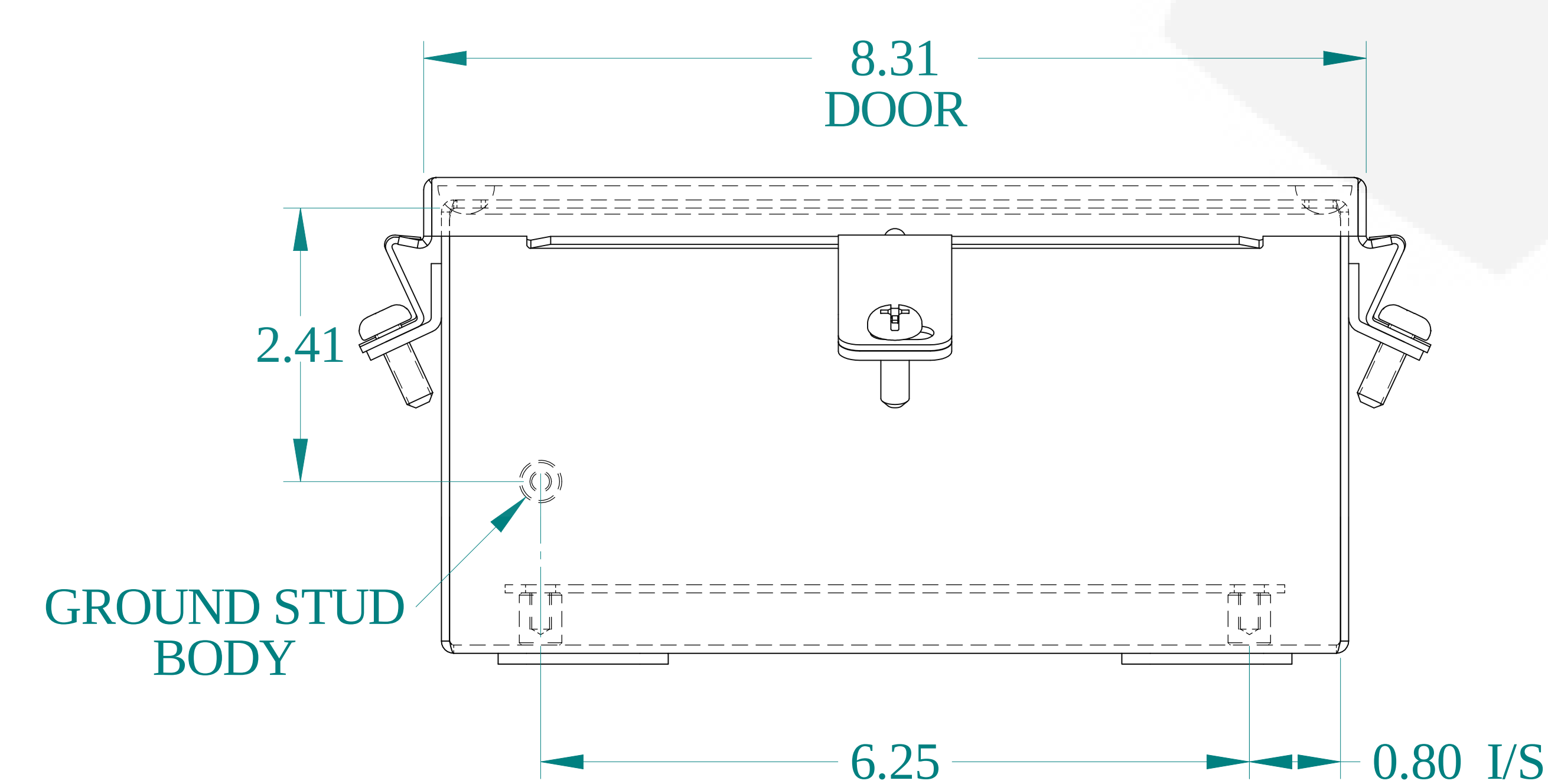
BOTTOM VIEW
