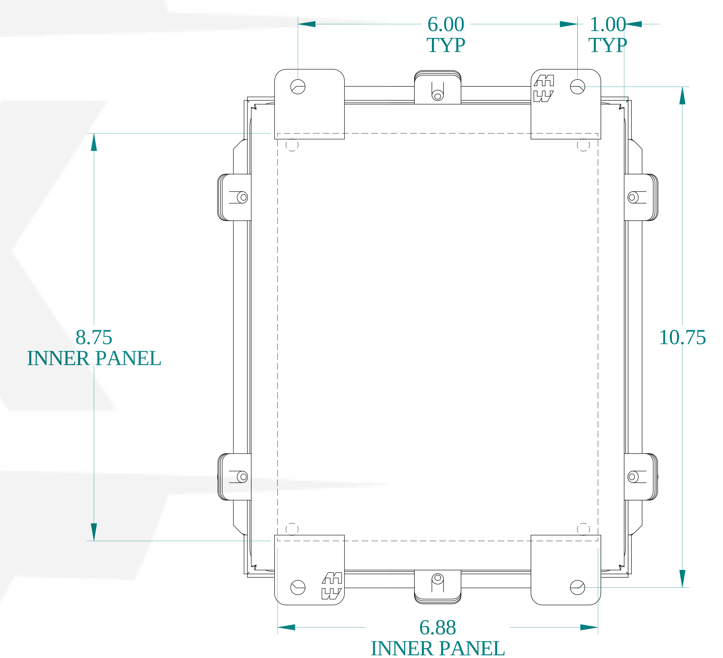
BACK VIEW
