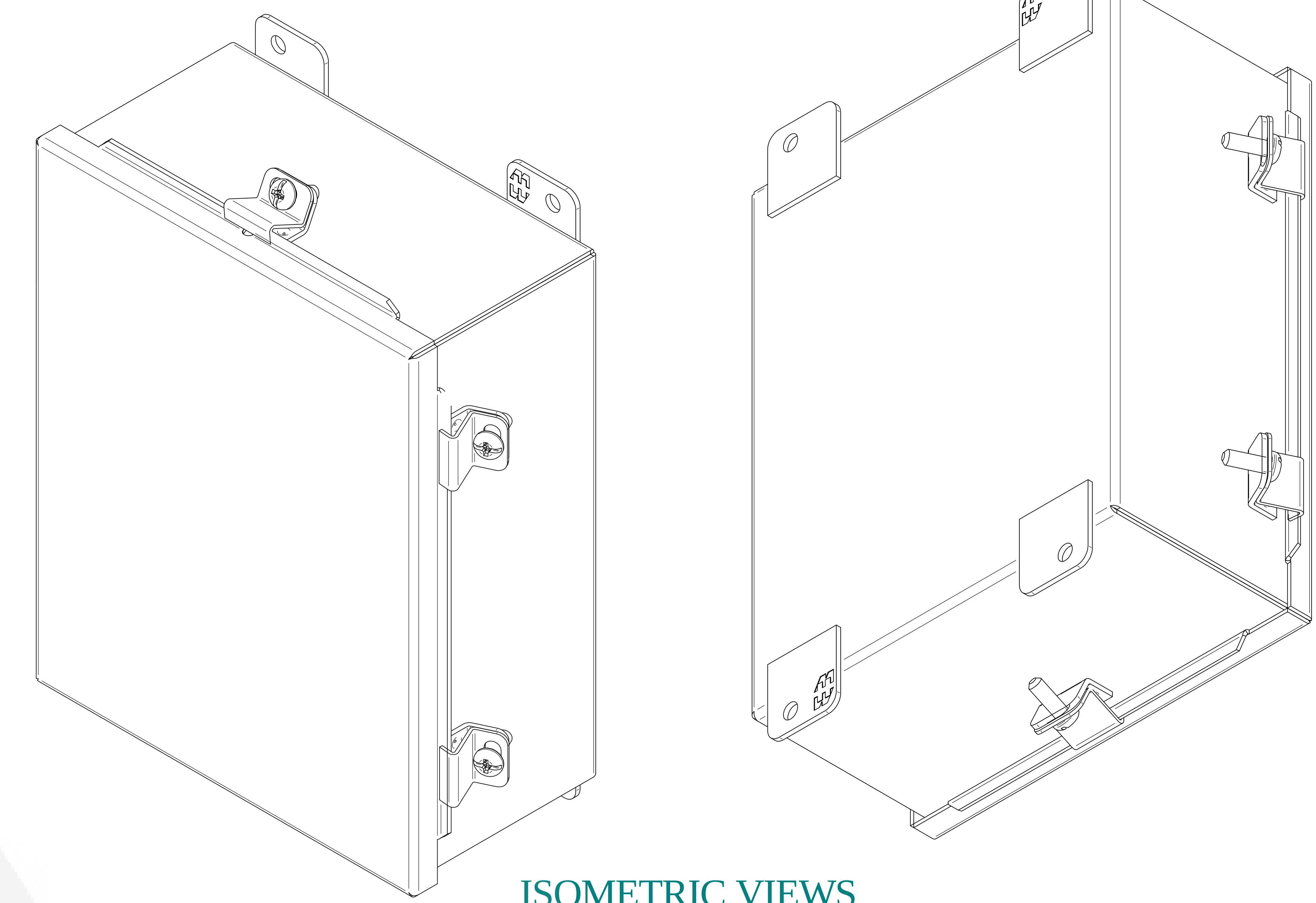
ISOMETRIC VIEWS
