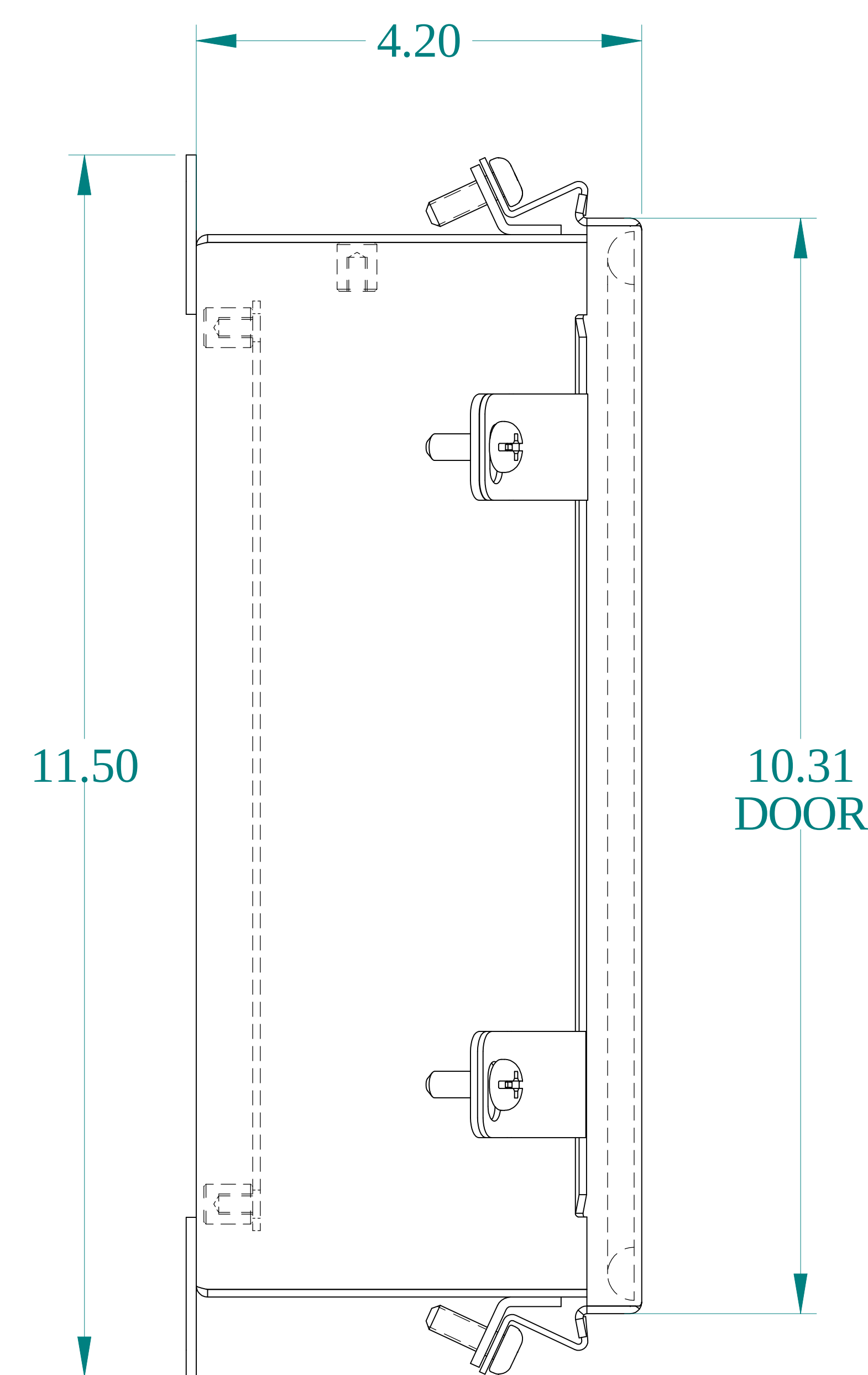
SIDE VIEW
