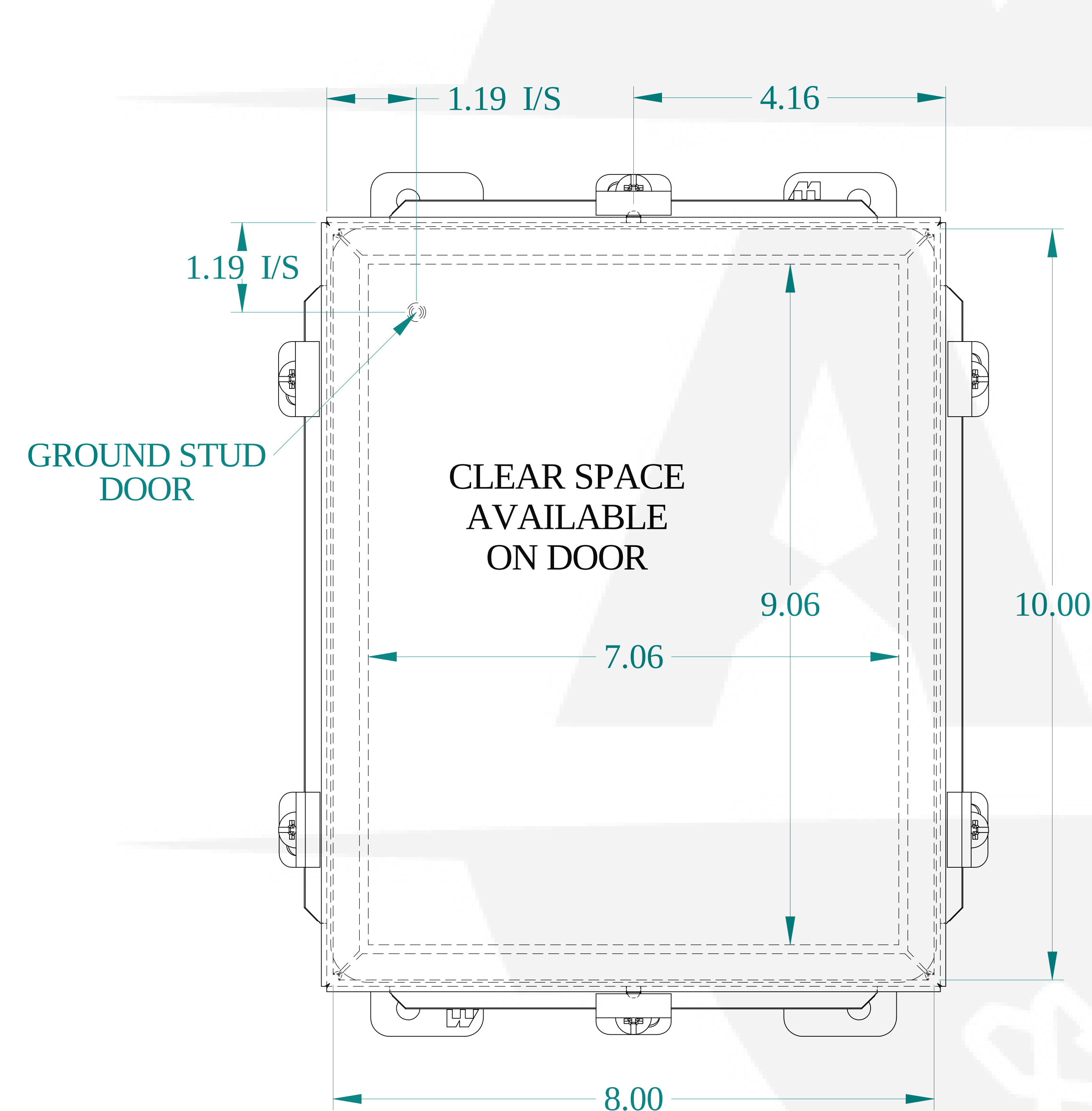
FRONT VIEW
