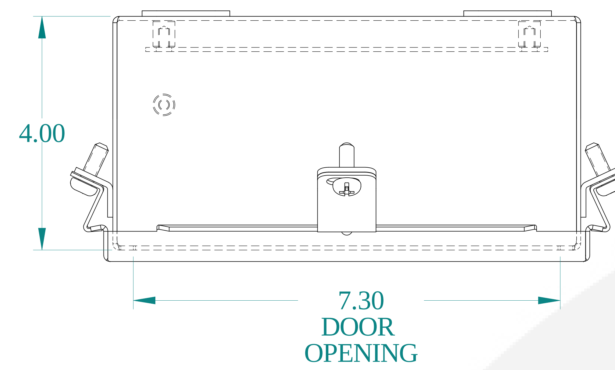
TOP VIEW
