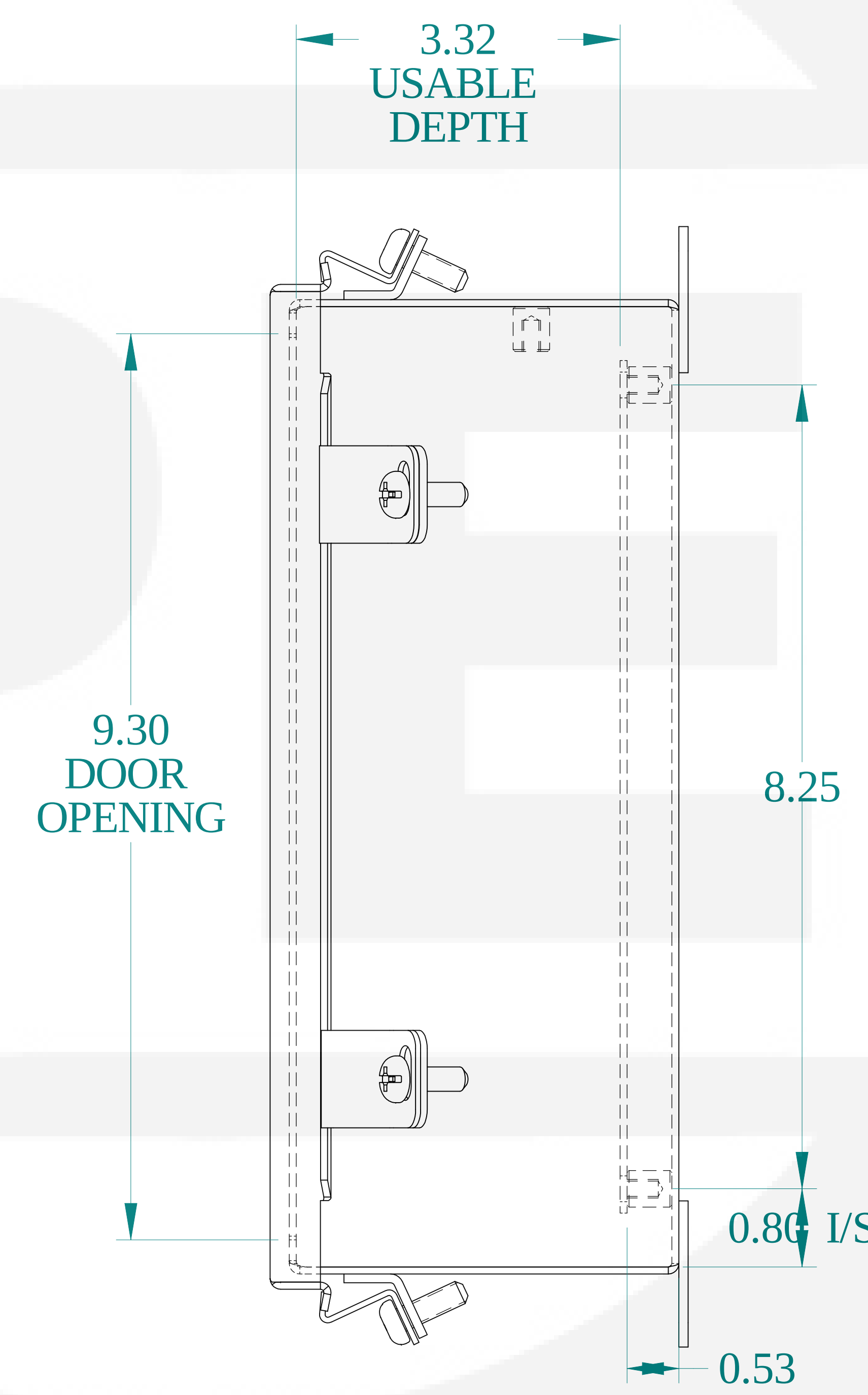
SIDE VIEW
