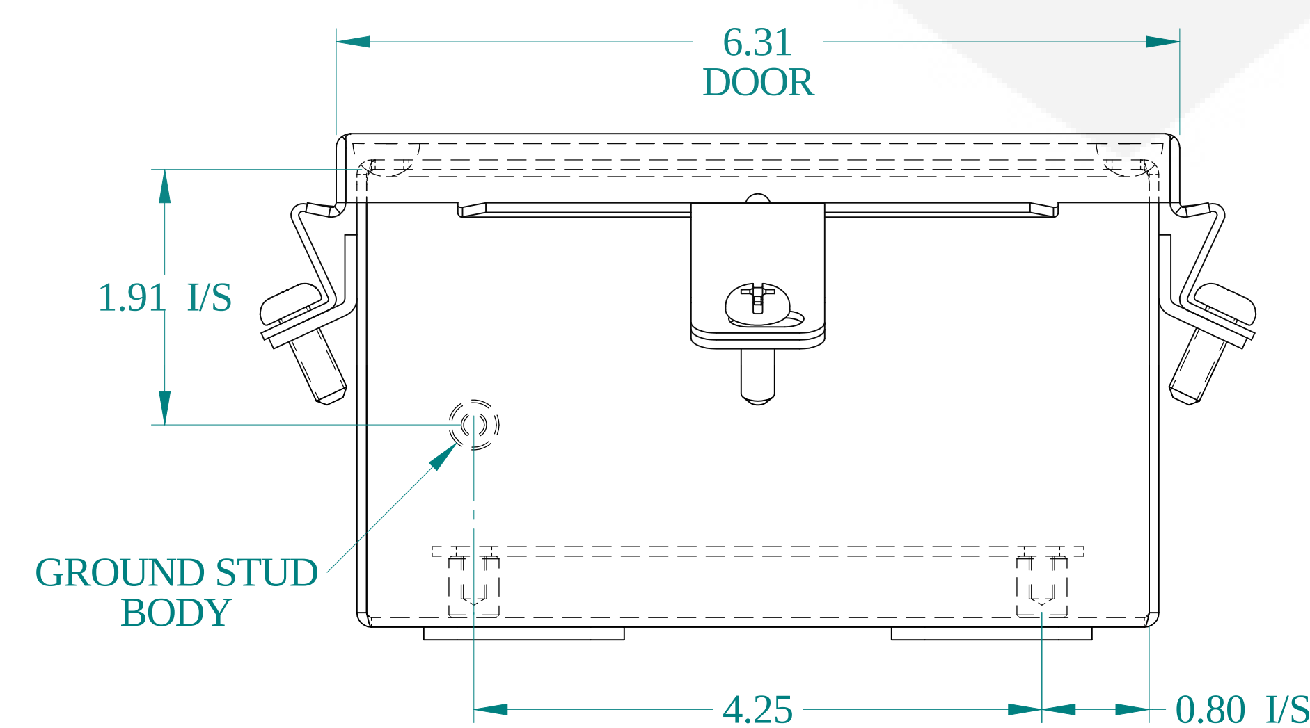
BOTTOM VIEW
