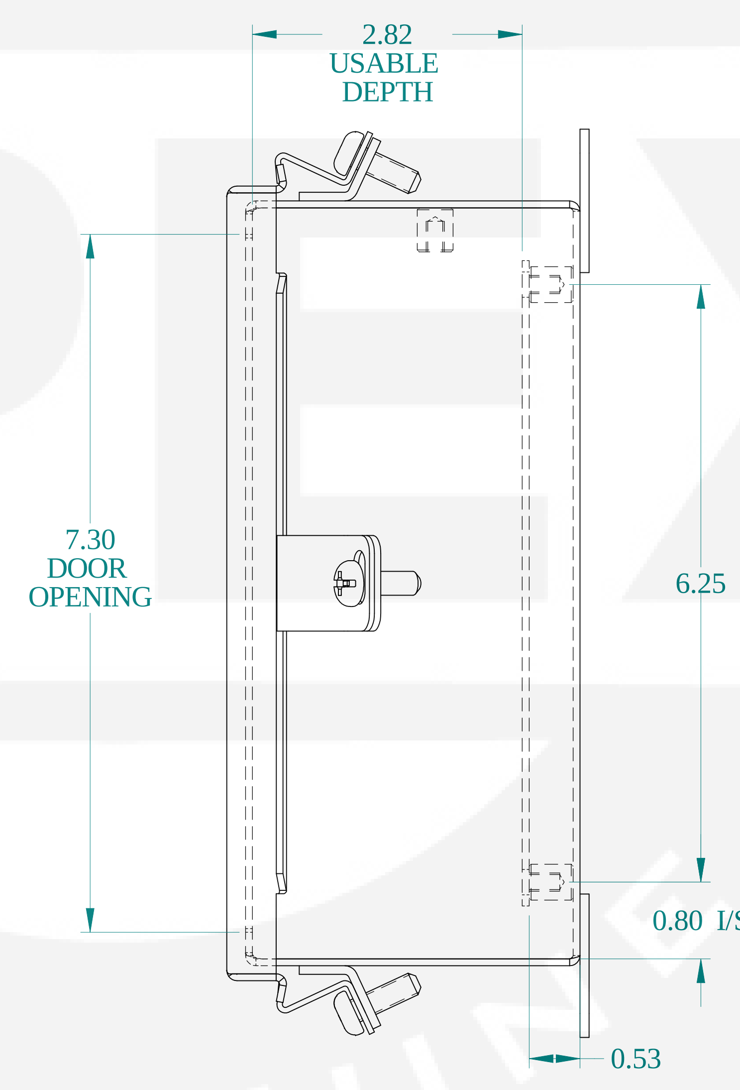
SIDE VIEW
