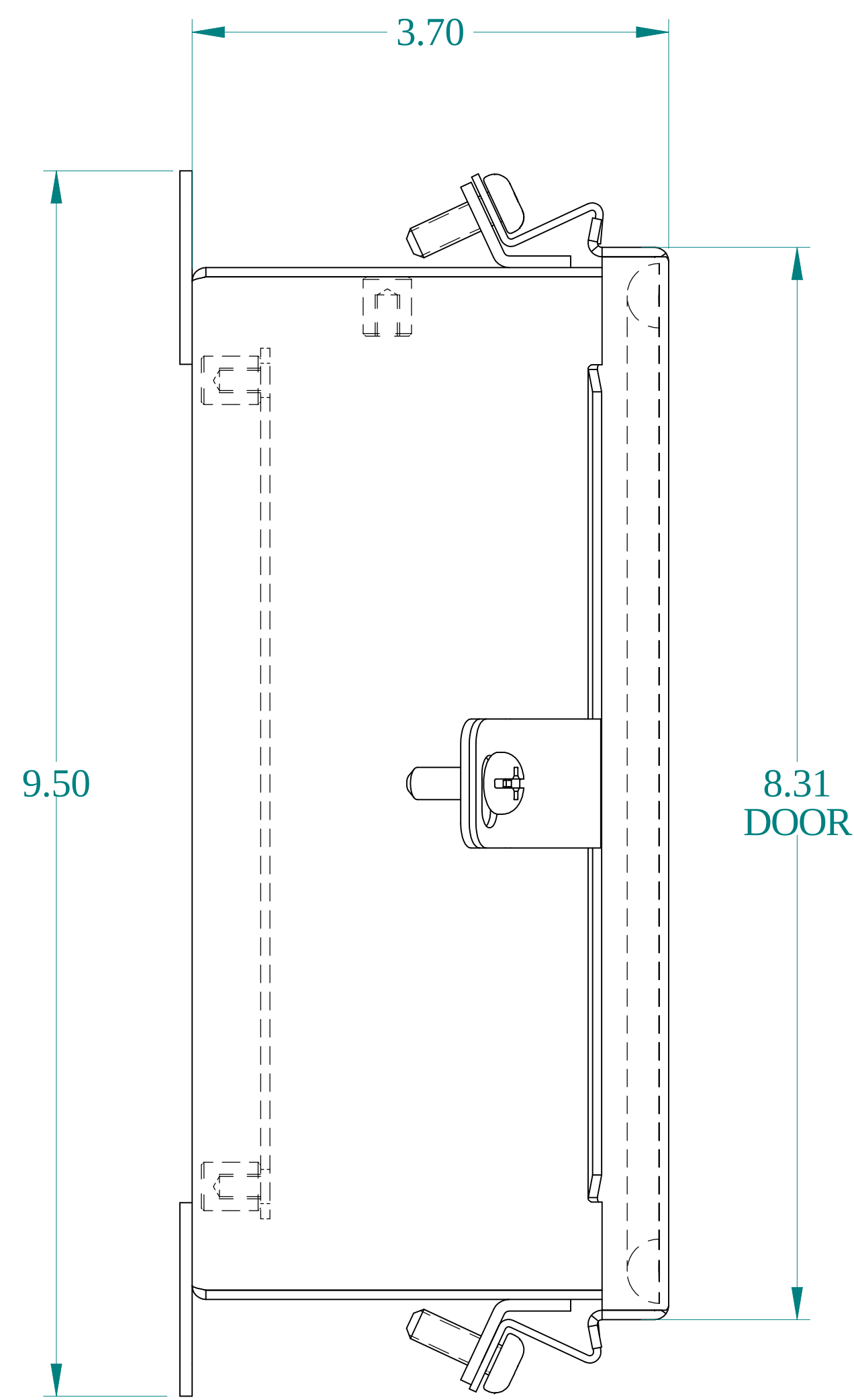
SIDE VIEW
