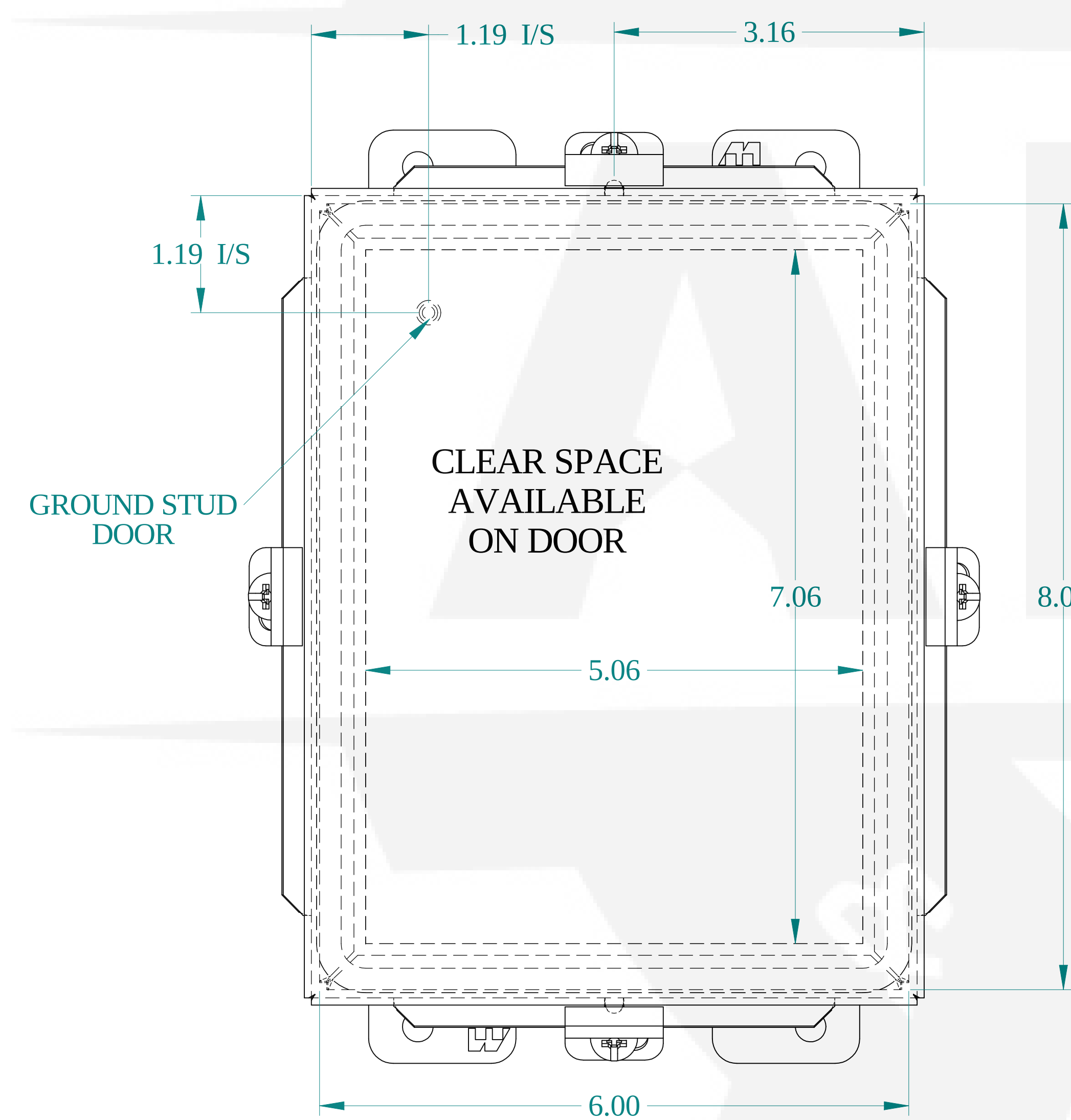
FRONT VIEW
