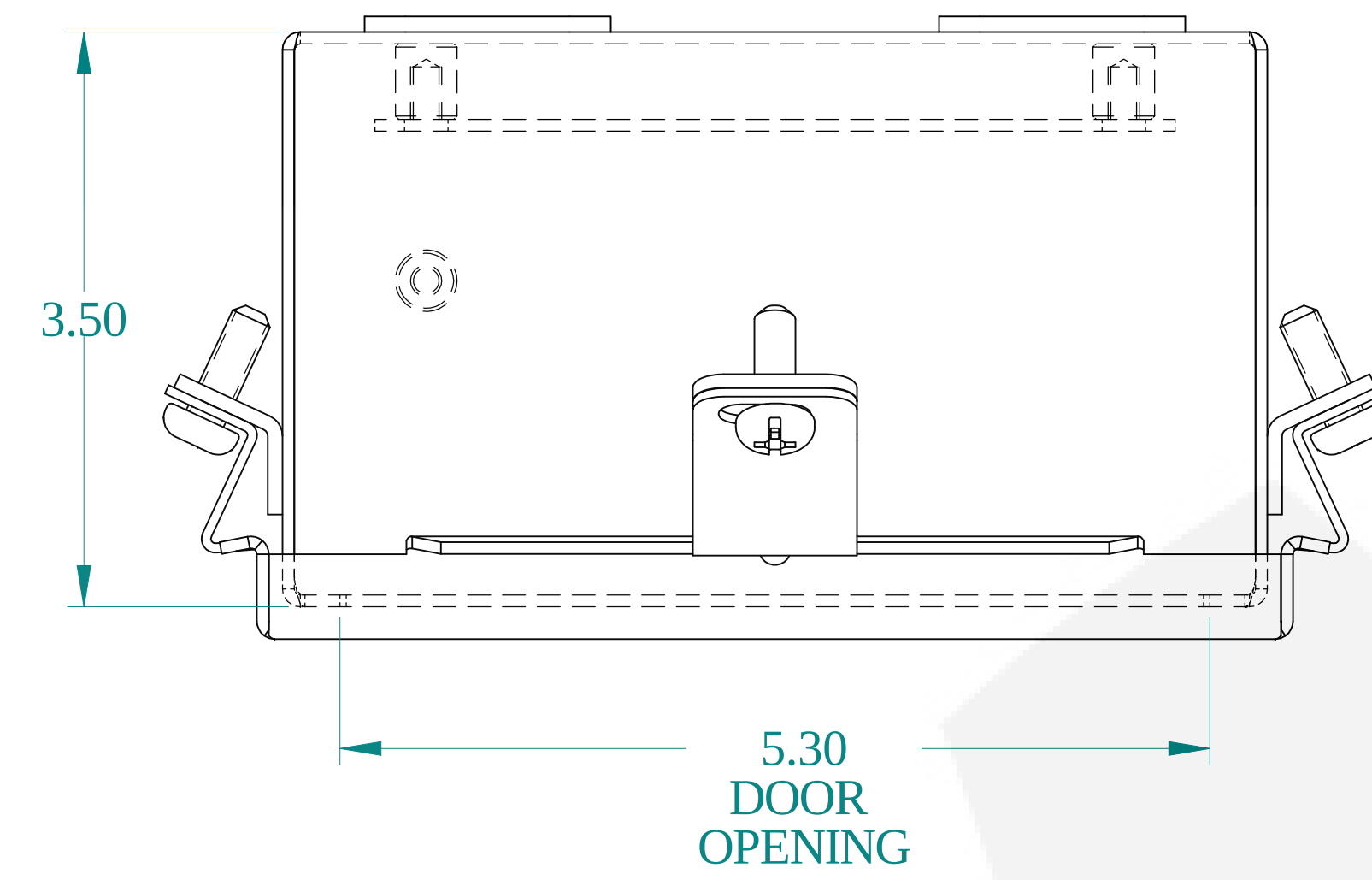
TOP VIEW
