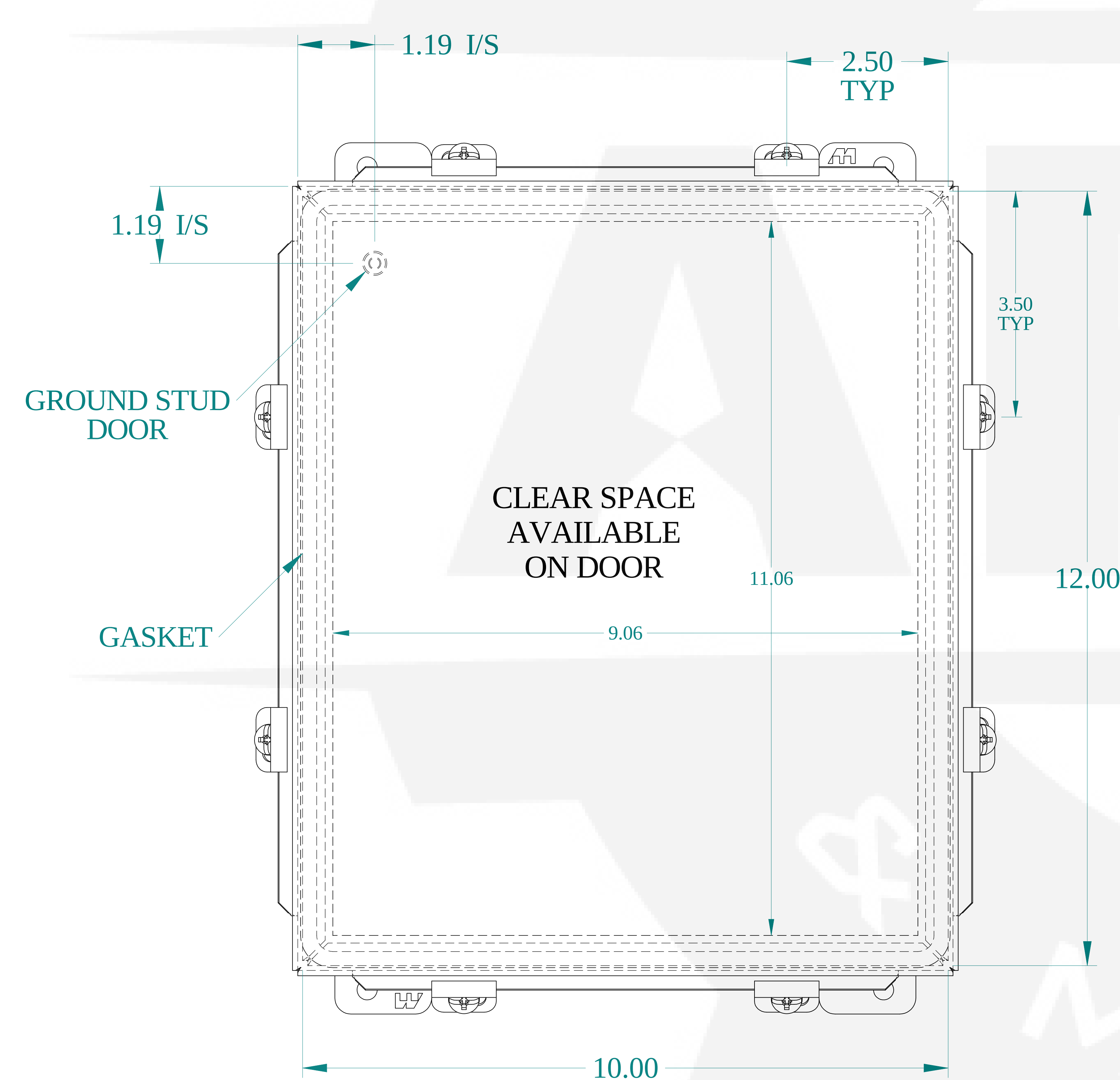
FRONT VIEW
