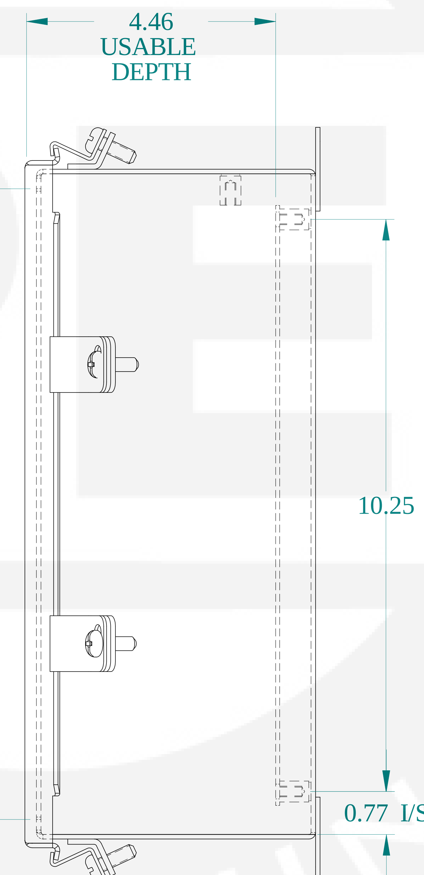
SIDE VIEW
