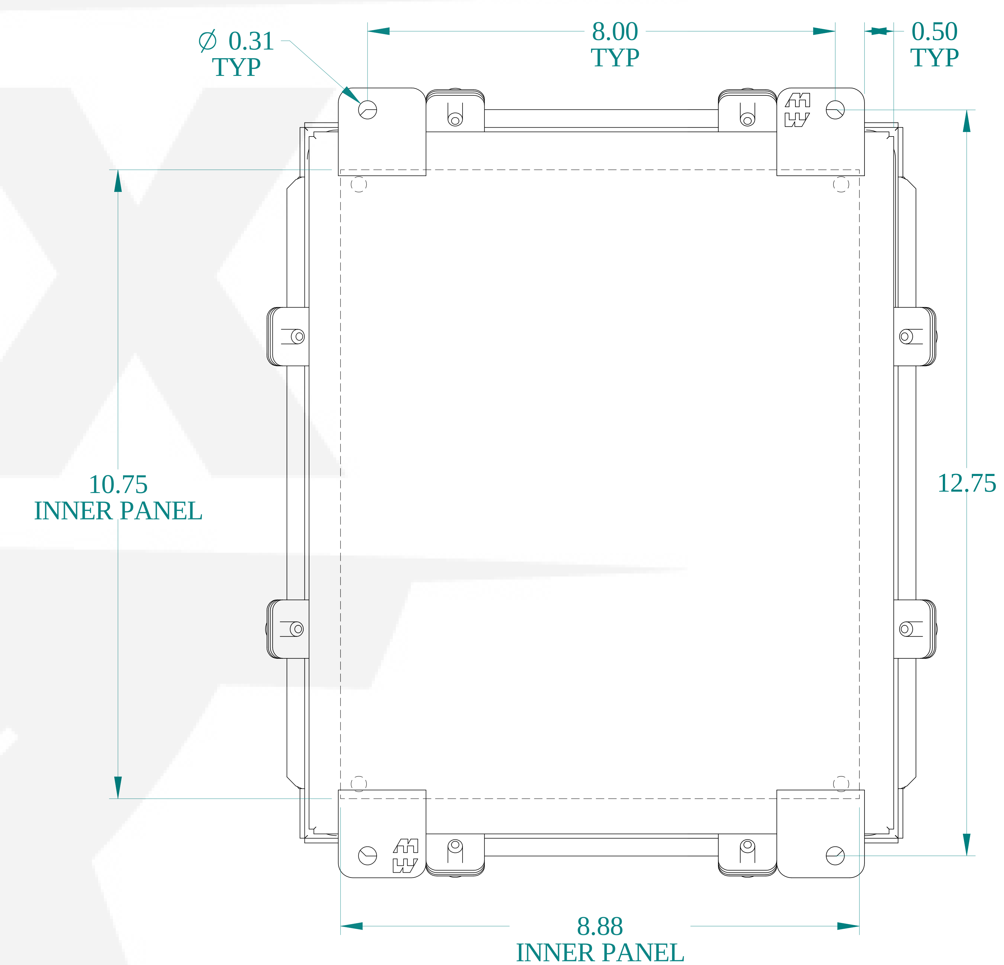
BACK VIEW
