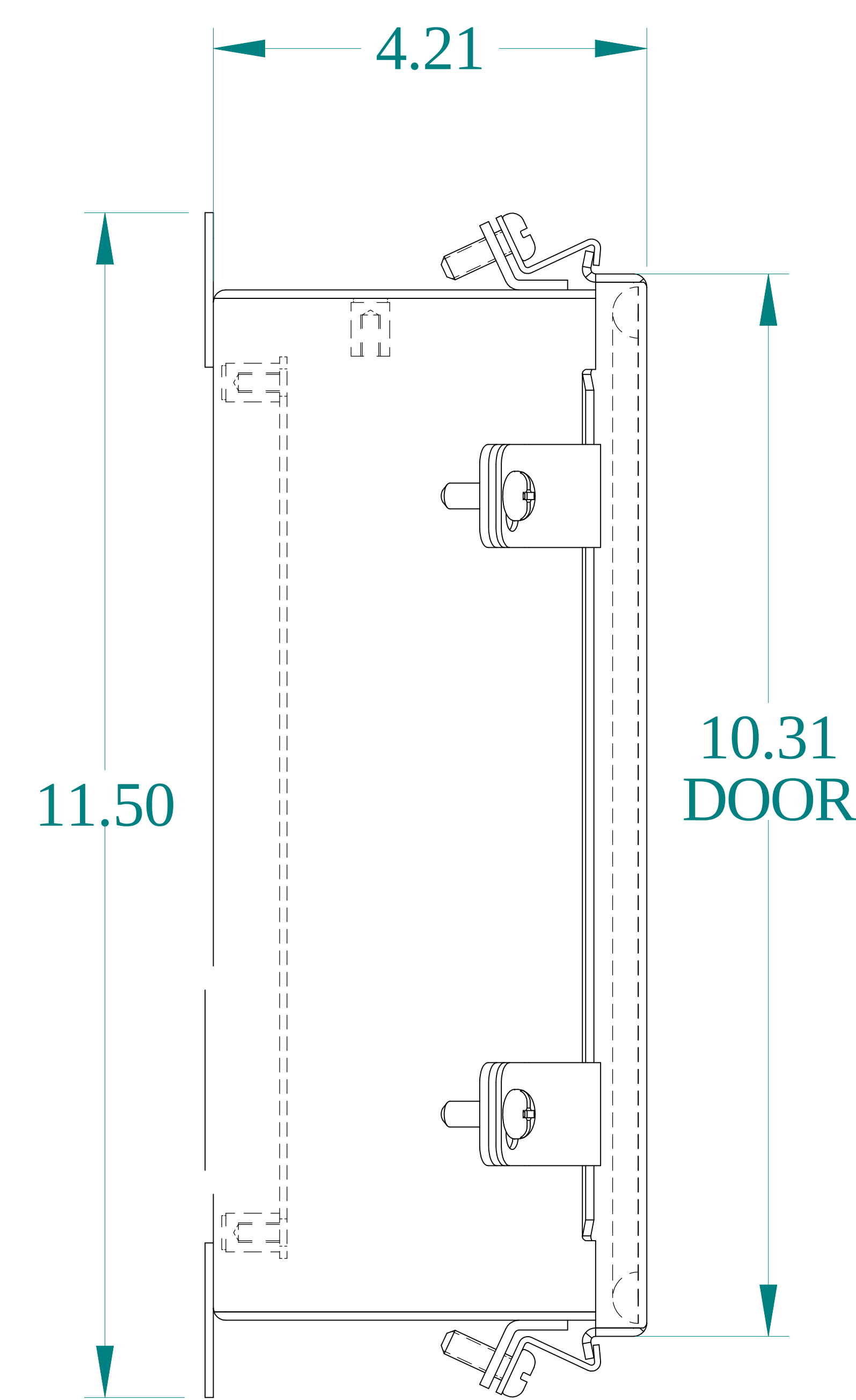
SIDE VIEW
