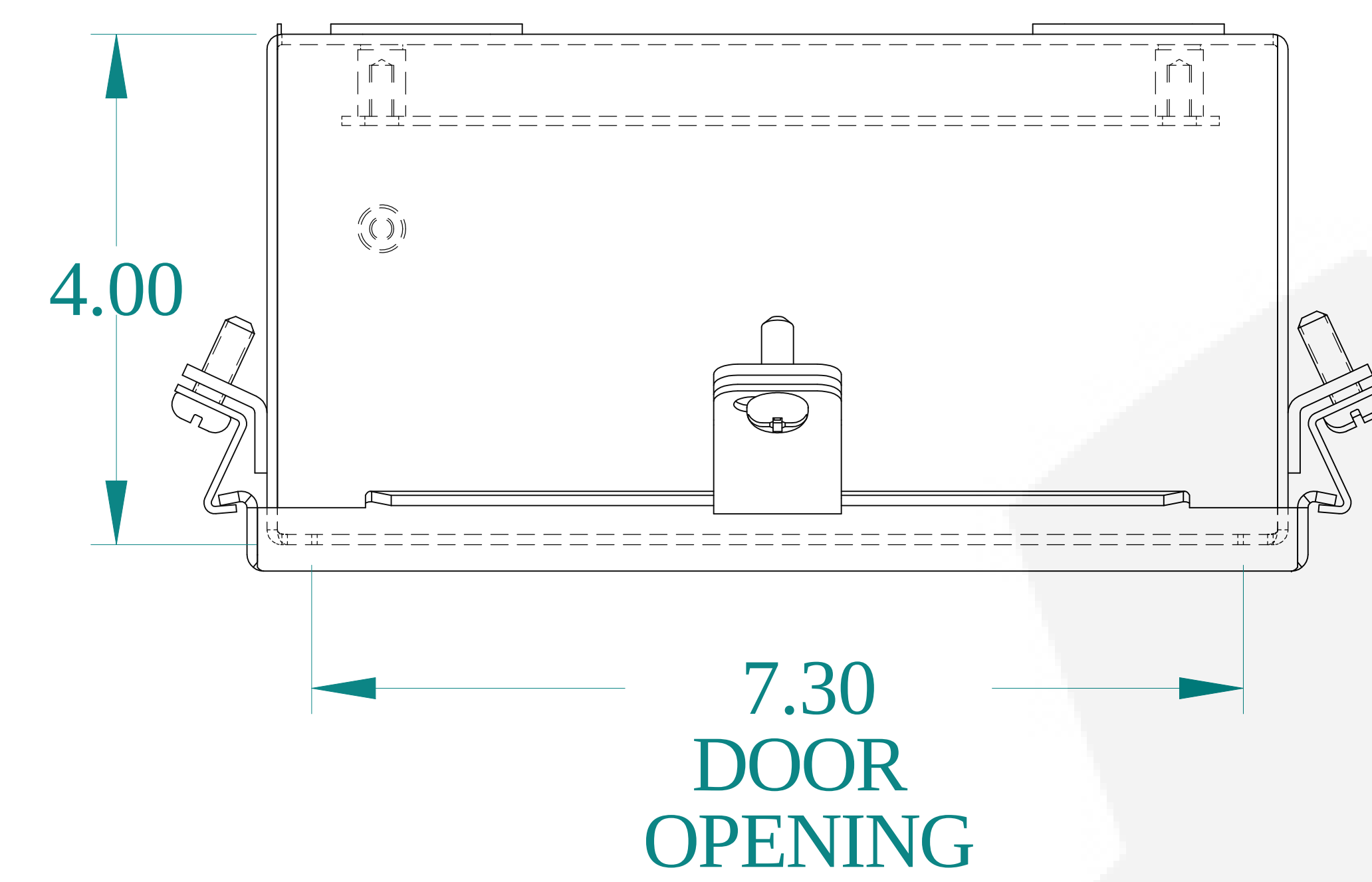
TOP VIEW
