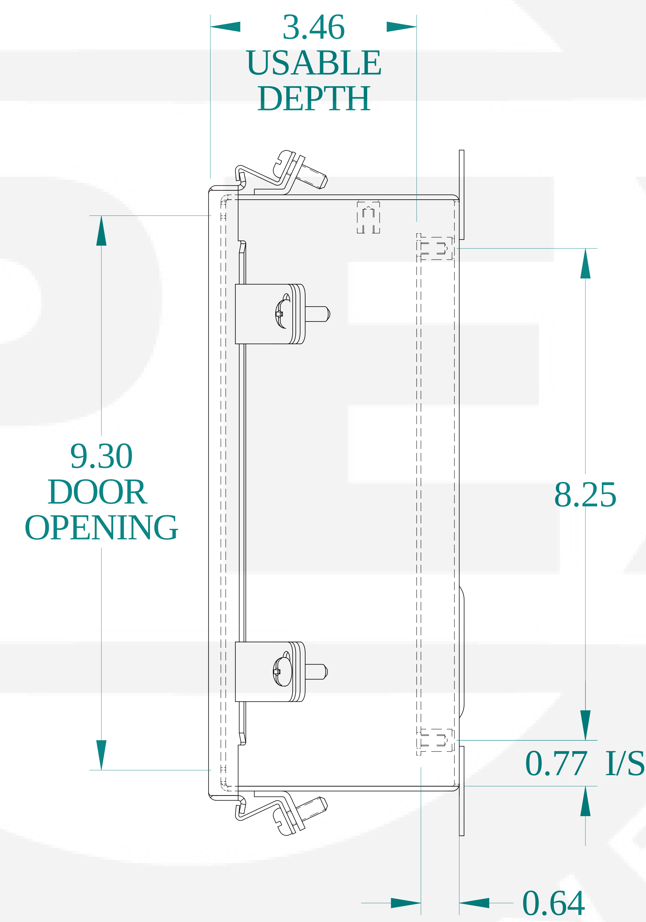
SIDE VIEW
