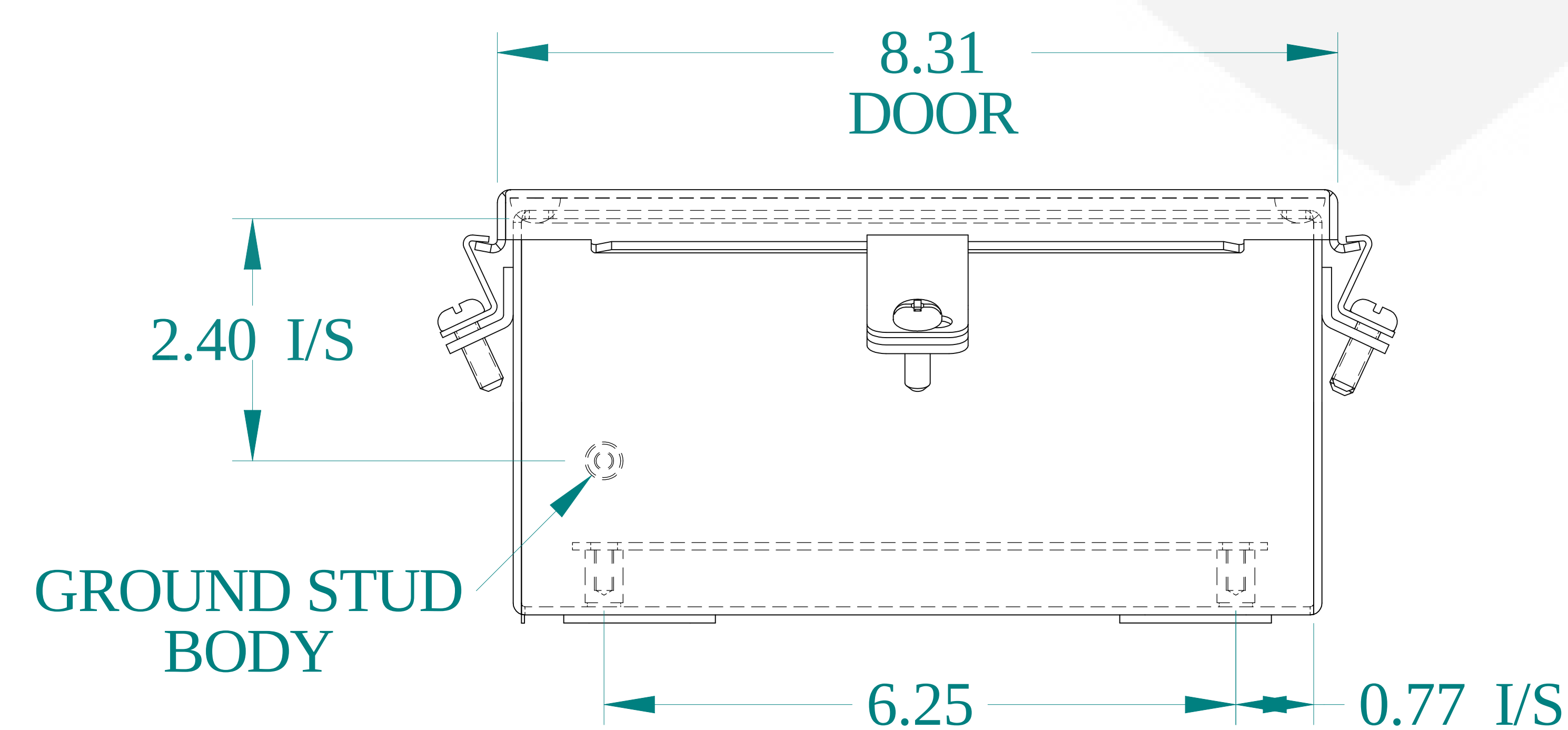
BOTTOM VIEW
