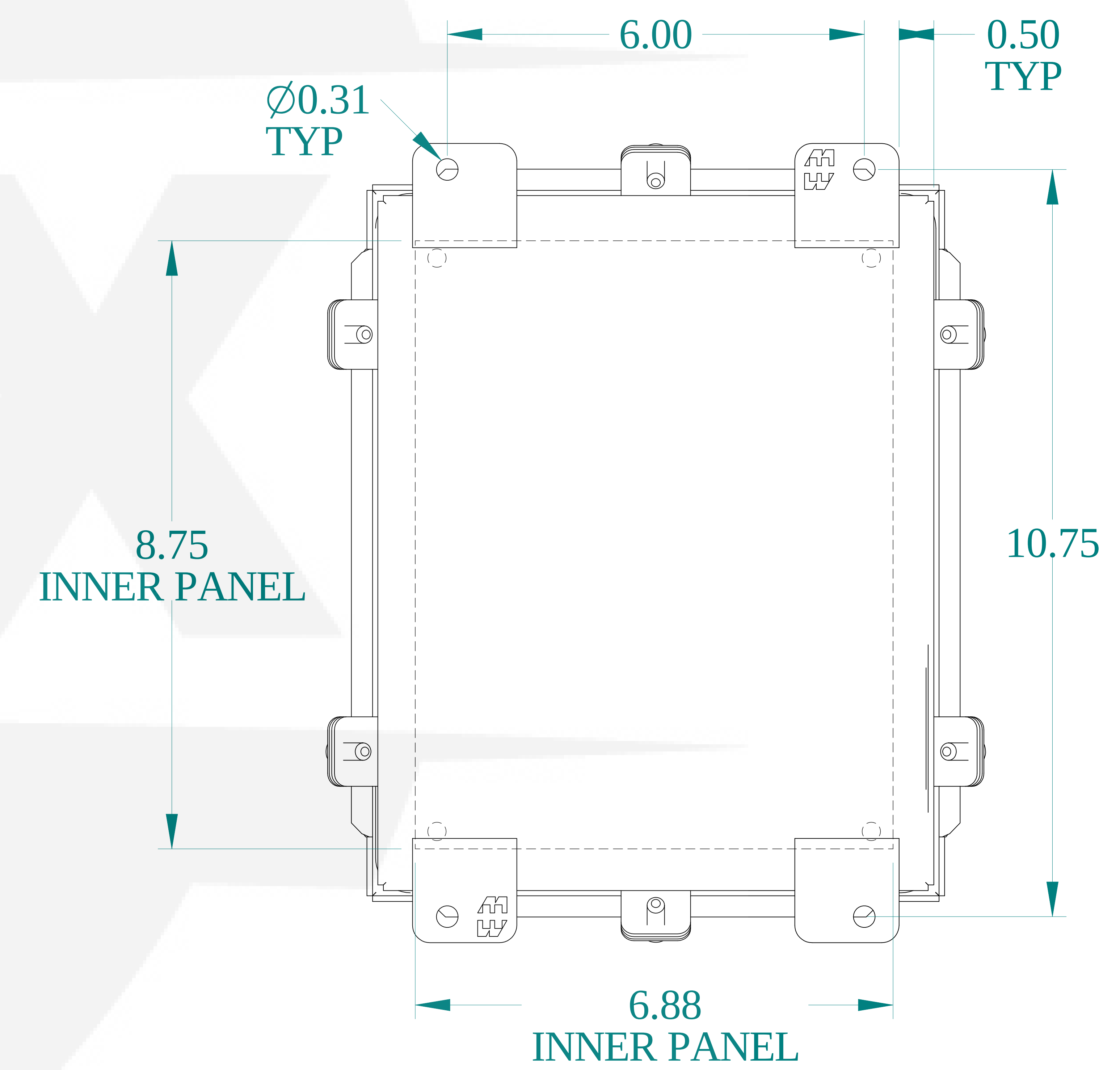
BACK VIEW
