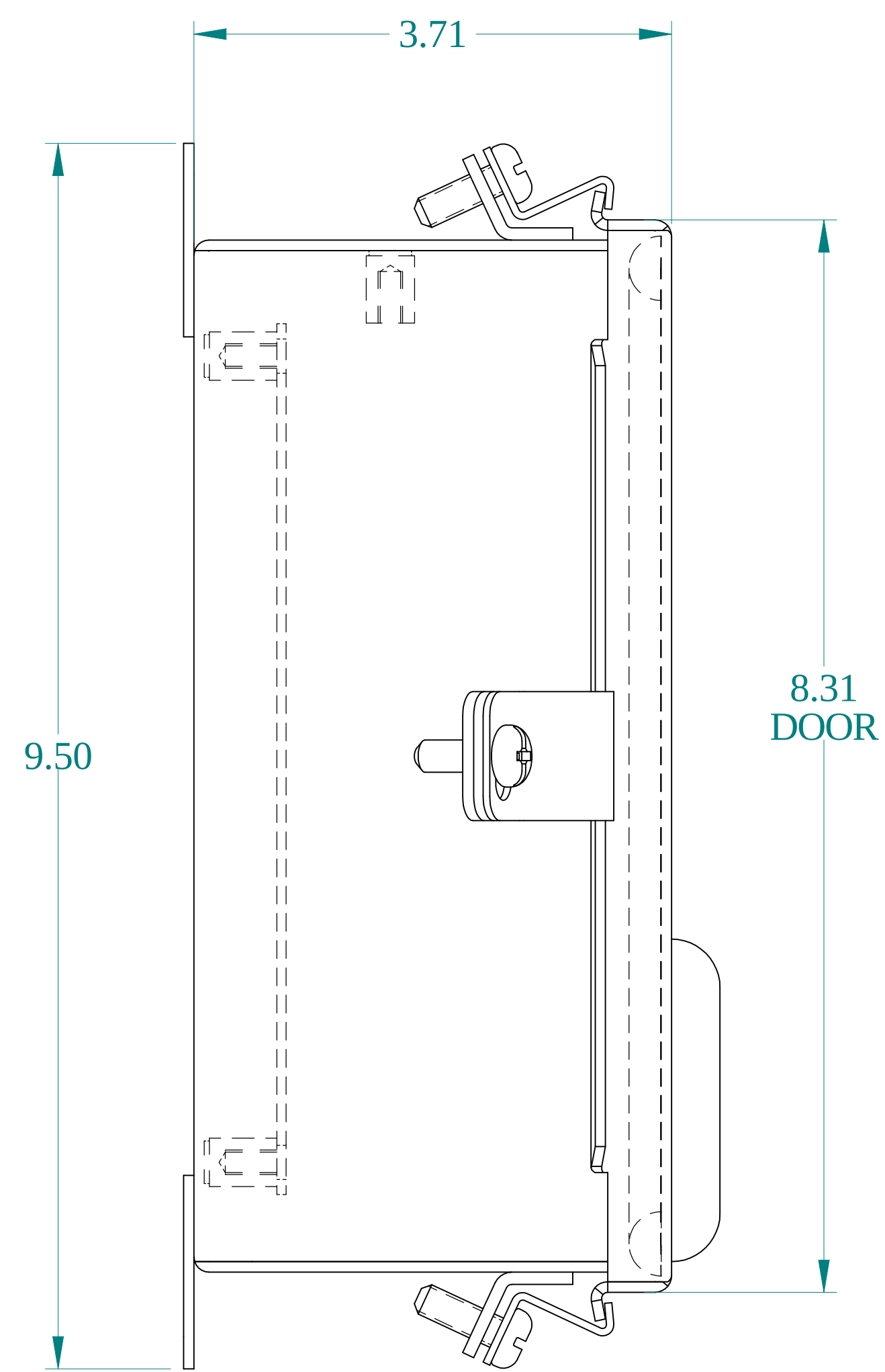
SIDE VIEW
