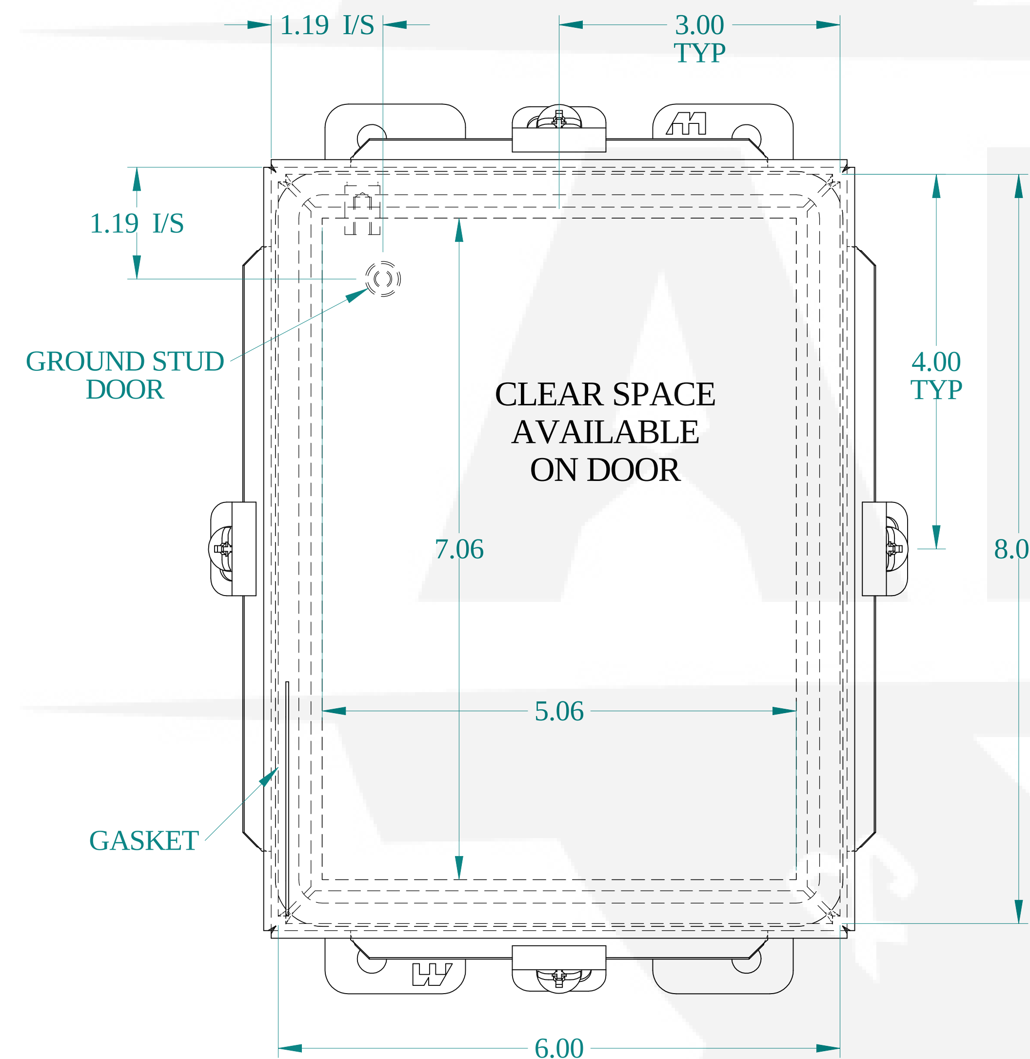
FRONT VIEW
