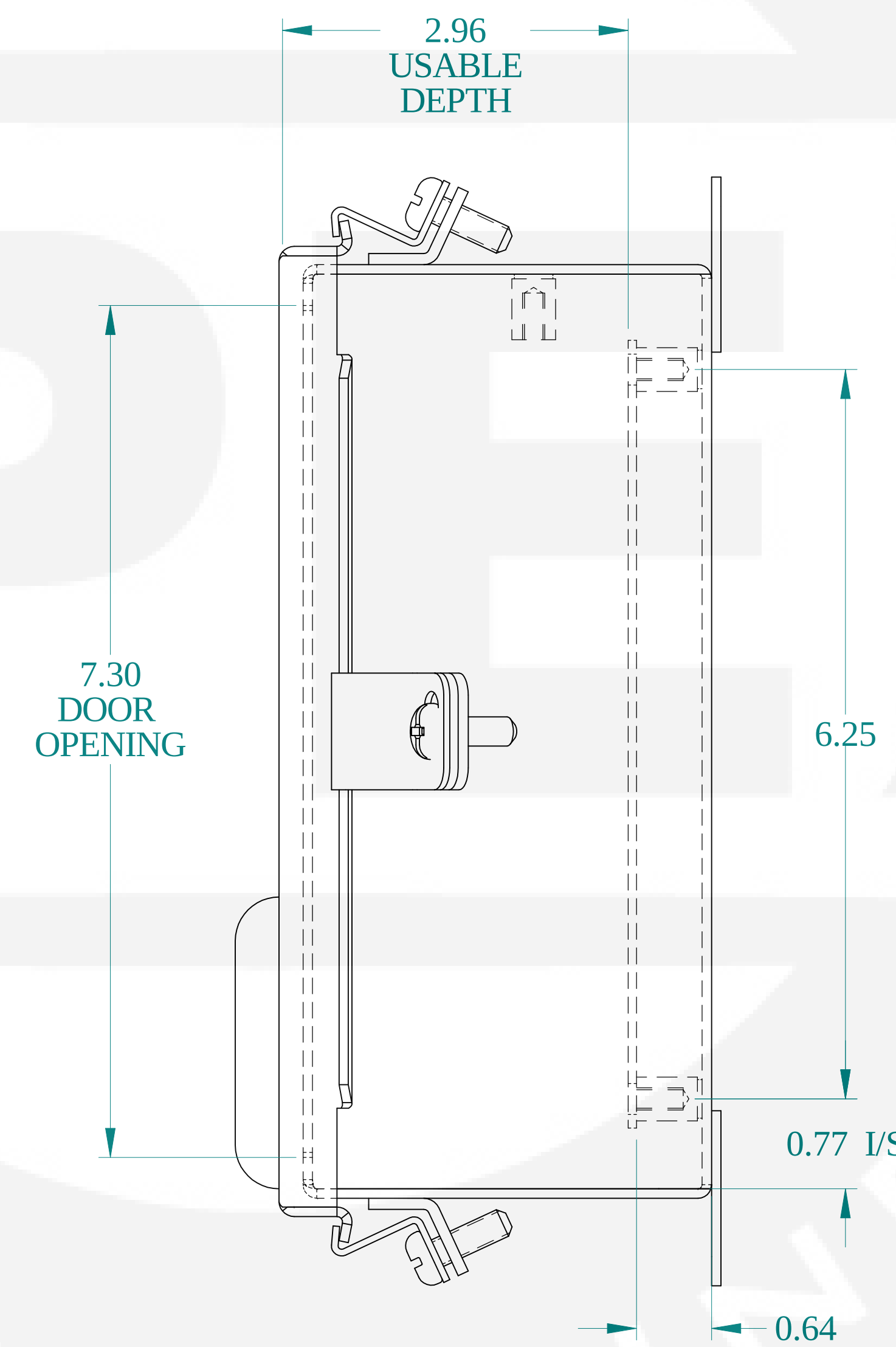
SIDE VIEW
