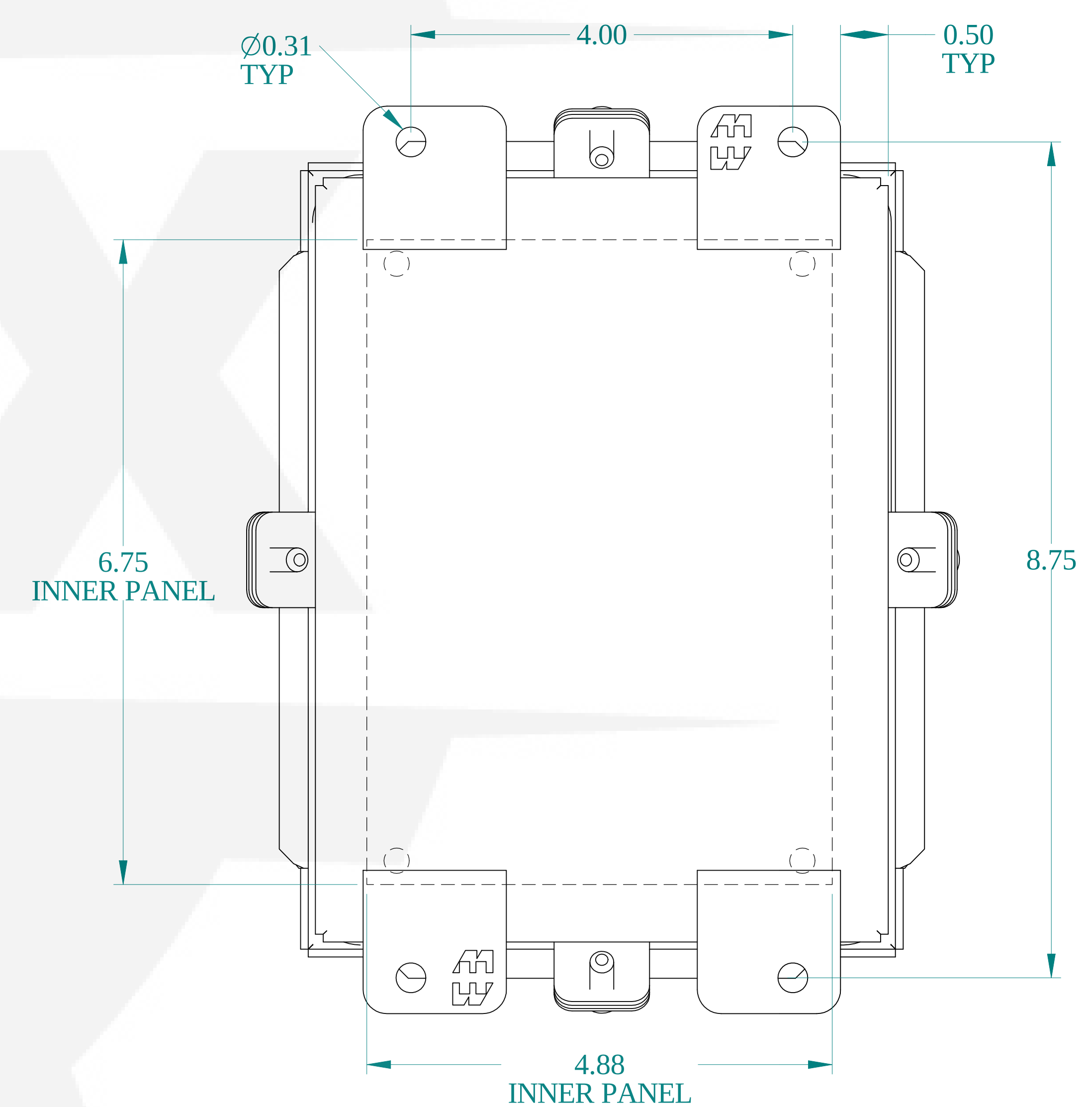
BACK VIEW
