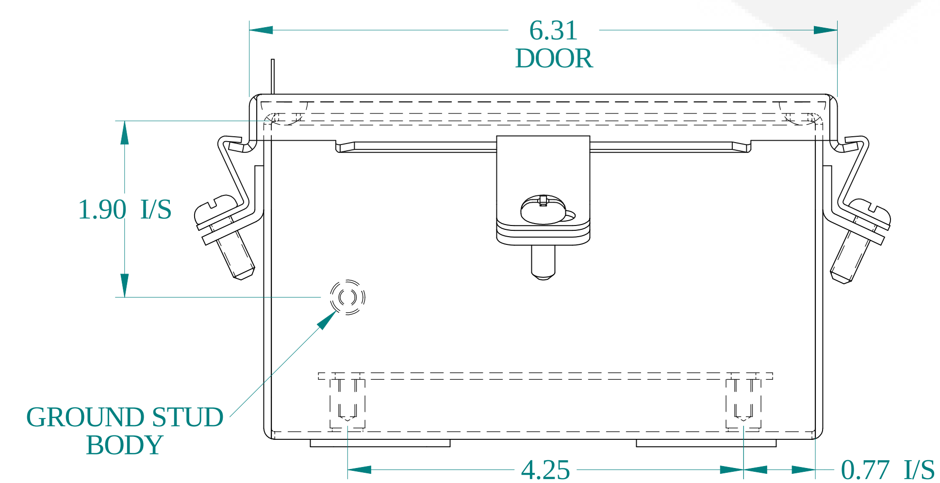
BOTTOM VIEW
