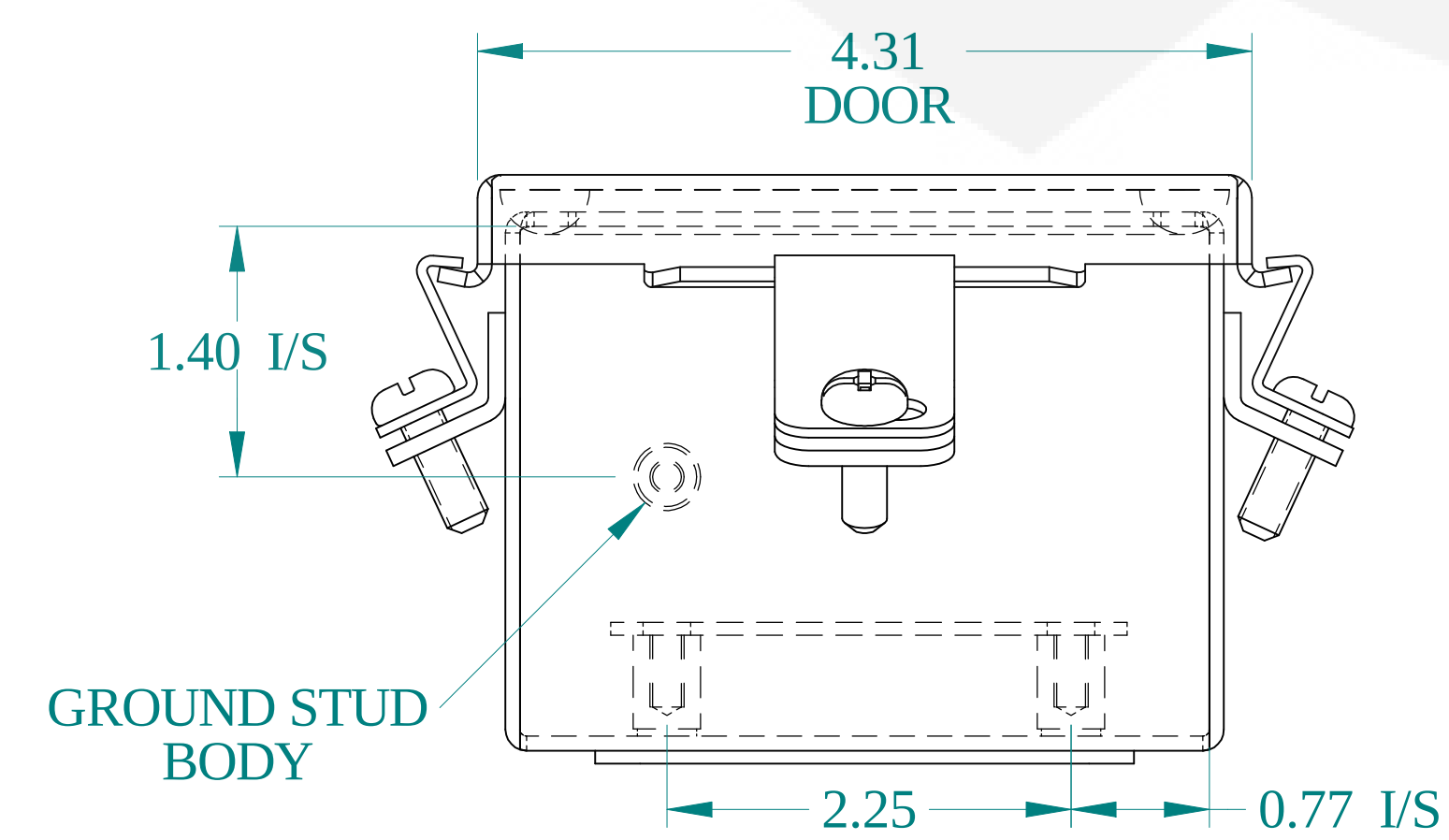
BOTTOM VIEW
