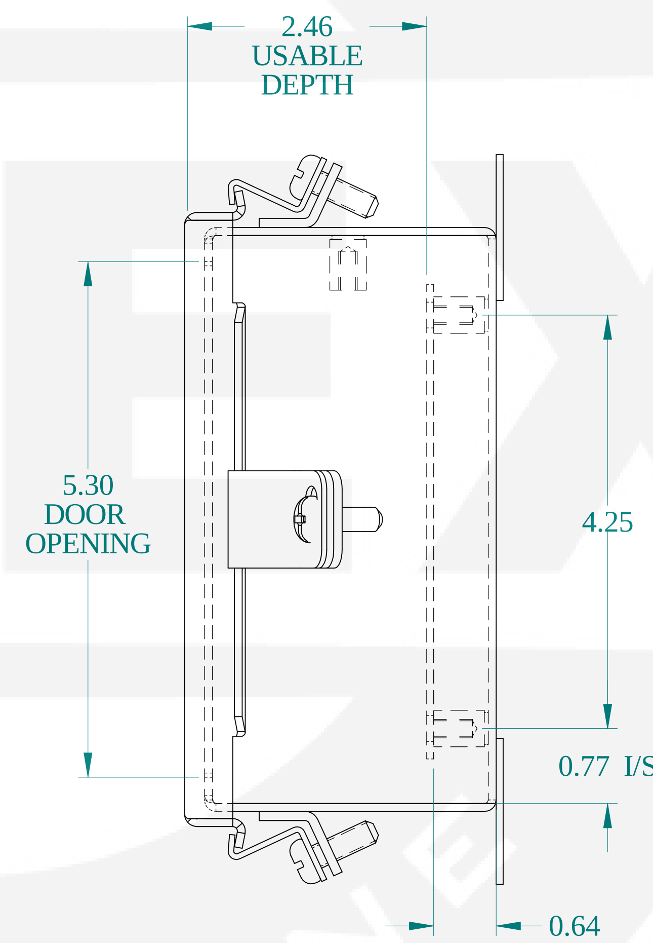
SIDE VIEW
