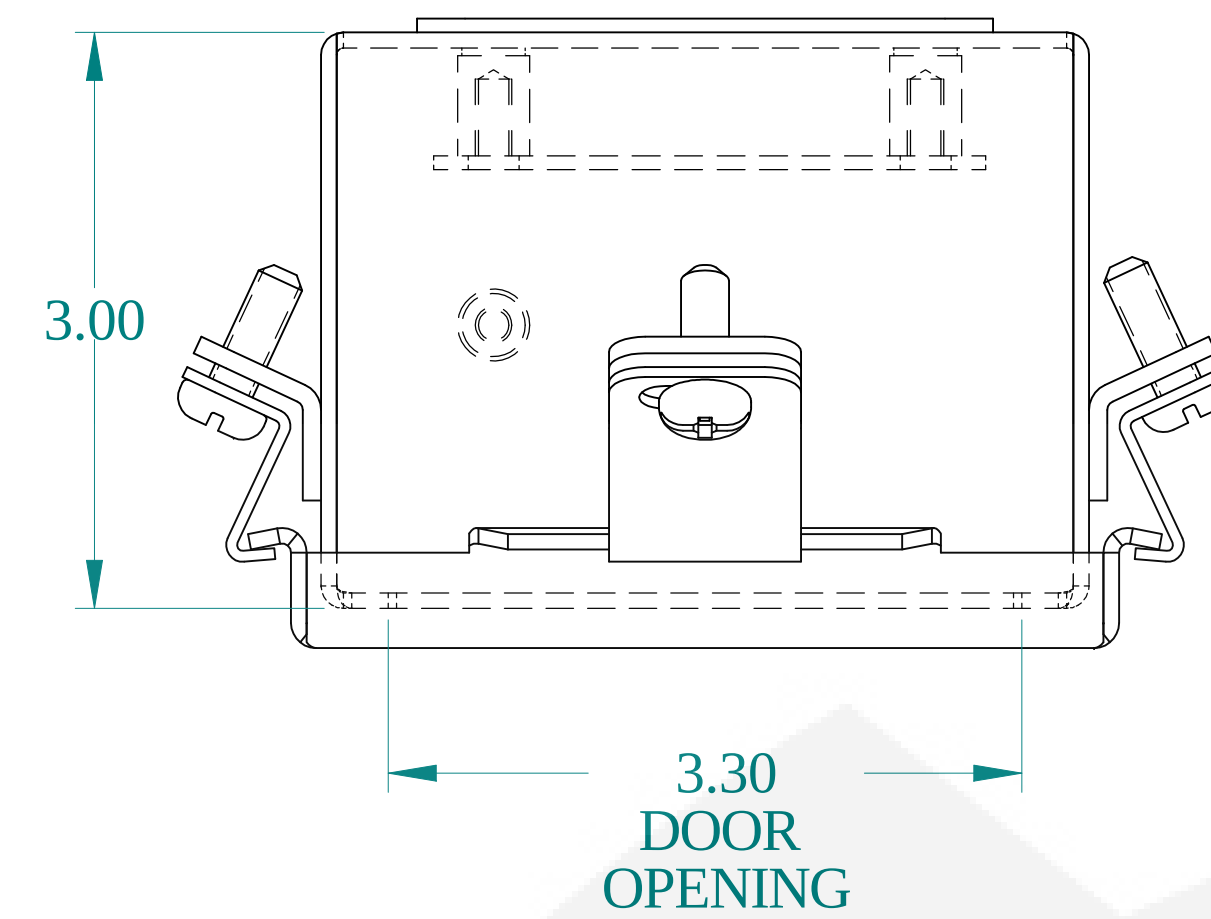
TOP VIEW
