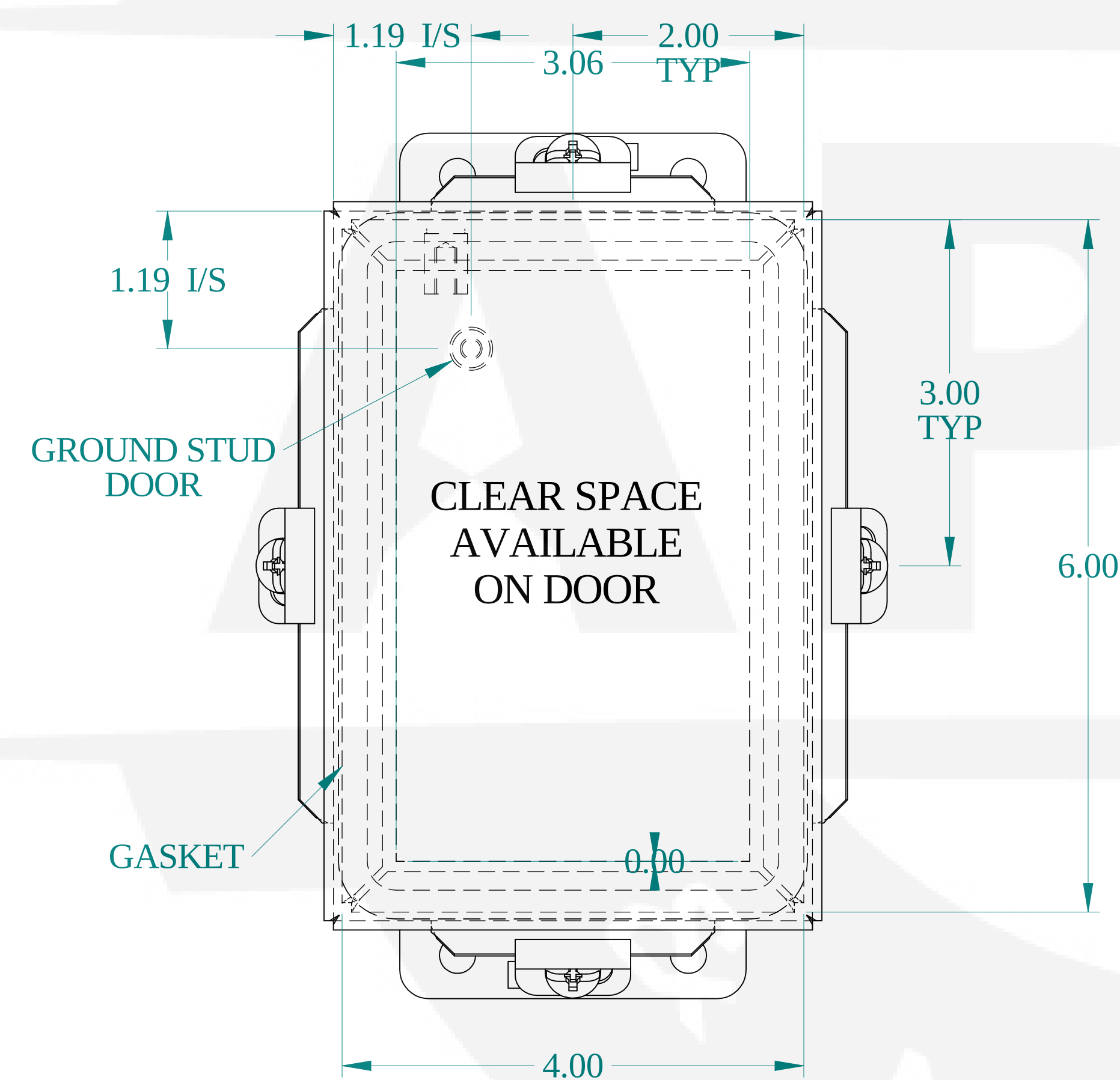
FRONT VIEW
