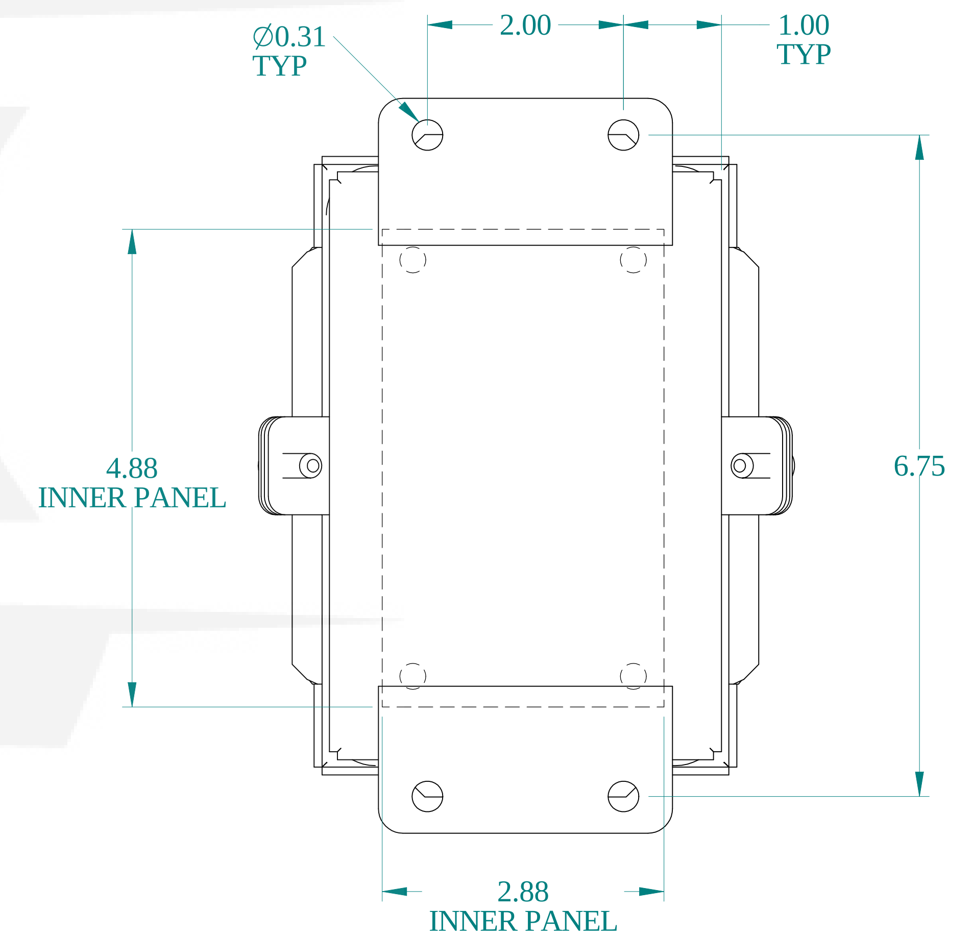
BACK VIEW
