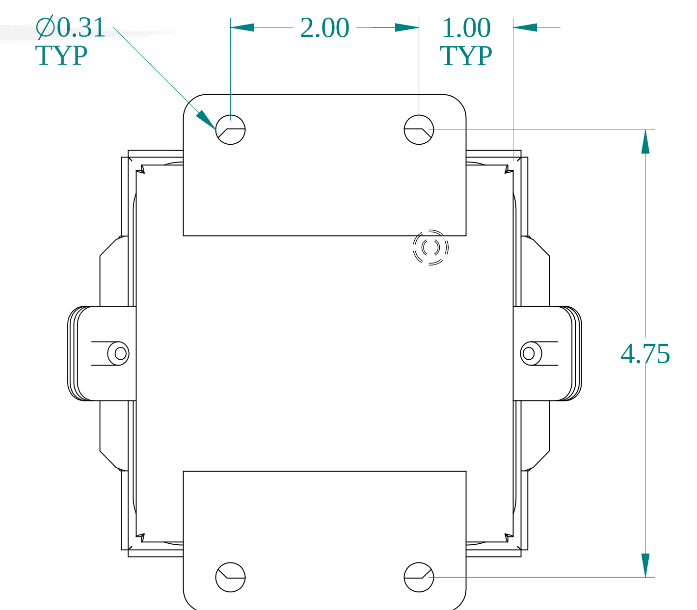
BACK VIEW
