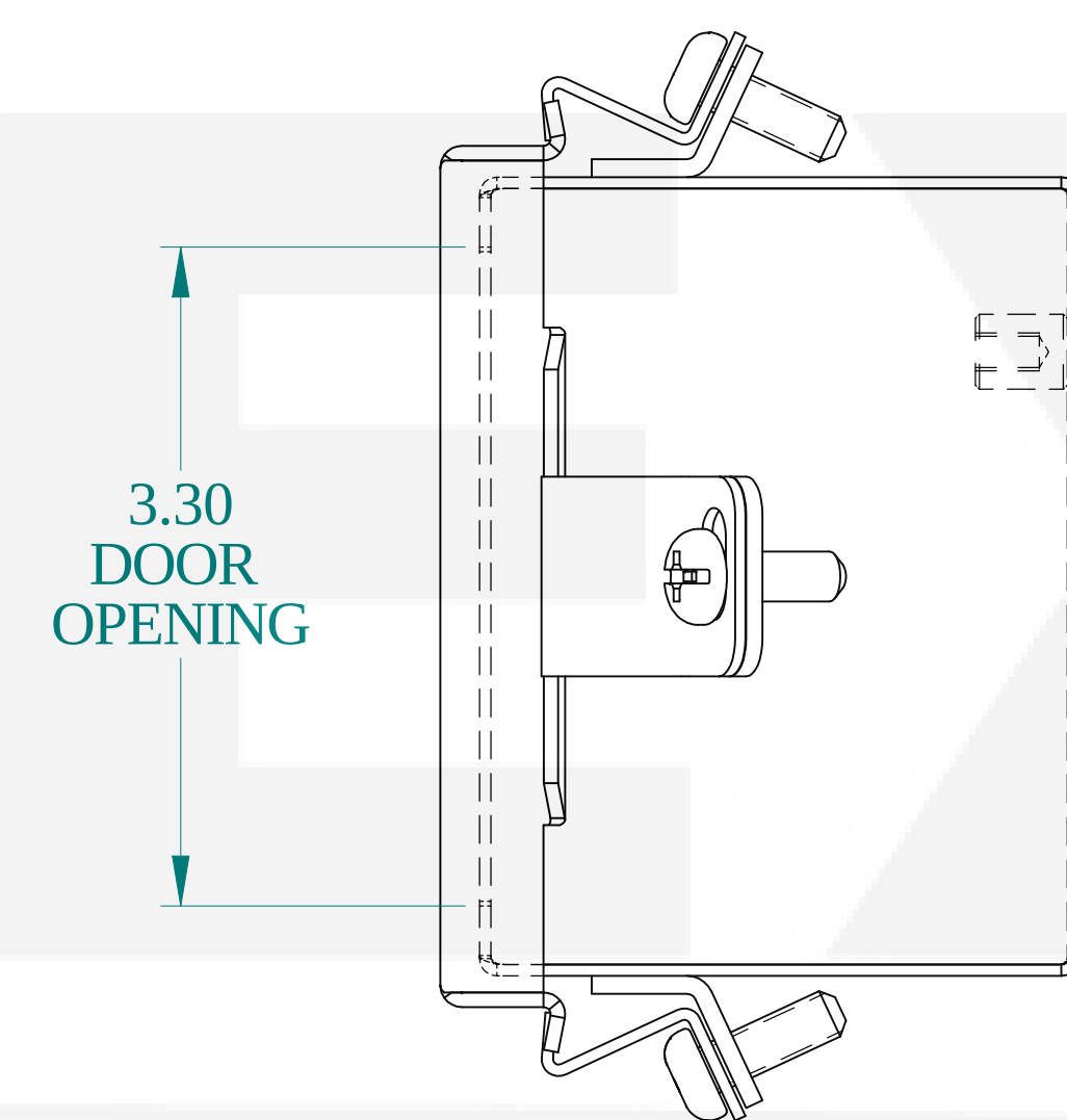
SIDE VIEW
