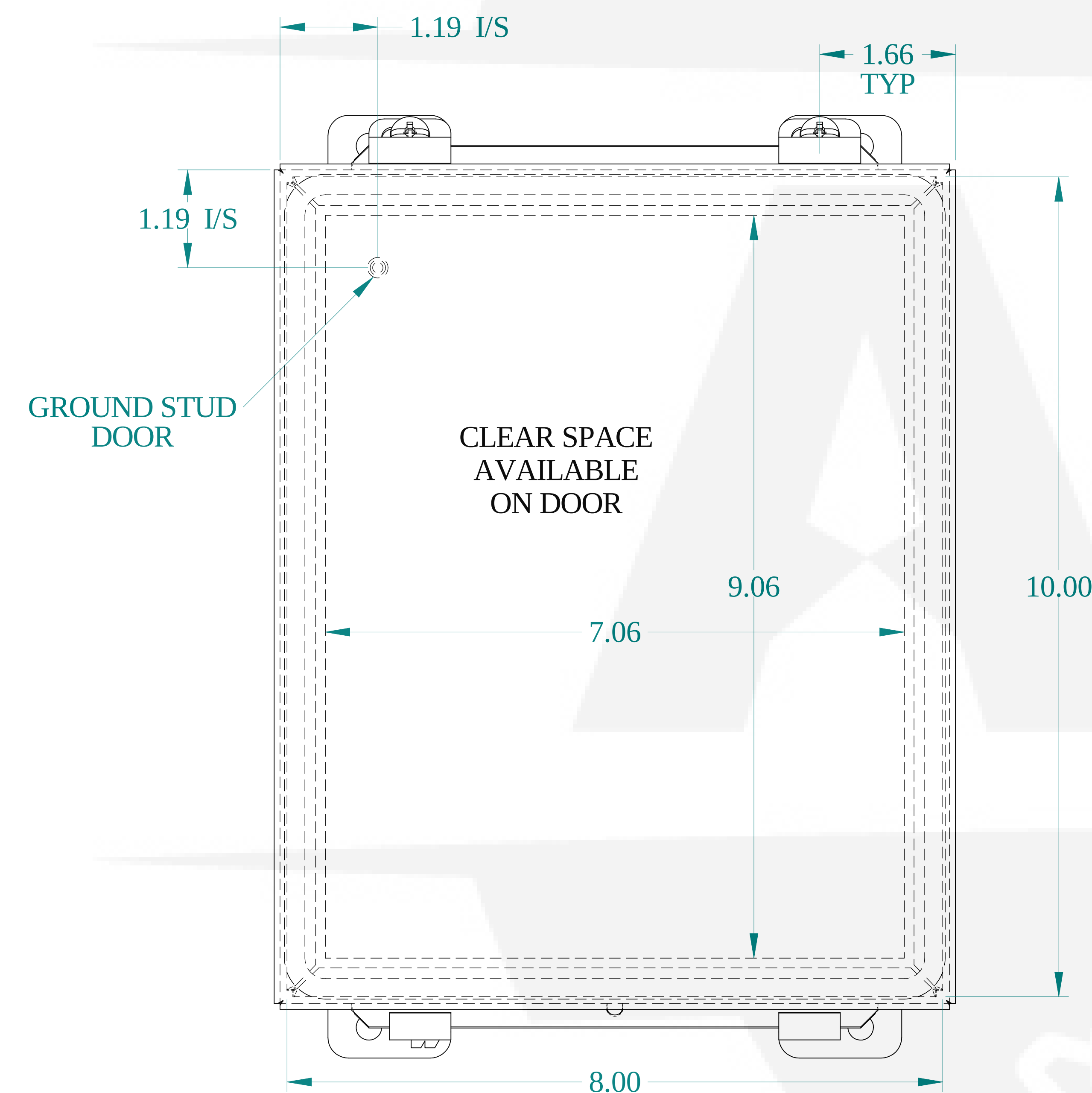
FRONT VIEW
