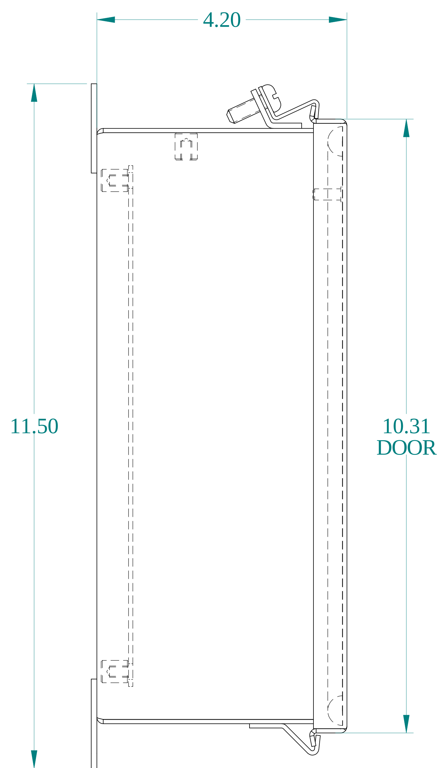
SIDE VIEW
