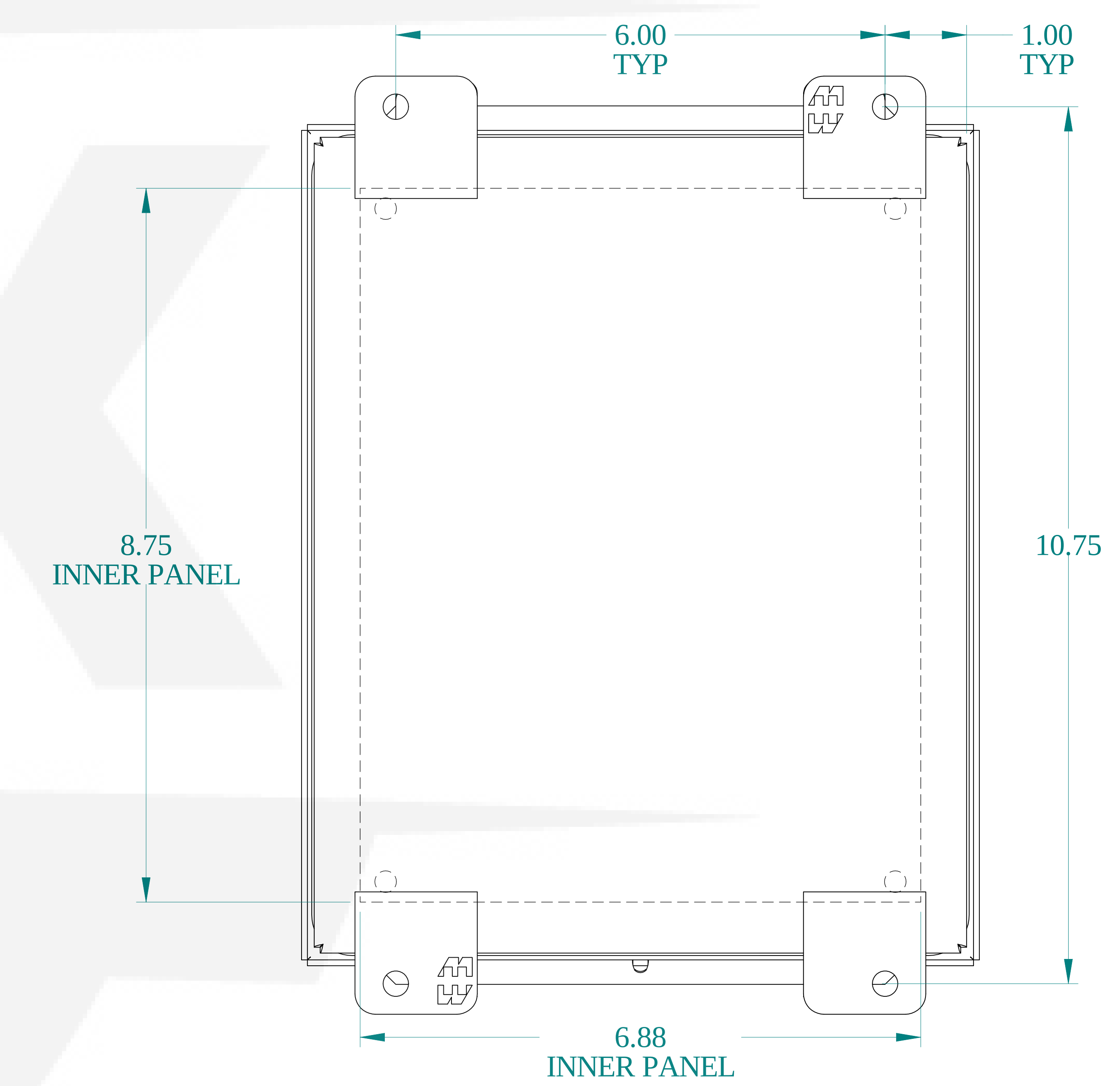
BACK VIEW
