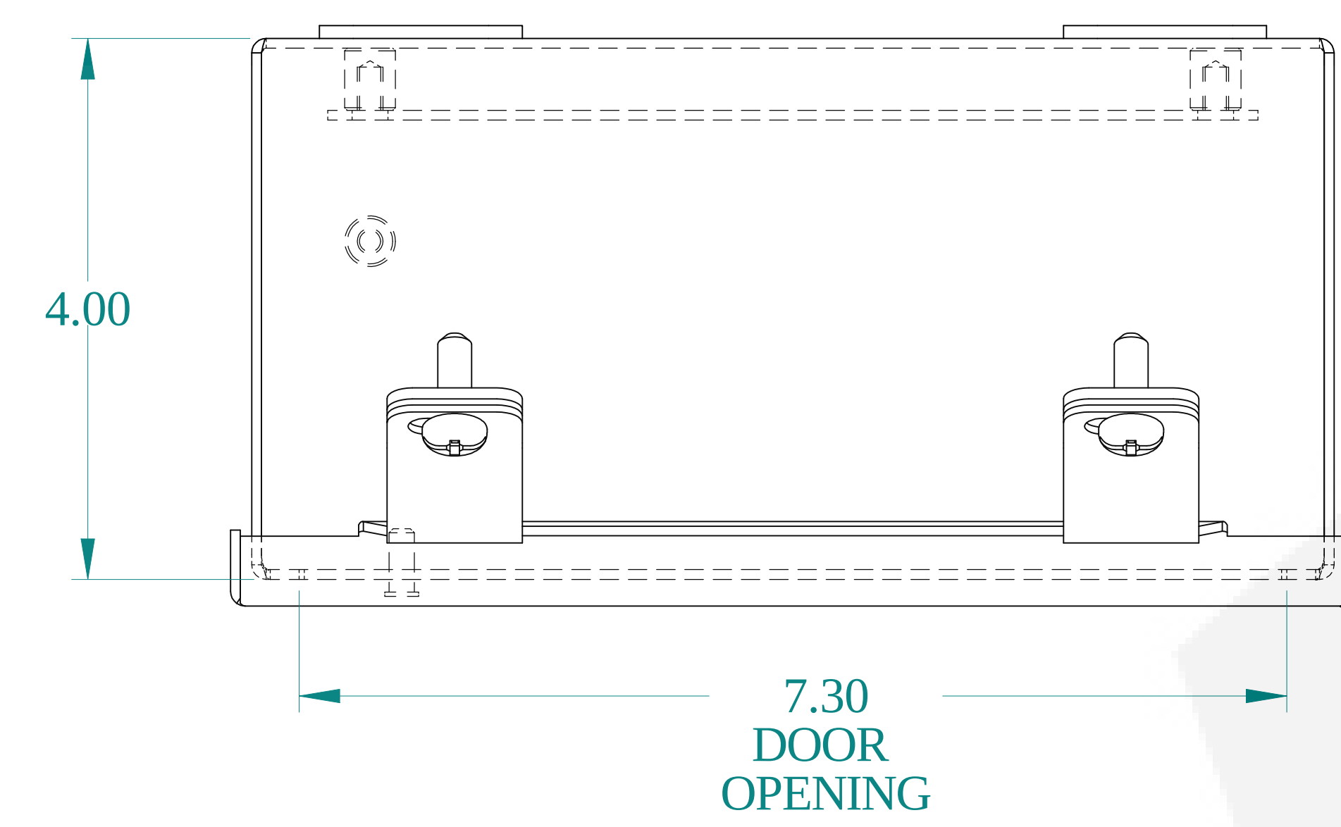
TOP VIEW
