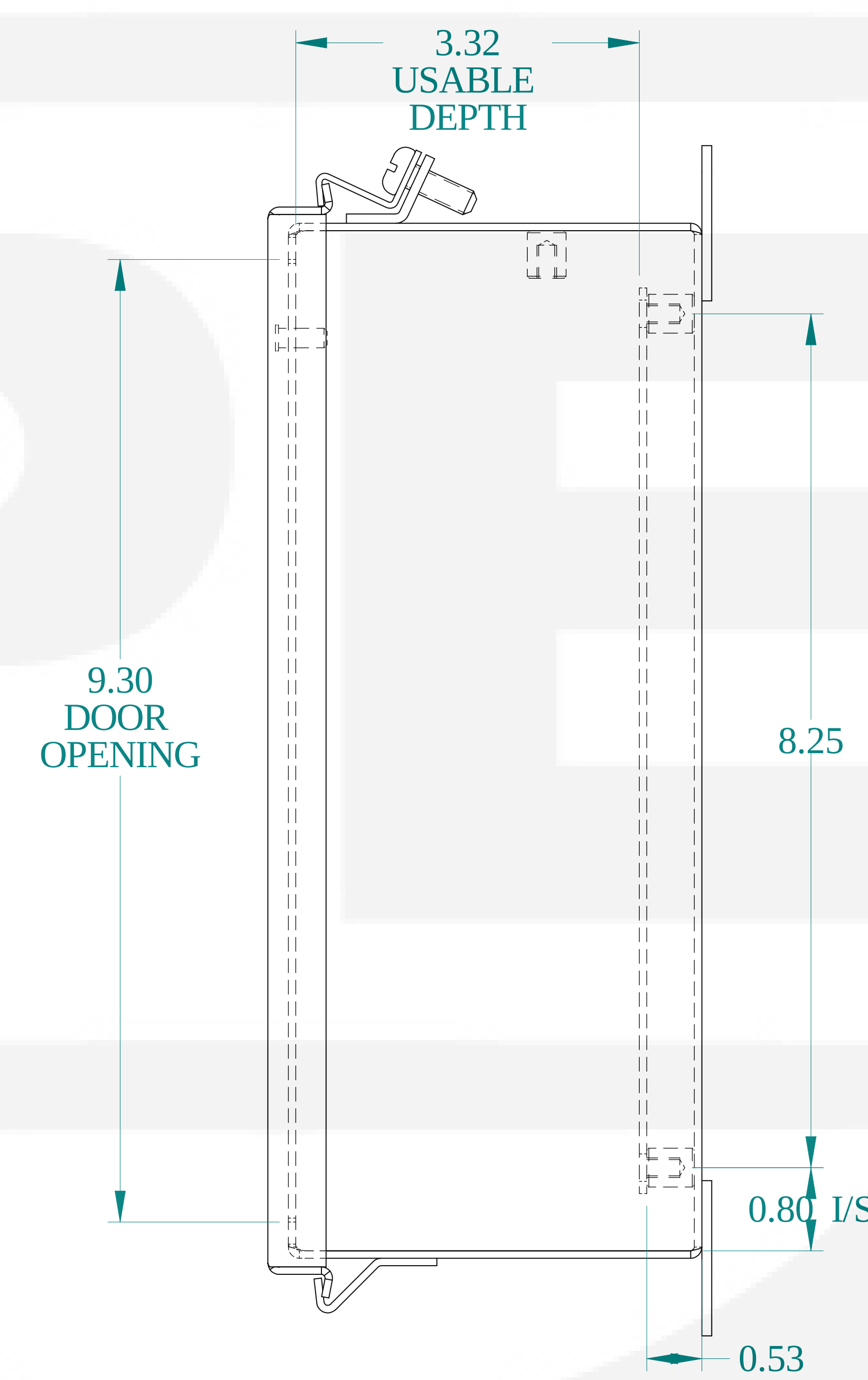
SIDE VIEW
