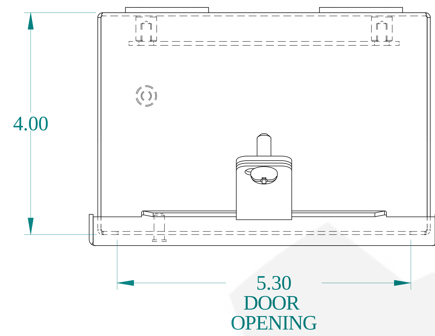
TOP VIEW
