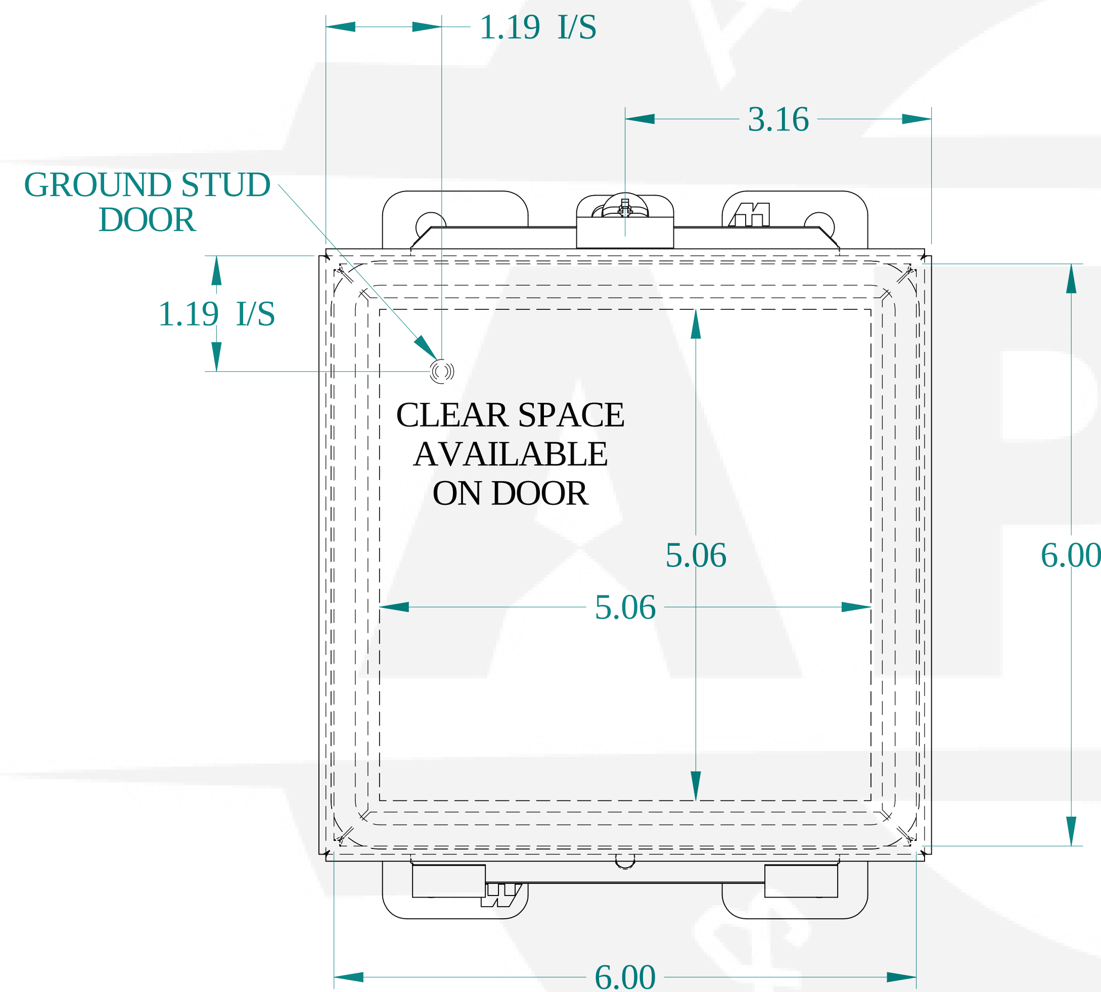
FRONT VIEW
