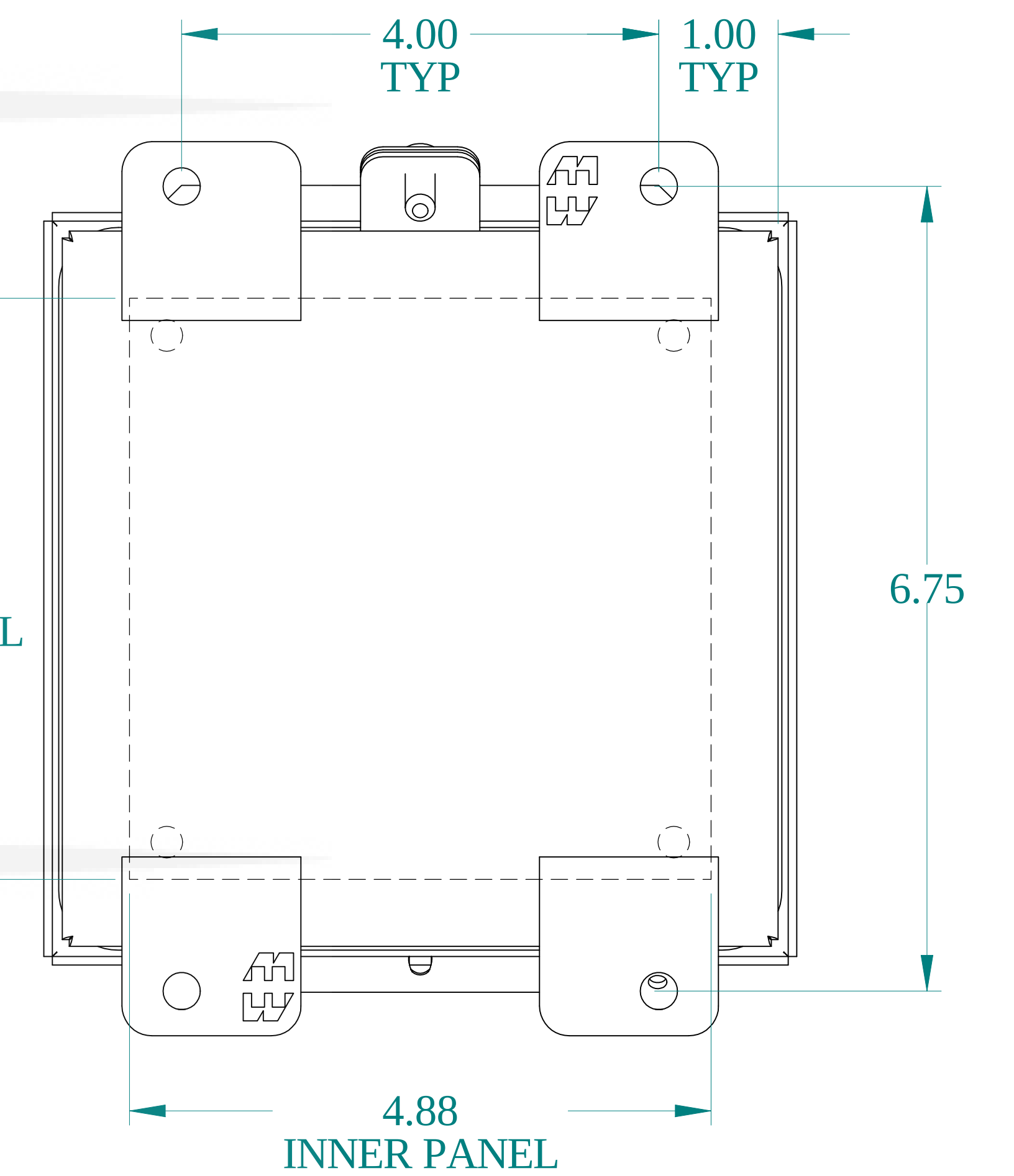
BACK VIEW
