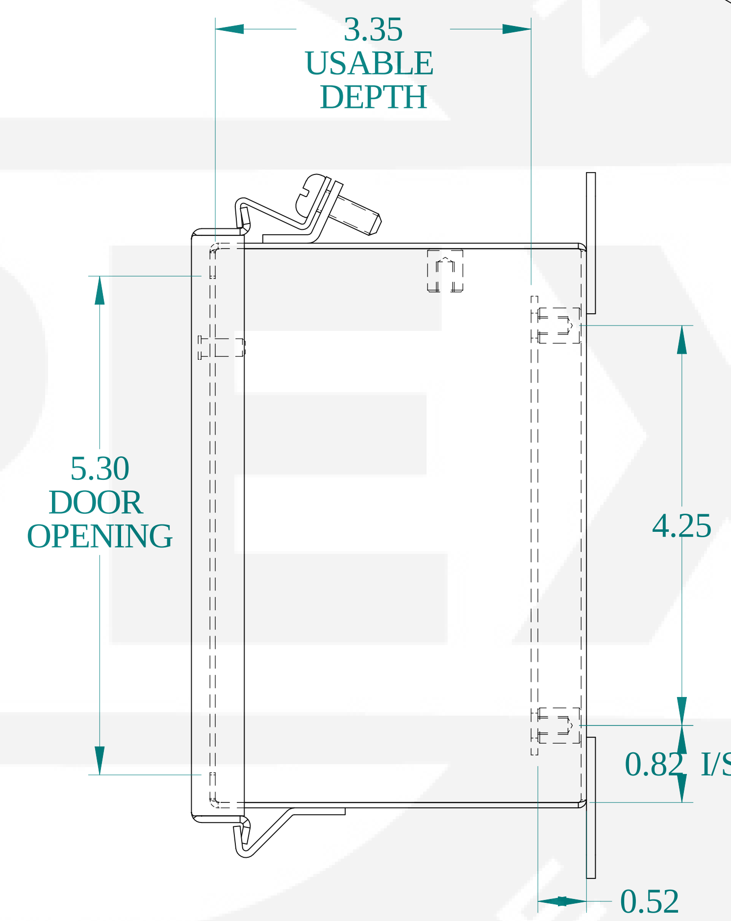
SIDE VIEW
