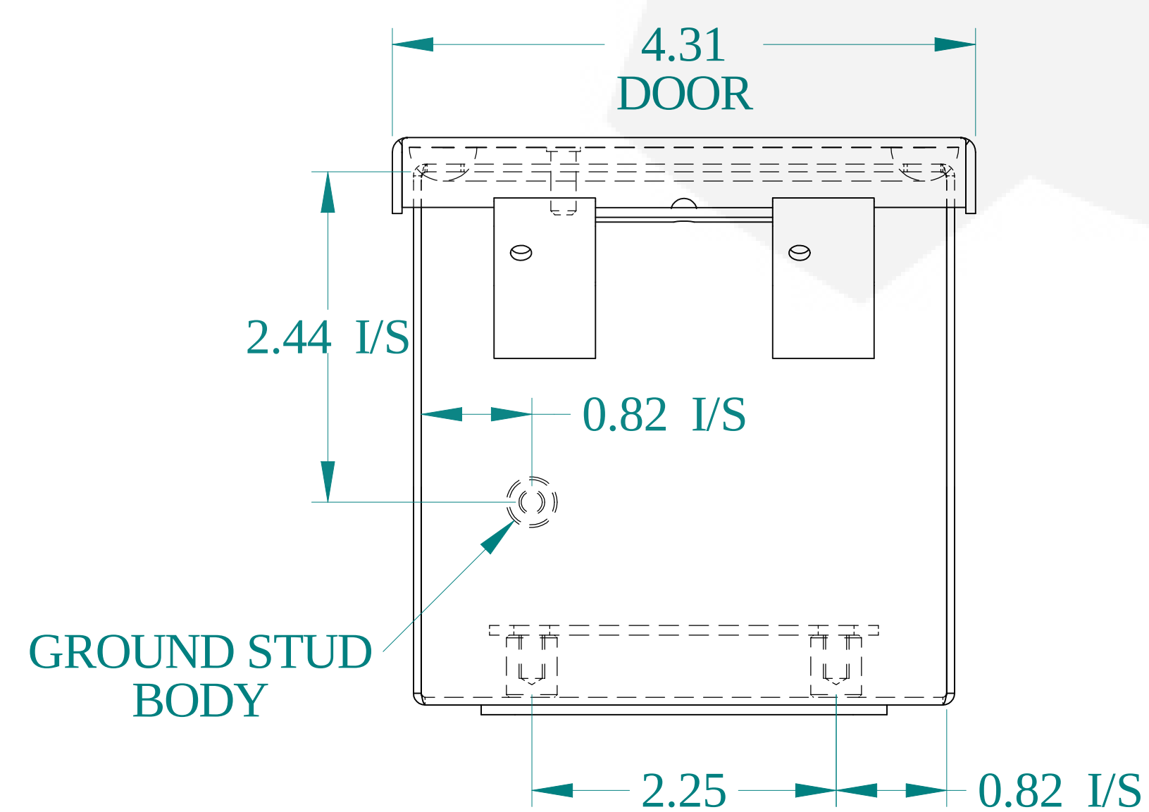
BOTTOM VIEW
