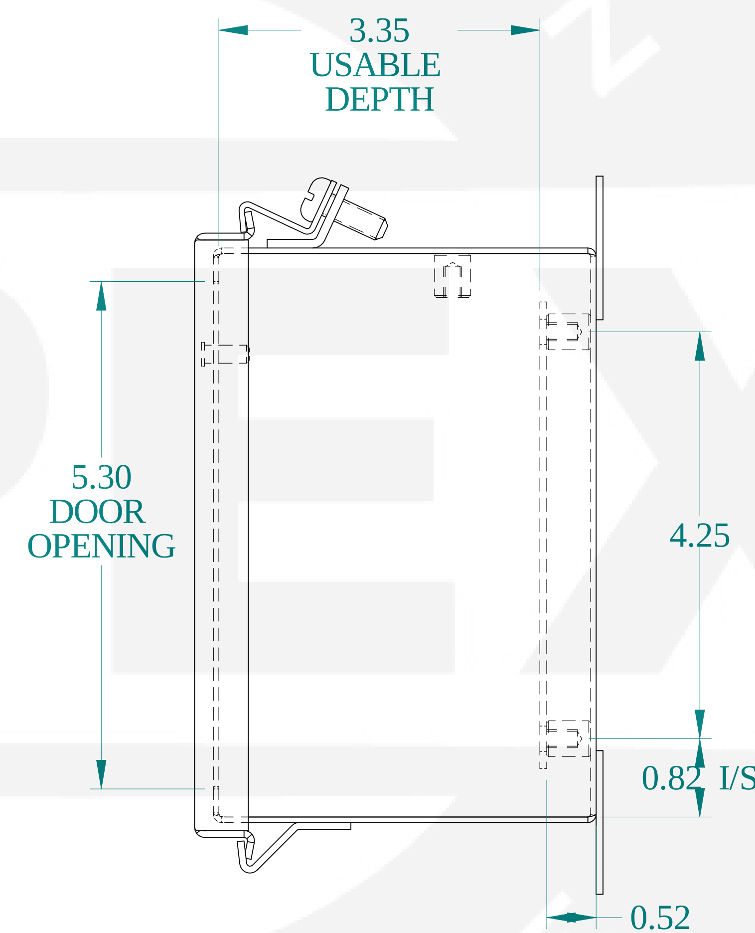
SIDE VIEW
