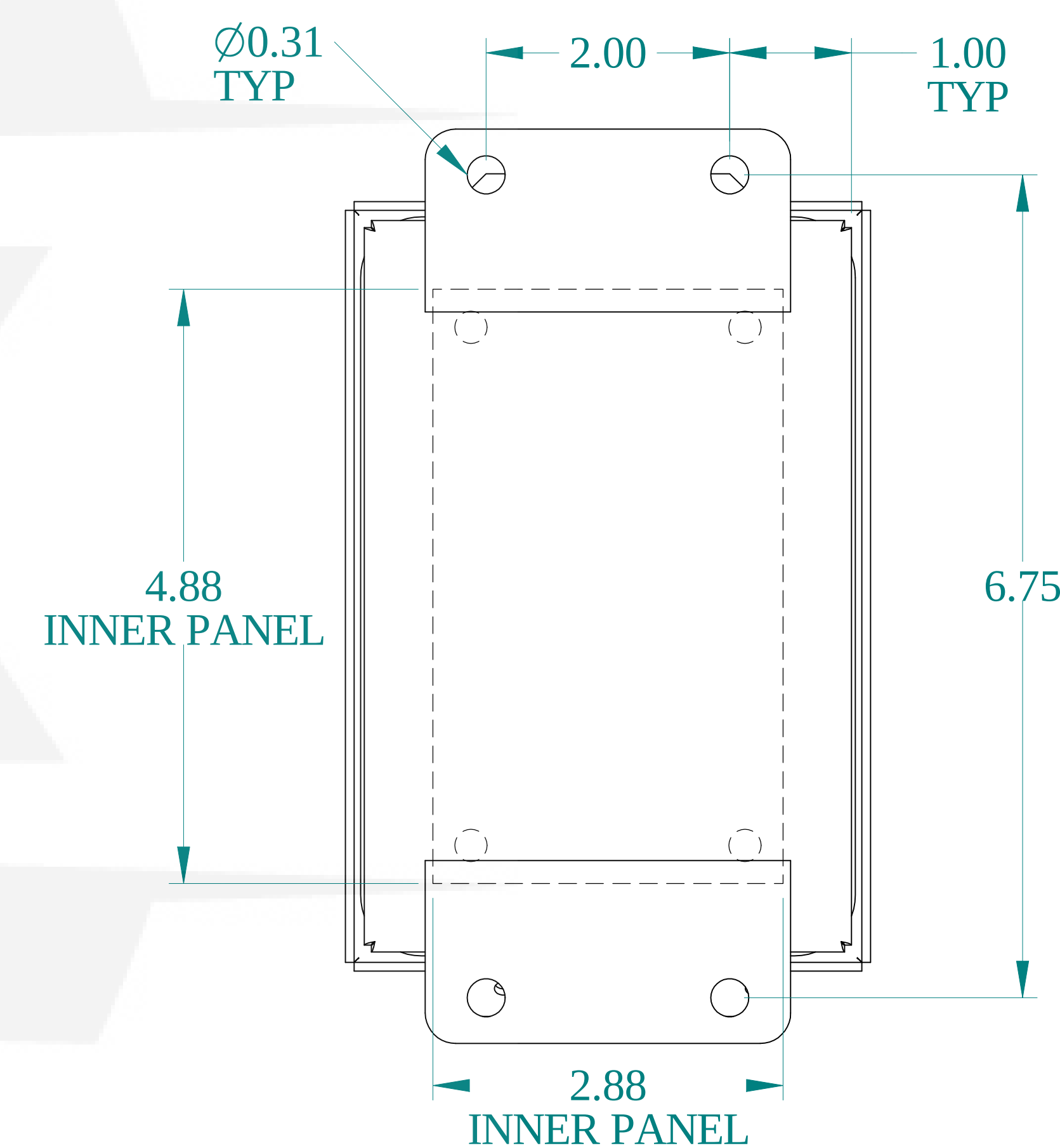
BACK VIEW
