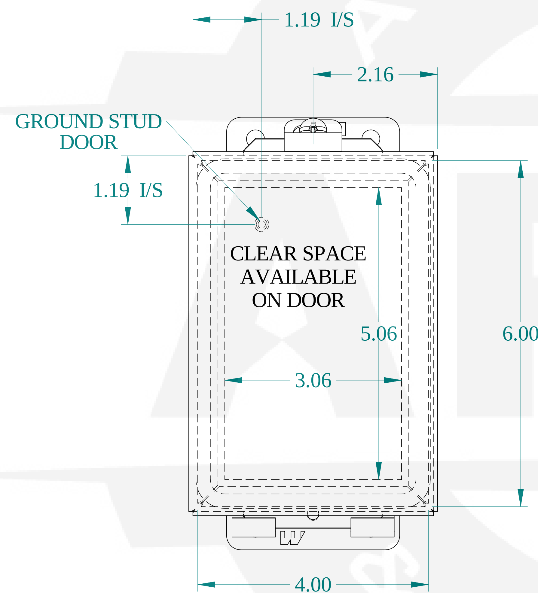
FRONT VIEW
