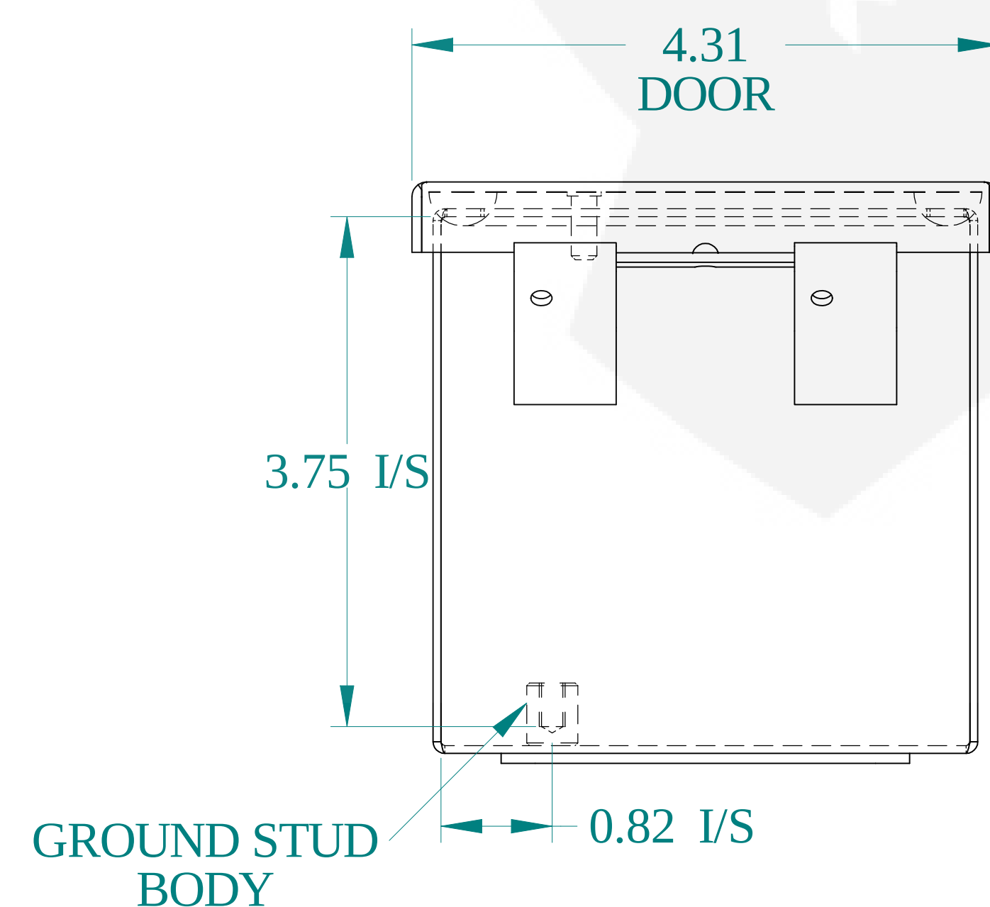
BOTTOM VIEW
