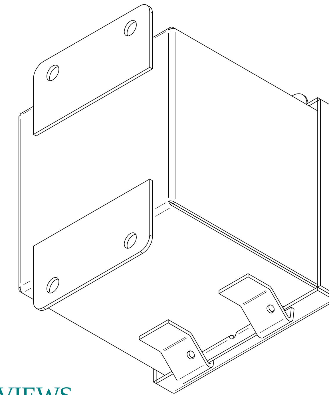
ISOMETRIC VIEWS
