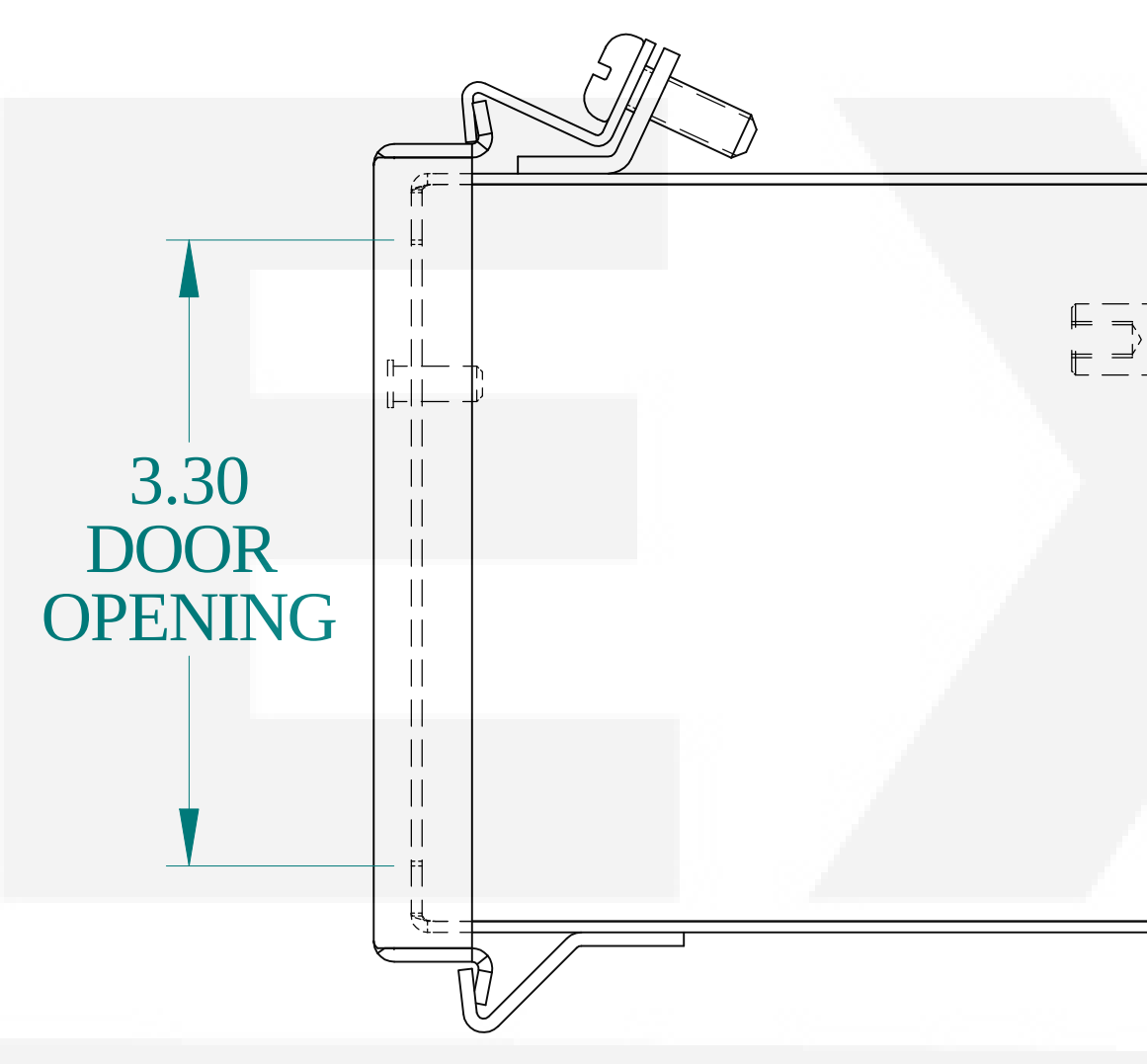
SIDE VIEW
