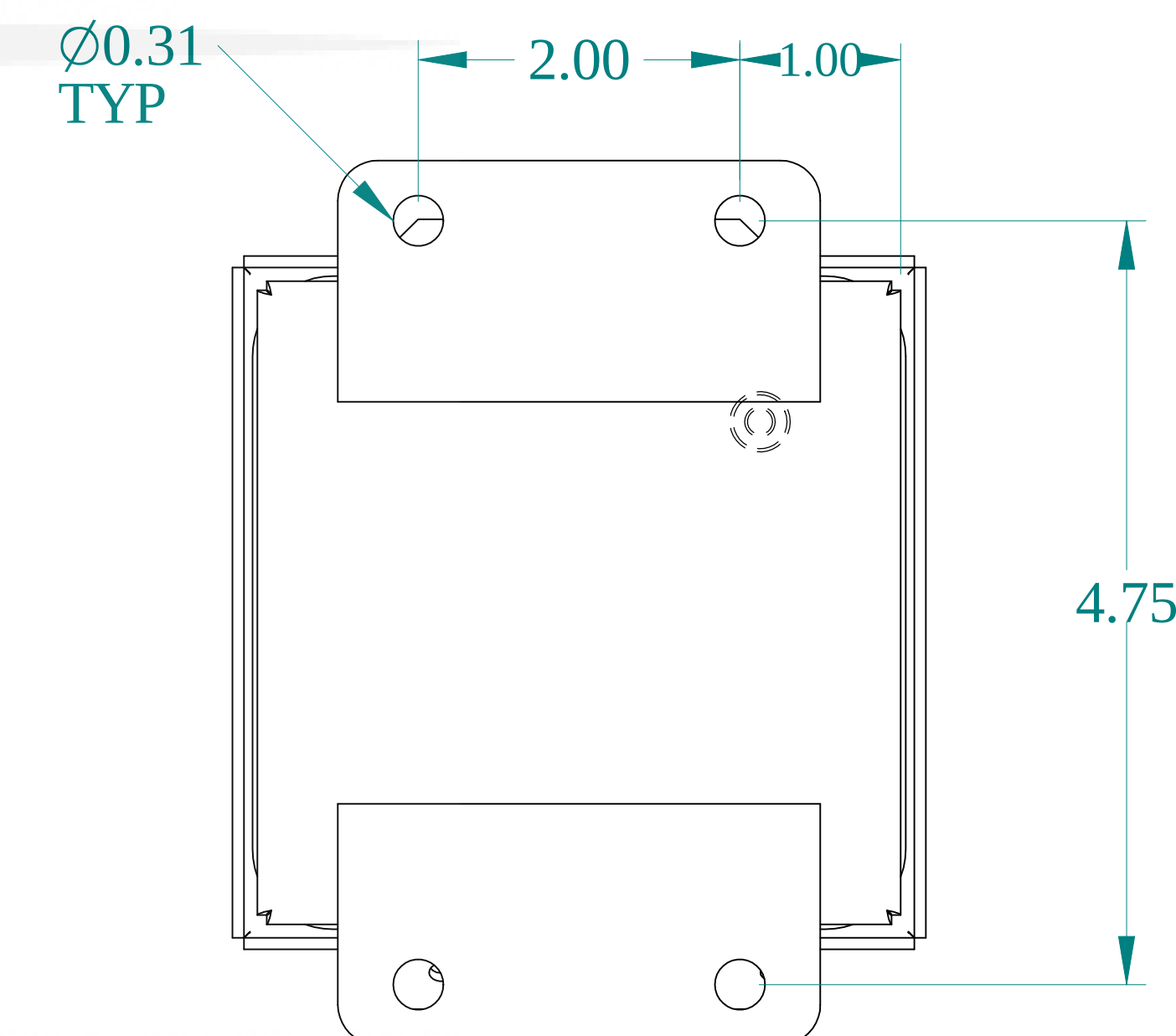
BACK VIEW
