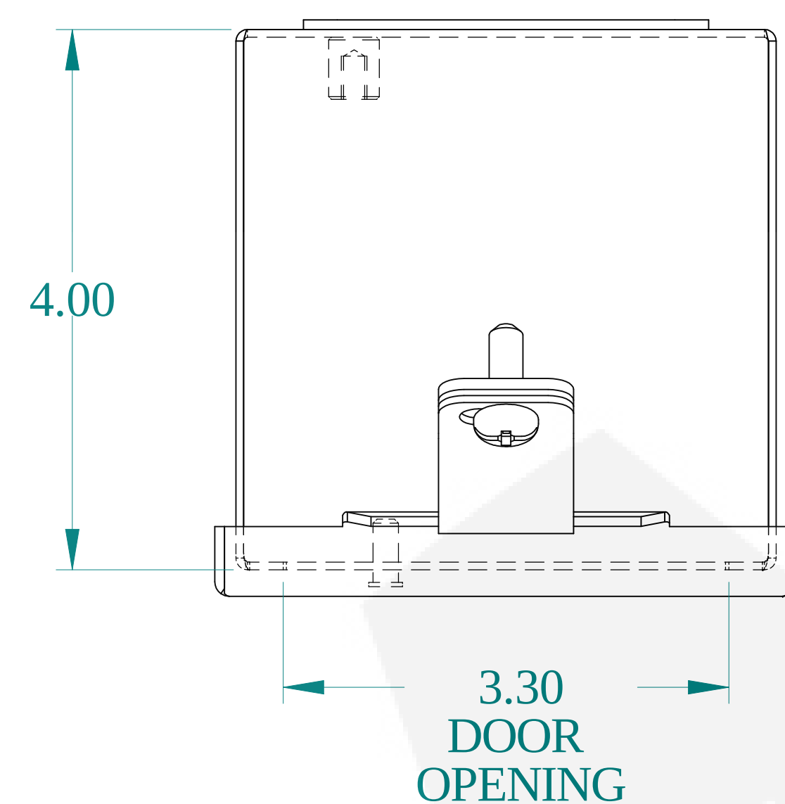
TOP VIEW
