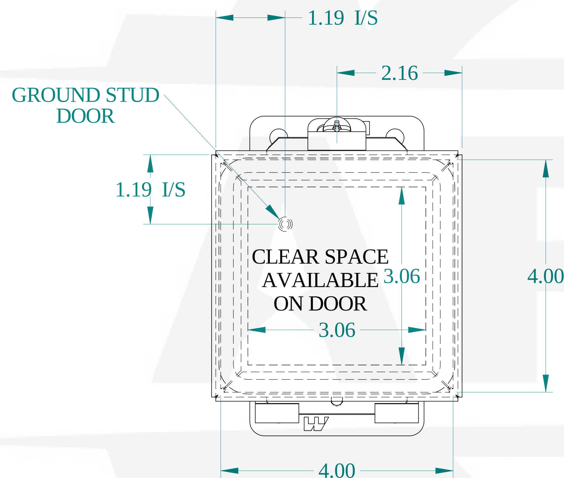
FRONT VIEW
