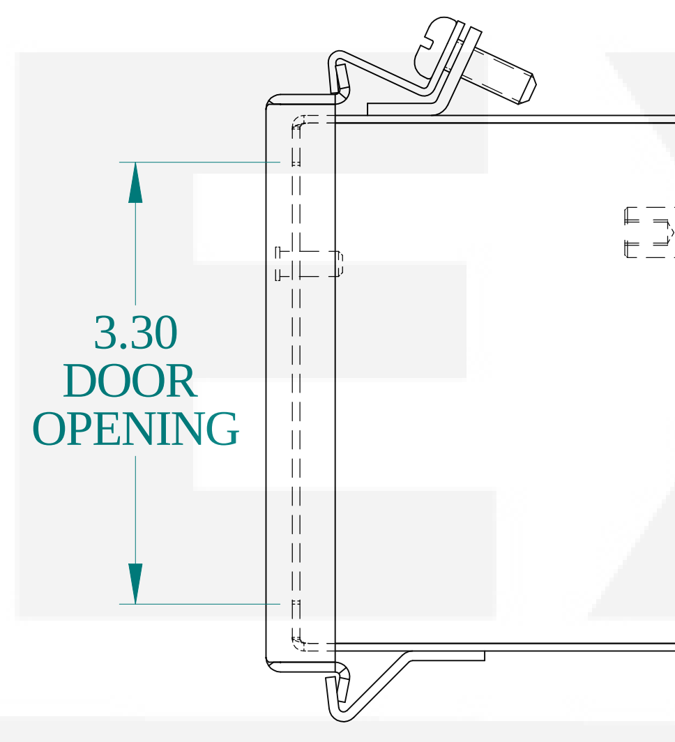
SIDE VIEW
