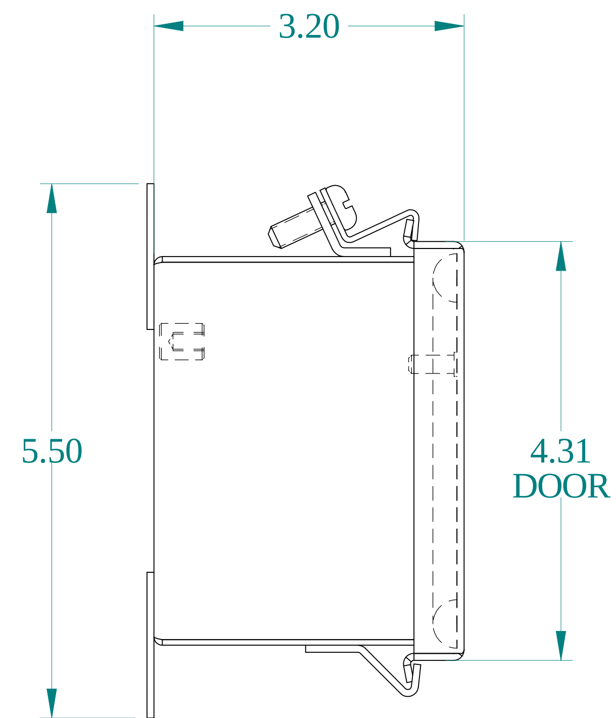
SIDE VIEW
