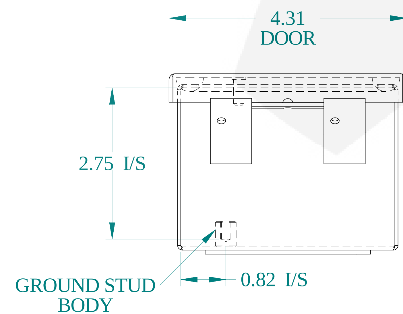
BOTTOM VIEW
