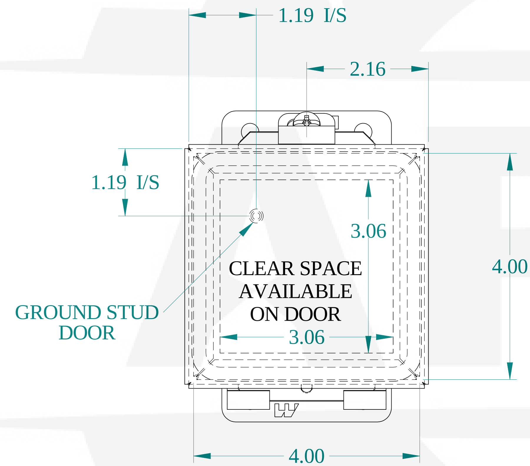
FRONT VIEW
