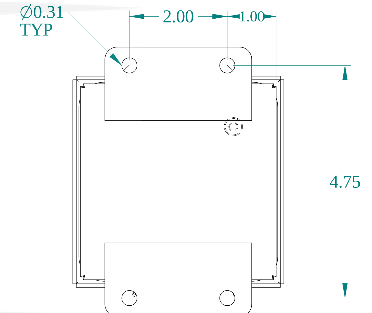
BACK VIEW
