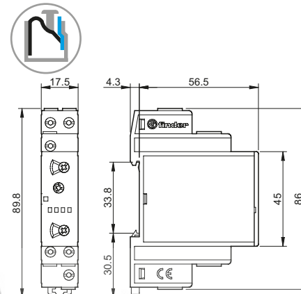
Type 80.41 Screw terminal
