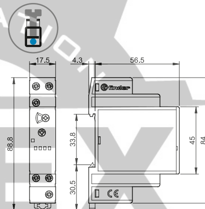
Type 80.71 Screw terminal
