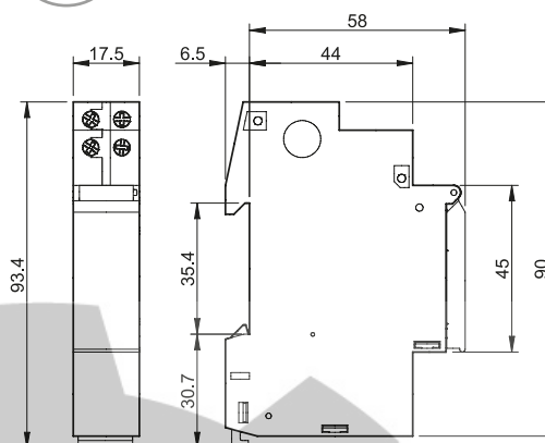
Types 12.51/12.81 Screw terminal
