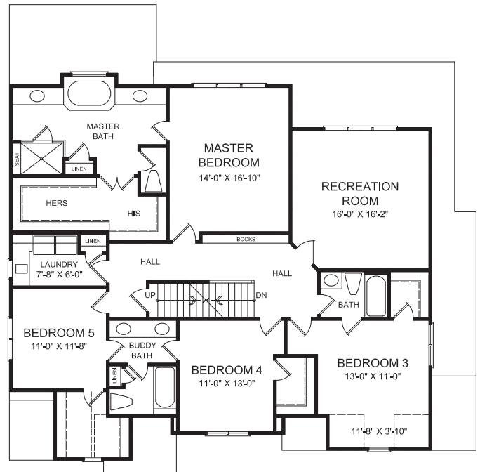
SECOND FLOOR
