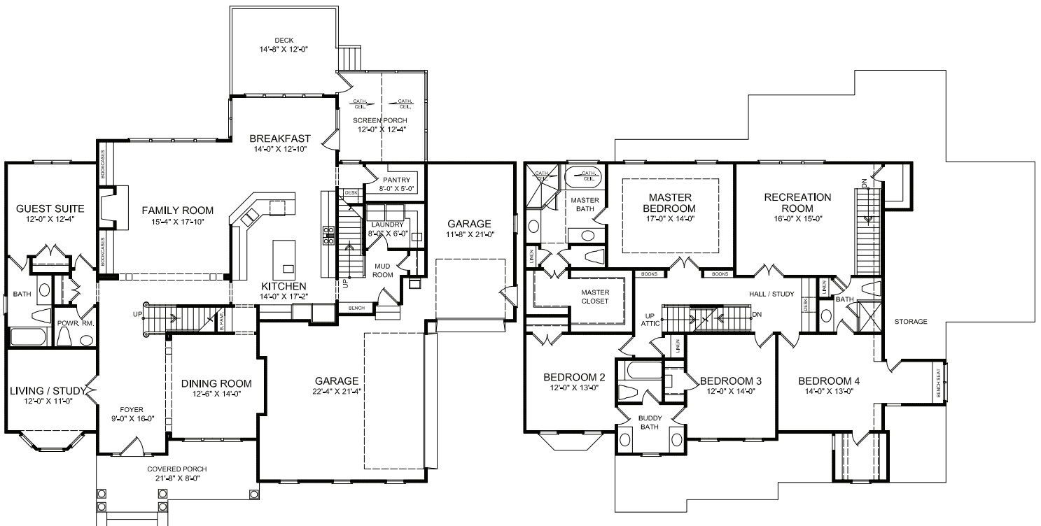
FIRST FLOOR
