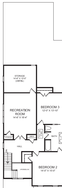
SECOND FLOOR
