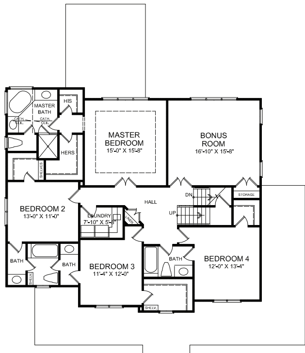
SECOND FLOOR
