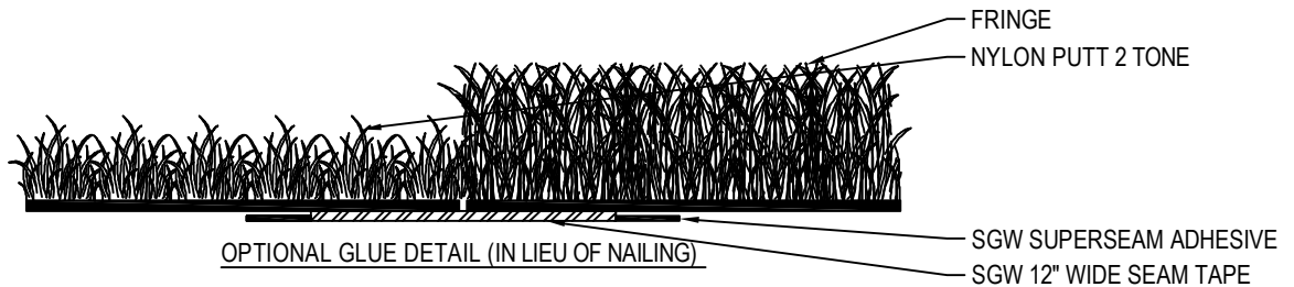
STANDARD INSTALL CROSS SECTION
