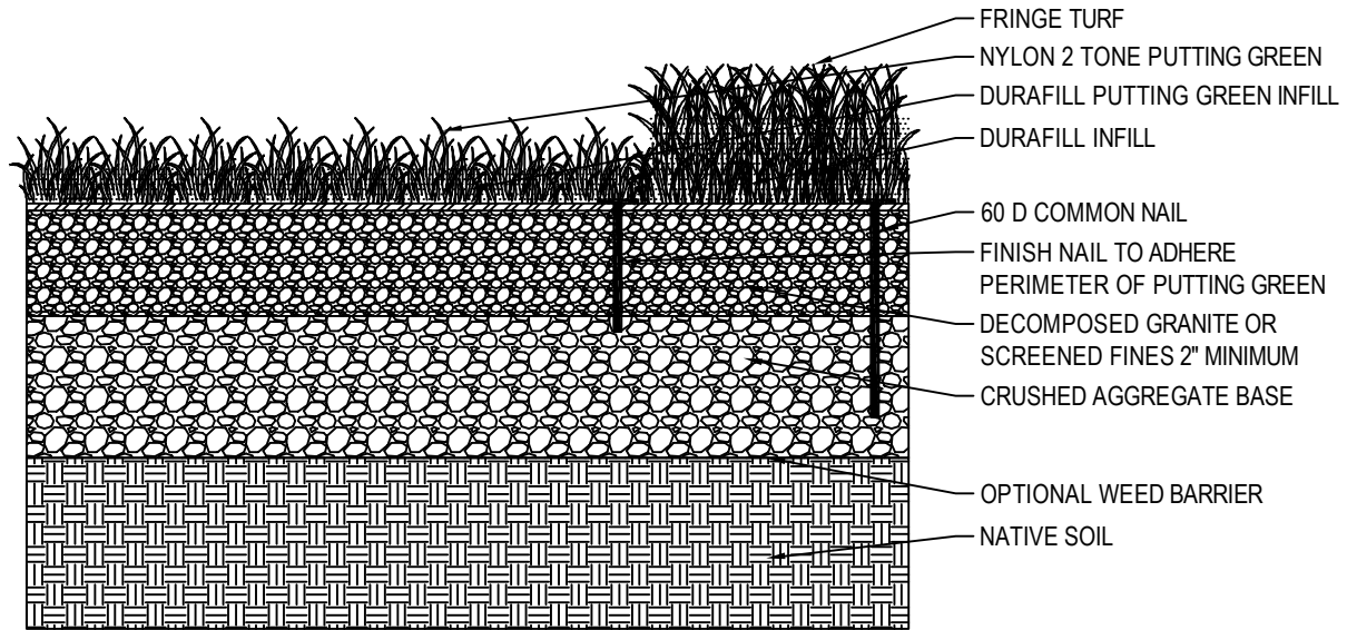
STANDARD INSTALL CROSS SECTION
