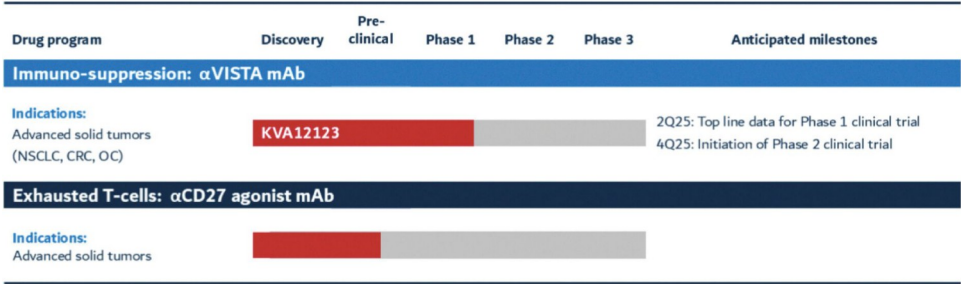
Figure 2. Kineta’s pipeline
