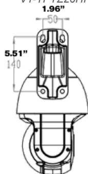
VT-TPT-WMT2 (Included) Wall Mount for VT-TPTZ20HRA-2A4
