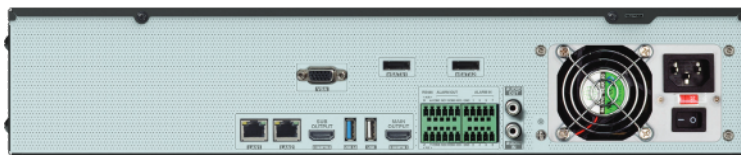
VT-TNR6480E1 Rear Connections
