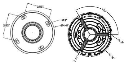
VT-TPDMT-A1 Transcendent Universal 10" Pendant Mount. Reqs. VT-TJB08
