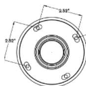
VT-TPDMT-A1 Transcendent Universal 10" Pendant Mount. Reqs. VT-TJB08
