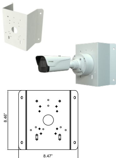
VT-TCNMT Transcendent Universal Corner Mount (reqs. VT-TJB08)
