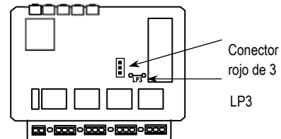
SK-910RAQ/RA-4Q PCB
