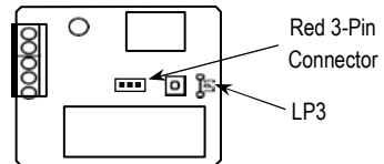
SK-910RAQ/RA-4Q PCB
