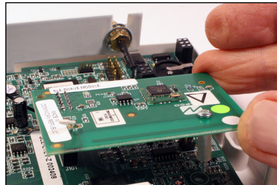
Fig. 5: Align and Insert the SLE-ZWAVE-MOD*
