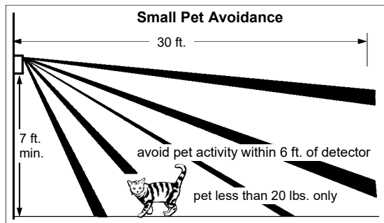
Side View: Standard Lens (LENS100) used for small pets
