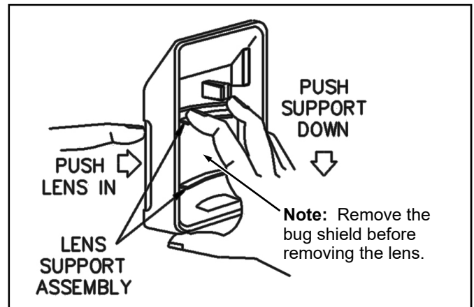
Replacing the lens
