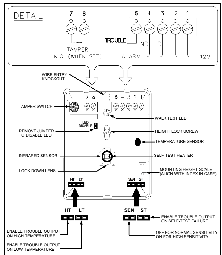
PIR1510 Circuit Board Detail
