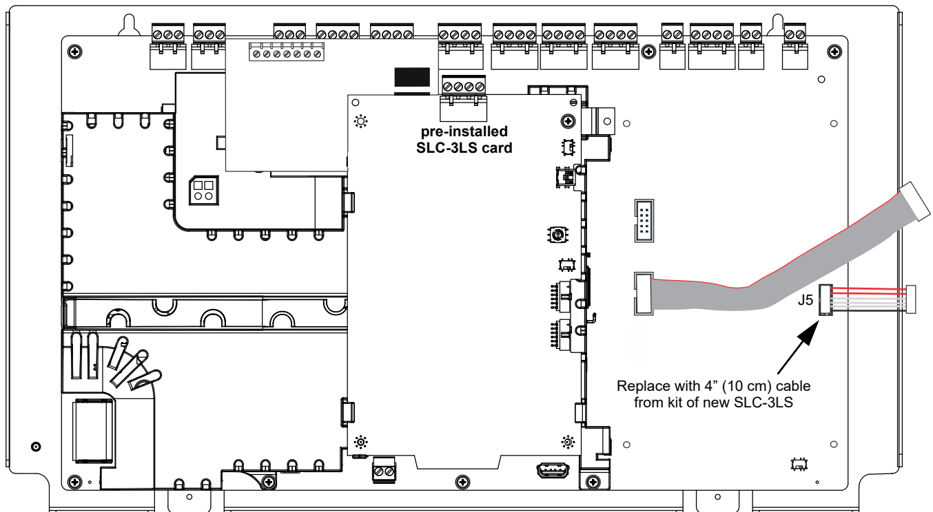
Figure 2 ES-1000X Assembly
